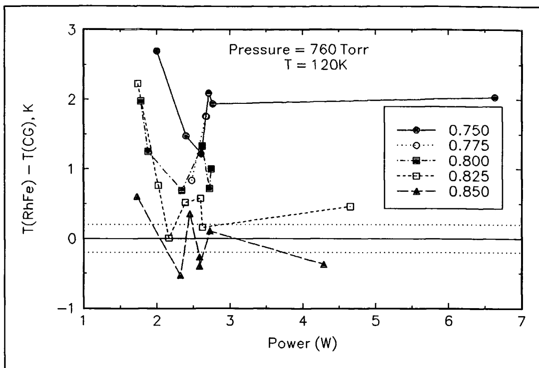
Figure 5.16 Temperature differences as a function of total heater power at fixed ratios of heater current.
