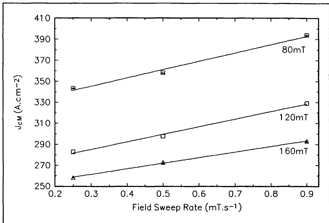
Figure 6.7 Dependence of J_{cM} values on magnetic field sweep rate for YBa_2Cu_3O_{7.8} single crystal F21 at 77K with B L.C.
