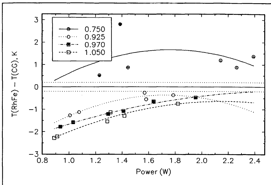
Figure 5.8 Temperature differences at 100K and 5 Torr as a function of heater power at fixed ratios of heater current. The lines are as a guide to the eye.
