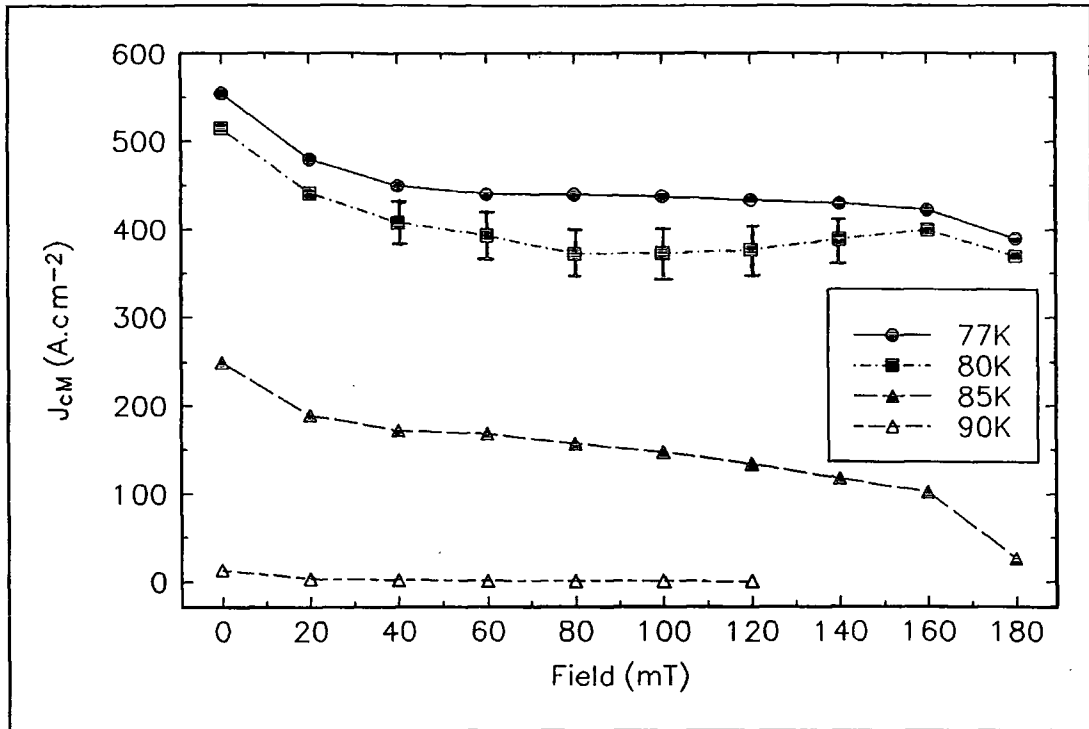
Figure 6.8 J_{cM} data for sample F21 from 77K to T_c with applied field parallel to the c-axis of the crystal.
