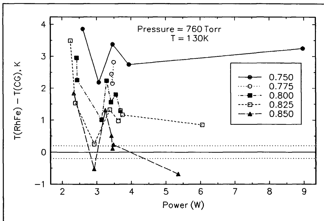
Figure 17 Temperature differences as a function of total heater power at fixed ratios of heater currents.
