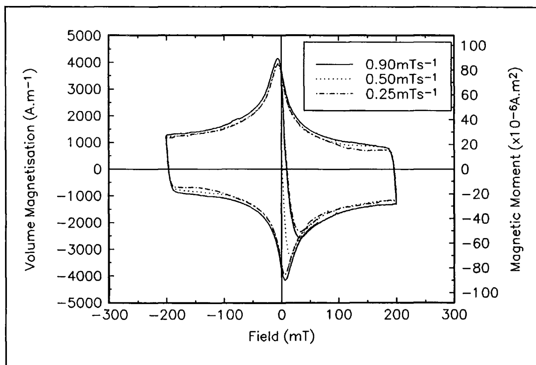
Figure 6.2 Effects of field sweep rate on hysteresis loops at 77K. Sample is YBa 2 Cu 3 O 7.6 single crystal F21 with B || c.
