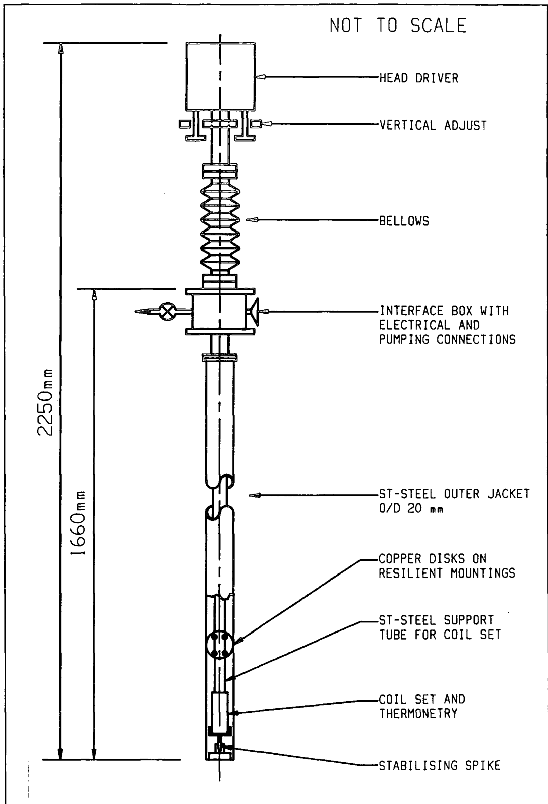
Figure 4.4 Overall view of the Vibrating Sample Magnetometer Probe.
