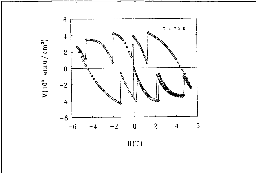
Figure A.1 Flux Jumping in a bulk sample of \text{YBa}_2\text{Cu}_3\text{O}_{7.6} [3].
