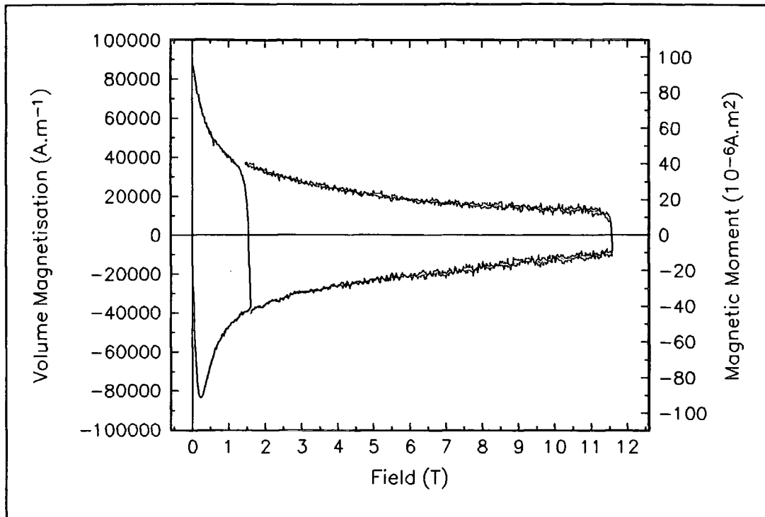
Figure 7.6 Magnetic hysteresis of a 19 filament \text{Bi}_2\text{Sr}_2\text{Ca}_2\text{Cu}_3\text{O}_x wire at 4.2K.
