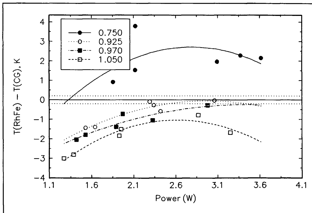
Figure 5.9 Temperature differences at 110K and 5 Torr as a function of heater power at fixed ratios of heater current. The lines are as guides to the eye.
