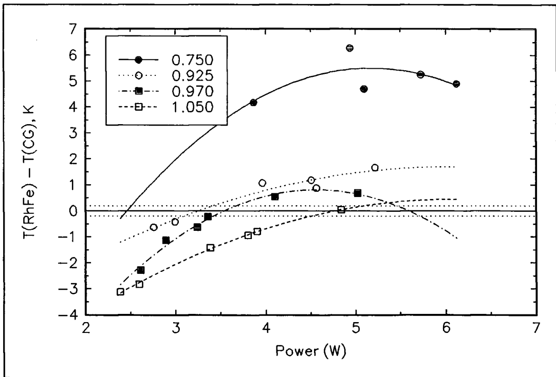
Figure 5.11 Temperature differences at 130K as a function of heater power at fixed ratios of heater currents. The lines are guides to the eye.
