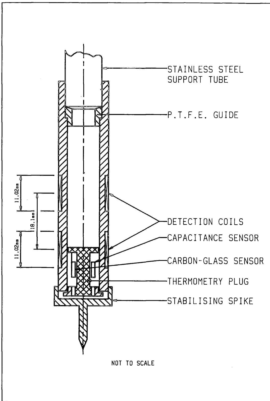
Figure 4.5 Detailed View of the coil set of the Vibrating Sample Magnetometer probe. Positions of the two thermometers and the stabilising spike are also shown.
