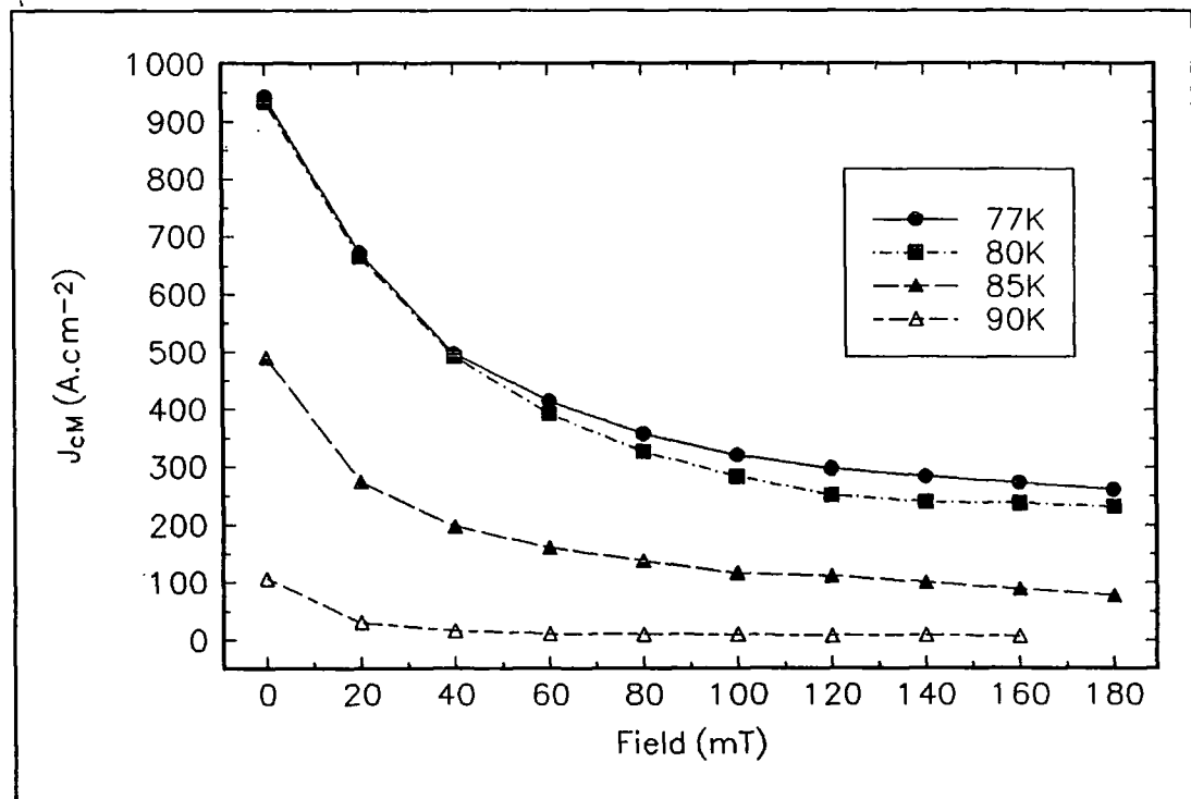
Figure 6.9 J_{cM} for sample F21 from 77K to T_c with applied field perpendicular to the c-axis of the crystal.
