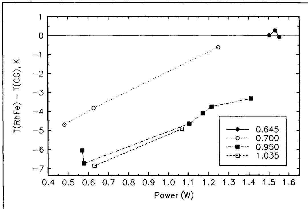
Figure 5.28 Temperature differences at 40K, 50mTorr as a function of heater power at fixed ratios of heater current.
