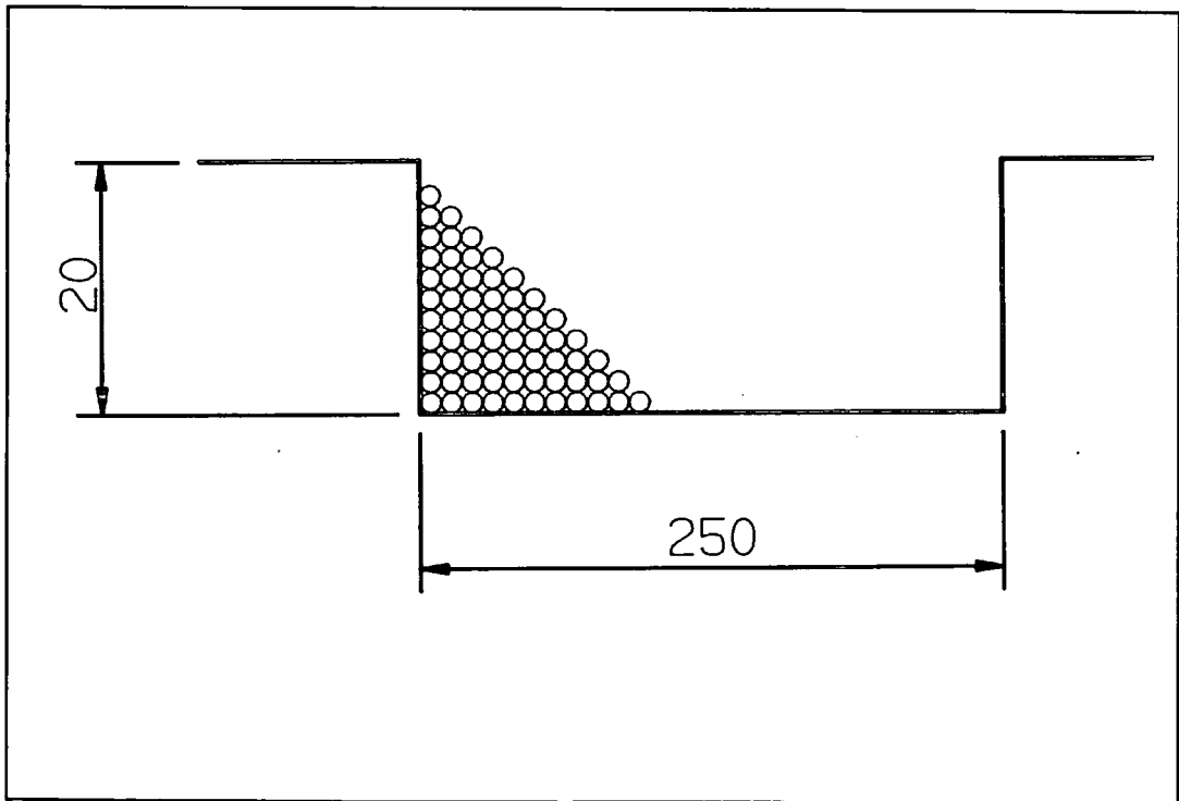
Figure 4.7 Basis of the model used to calculate the induced voltage in the coils.
