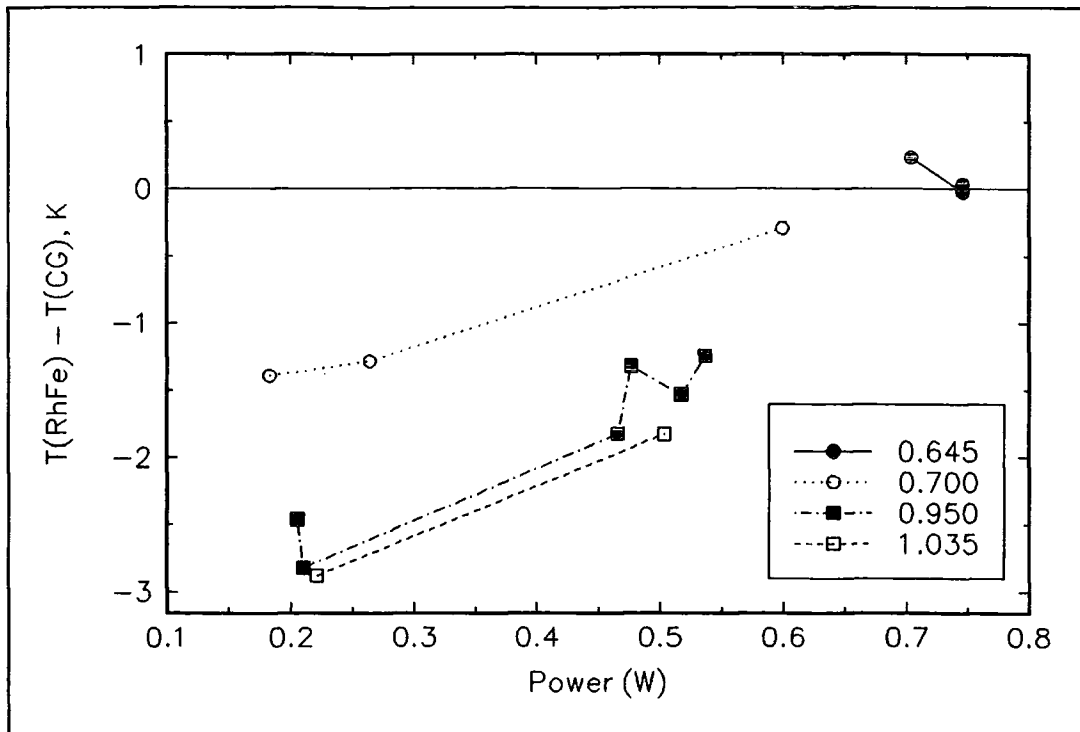
Figure 5.27 Temperature differences at 20K, 50mTorr as a function of heater power at fixed ratios of heater current.
