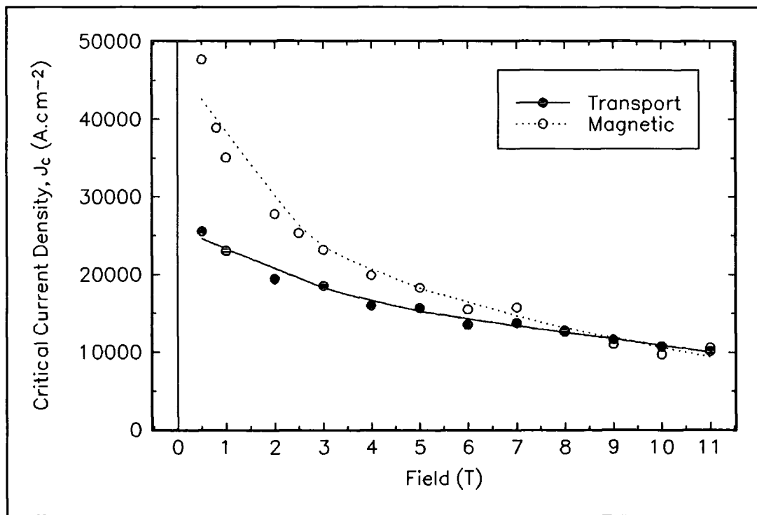
Figure 7.7 Comparison of transport and magnetisation critical current densities for a 19 filament \text{Bi}_2\text{Sr}_2\text{Ca}_2\text{Cu}_3\text{O}_x wire at 4.2K.
