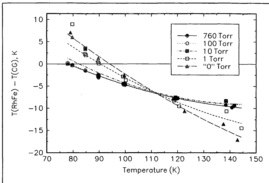
Figure 5.3 Temperature differences as a function of the pressure of helium transfer gas in the probe.
