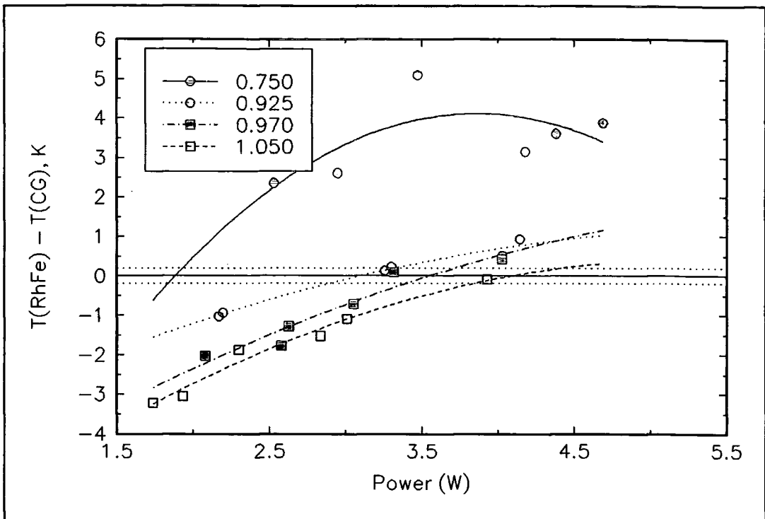
Figure 5.10 Temperature differences at 120K and 5 Torr as a function of heater power at fixed ratios of heater currents. The lines are guides to the eye.
