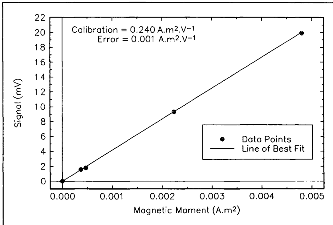
Figure 4.15 Calibration of VSM signal using the saturation magnetic moment of several nickel samples.
