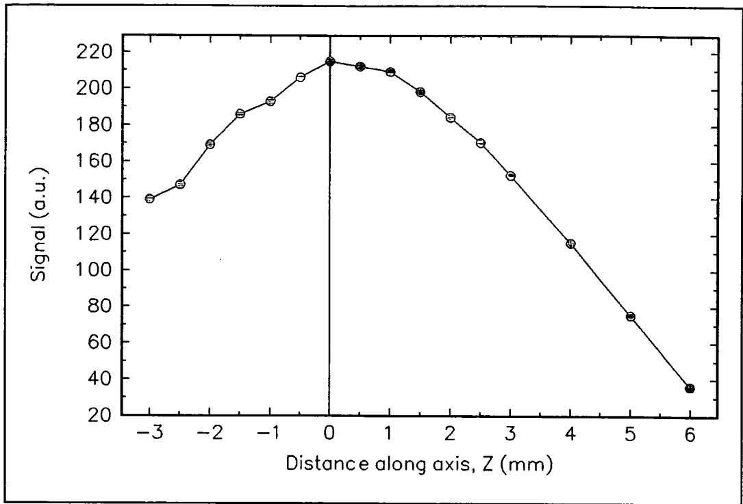
Figure 4.6 Experimental coil pick-up profile for the 12.1mm centre-centre separation.
