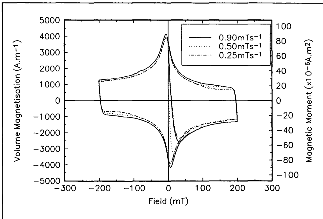
Figure 6.2 Effects of field sweep rate on hysteresis loops at 77K. Sample is YBa 2 Cu 3 O 7-δ single crystal F21 with B || c.
