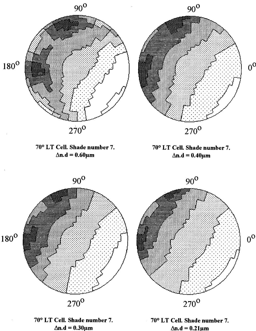
Figure 5.21: Optical angular properties of 70^\circ LT cells as a function of the \Delta n.d value. The cells are in the “Symmetric A” polariser configuration and a standard I.F is present. Shade number 7.
