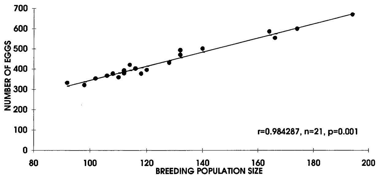
REGRESSION OF NO.EGGS AGAINST NO.BREEDING POPULATION
