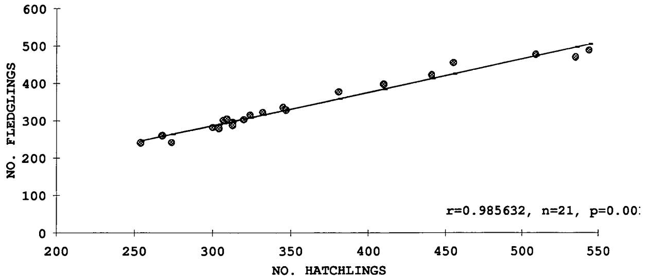
REGRESSION OF THE NUMBER OF FLEDGLINGS AGAINST THE NUMBER OF HATCHLINGS
