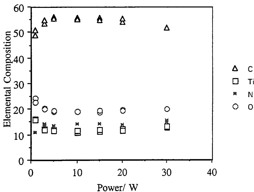
Fig. 1 Elemental percentages as a variation of glow discharge power (3 min, 19 cm): (a) TMT; and (b) TMT/H 2 .
