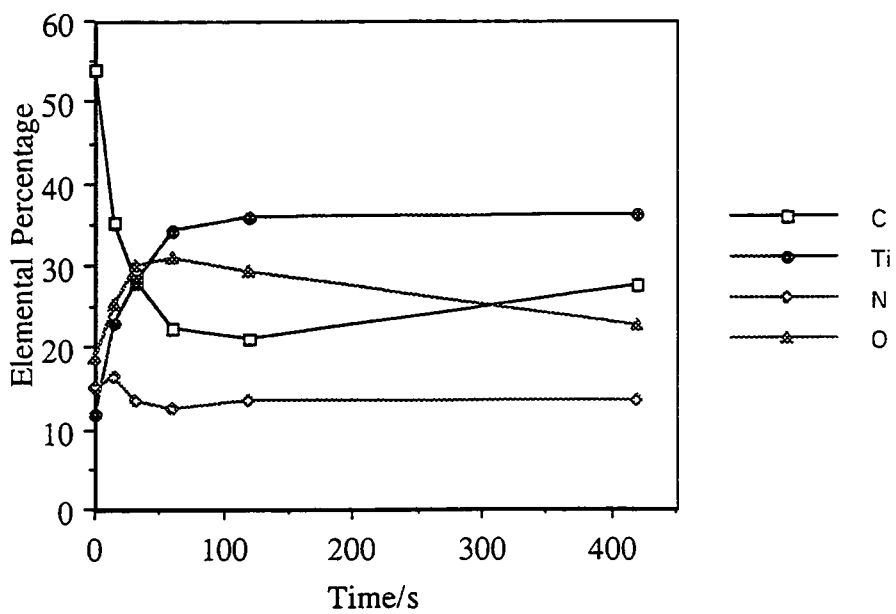
Fig. 4 XPS depth profile for PACVD films onto a glass substrate (15 W, 3 min, 19 cm): (a) TMT; and (b) TMT/H 2 .
