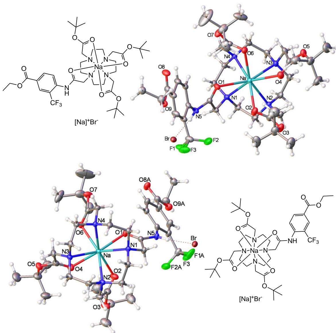
Fig. 3.15 Crystal structure of the trisubstituted para -ethyl ligand 4 , containing an octadentate \text{Na}^+ ion with bromide as the counter ion, hydrogen-bonded to the amide proton. The two structures are the same molecule seen from above and below (for crystallographic details see appendix B).
