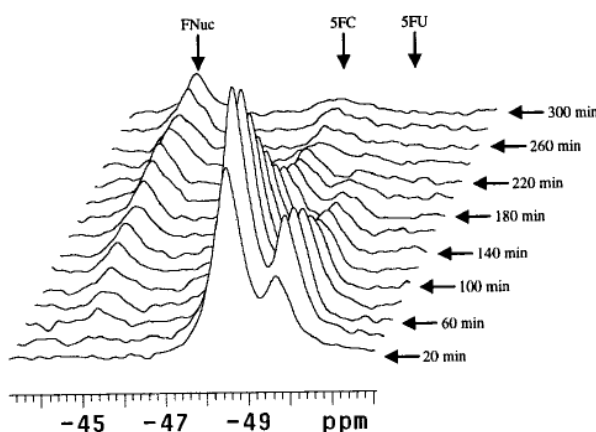
Fig. 1.4 ^{19}\text{F} NMR spectra over time monitoring the changes of 5-FC in a subcutaneous tumour expressing yeast CD. Start 20 min after i.p. administration of 1g/kg 5-FC. 20-min interval for each spectrum (Figure taken from reference 32 ).
