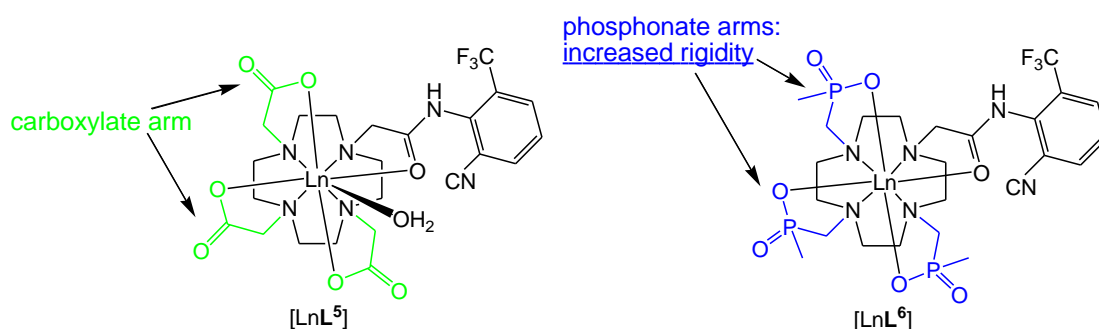
Fig. 2.21 DO3A monoamide complex [ LnL 5 ] vs DOTP monoamide complex [ LnL 6 ].
