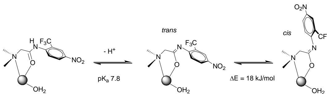
Scheme 2.6 Acid-base equilibrium between the protonated and non-protonated form in [LaL^2] showing the conformational exchange between cis/trans amide forms in the deprotonated species.
