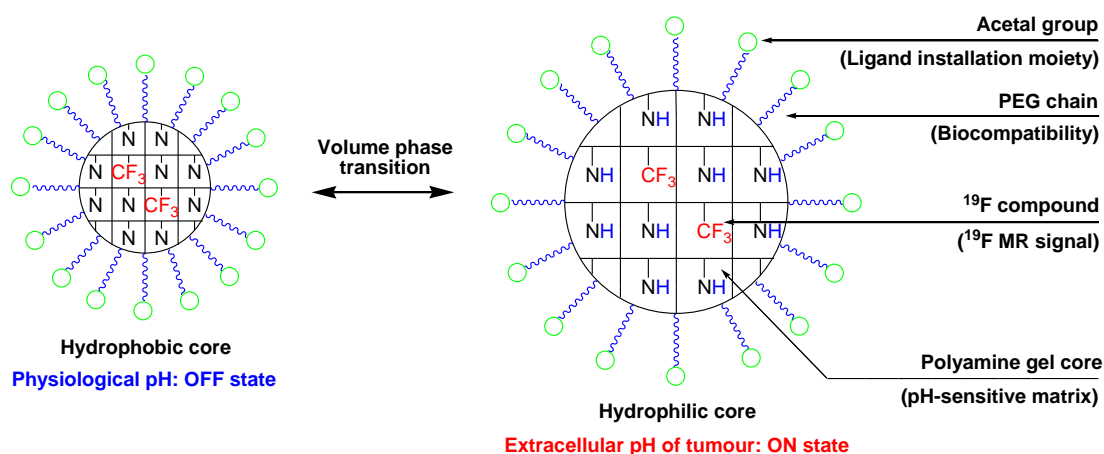
Fig. 1.5 Schematic representation of the pH sensitive PEGylated nanogels.
