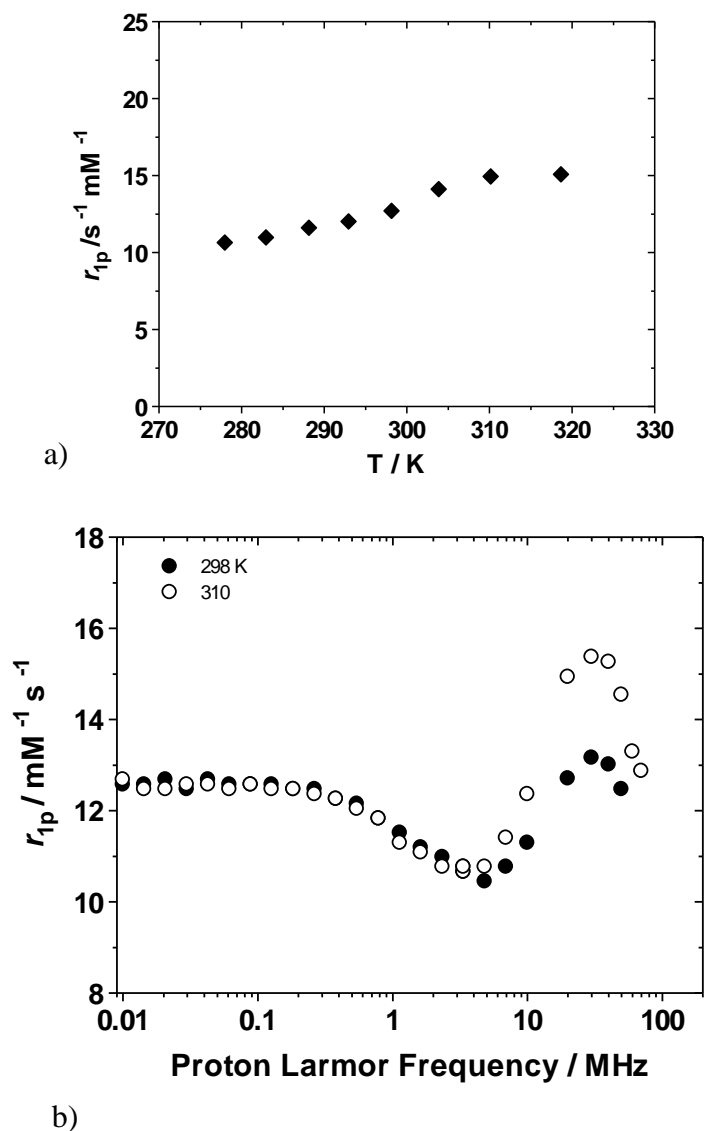
Fig. 5.3 Proton relaxivity studies for the Gd-conjugate 75 . a) relaxivity vs temperature profile measured at 20 MHz. b) 1/T_1 NMRD profiles at 298 (filled circles) and 310 K (open circles).
