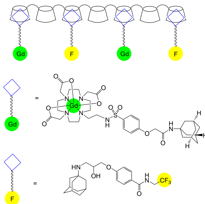
Fig. 1.8 Schematic representation of the poly-β-cyclodextrin pH probe.
