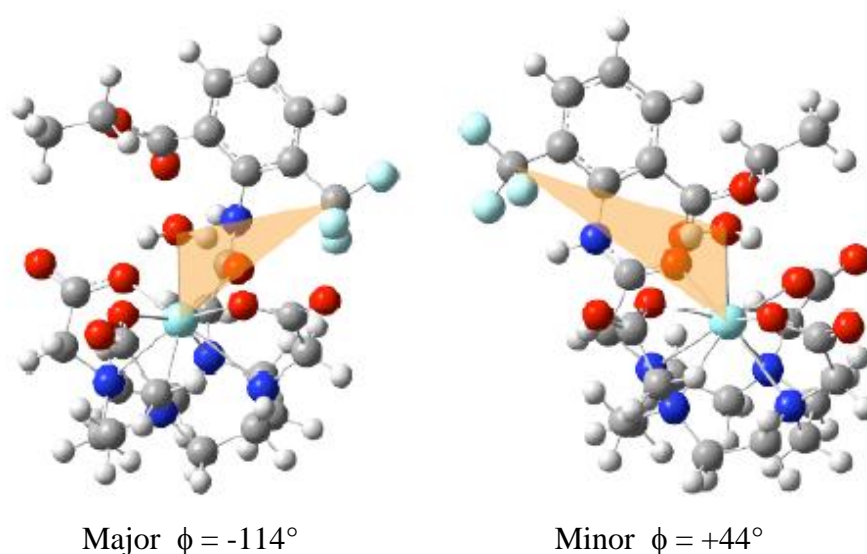
Fig. 3.7 DFT calculated structures showing the two low-energy isomers of [\text{LnL}^{4a}] associated with the rotation of the phenyl ring around the C-N bond.
