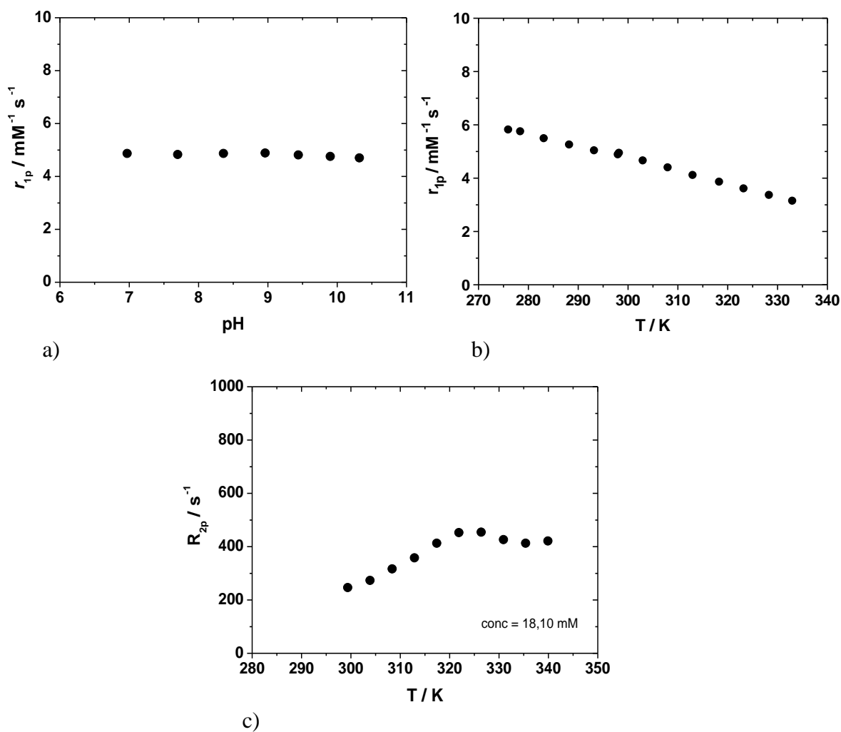
Fig. 3.17 Relaxivity studies for [\text{GdL}^{4b}] a) Relaxivity as function of pH. b) Relaxivity as a function of temperature. c) Variable temperature ^{17}\text{O} NMR R_{2p} .
