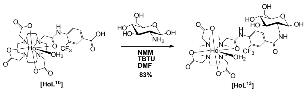
Scheme 2.4 Synthesis of [ HoL^{13} ].
