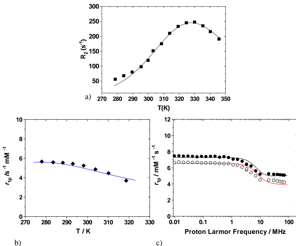
Fig. 5.2 [GdL 1b ] proton relaxivity studies showing the fit (line) to the measured data. a) 17 O R_2 vs temperature profile measured at 11.7 T (500 MHz). b) relaxivity vs temperature profile measured at 20 MHz and pH 7.2. c) 1/T_1 NMRD profiles at 298 (filled circles) and 310 K (open circles).
