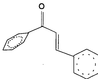
transoid conformation
