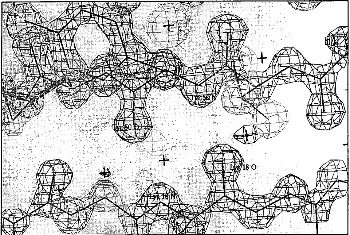
Figure 7. Intermolecular H-bonding.
