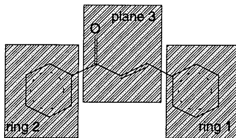
Figure 1, Molecular conformation
