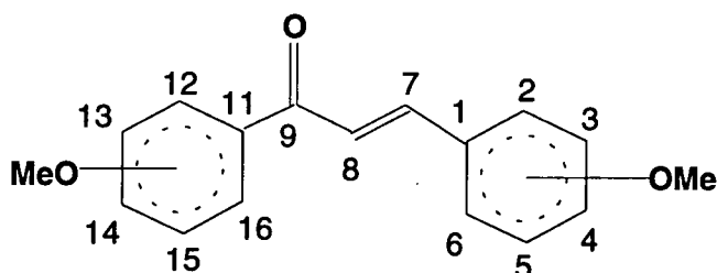
Numbering scheme for substitution positions on the chalcone molecule
