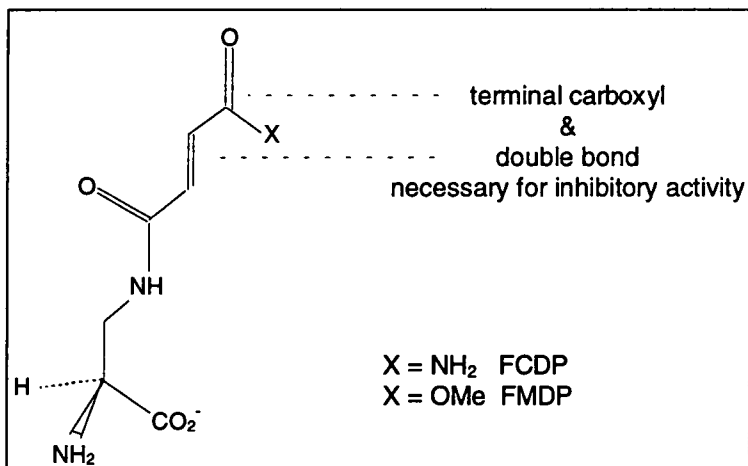
Figure 2. Possible mechanisms proposed for formation of Cys1 - FMDP complex
