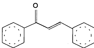
cisoid conformation
