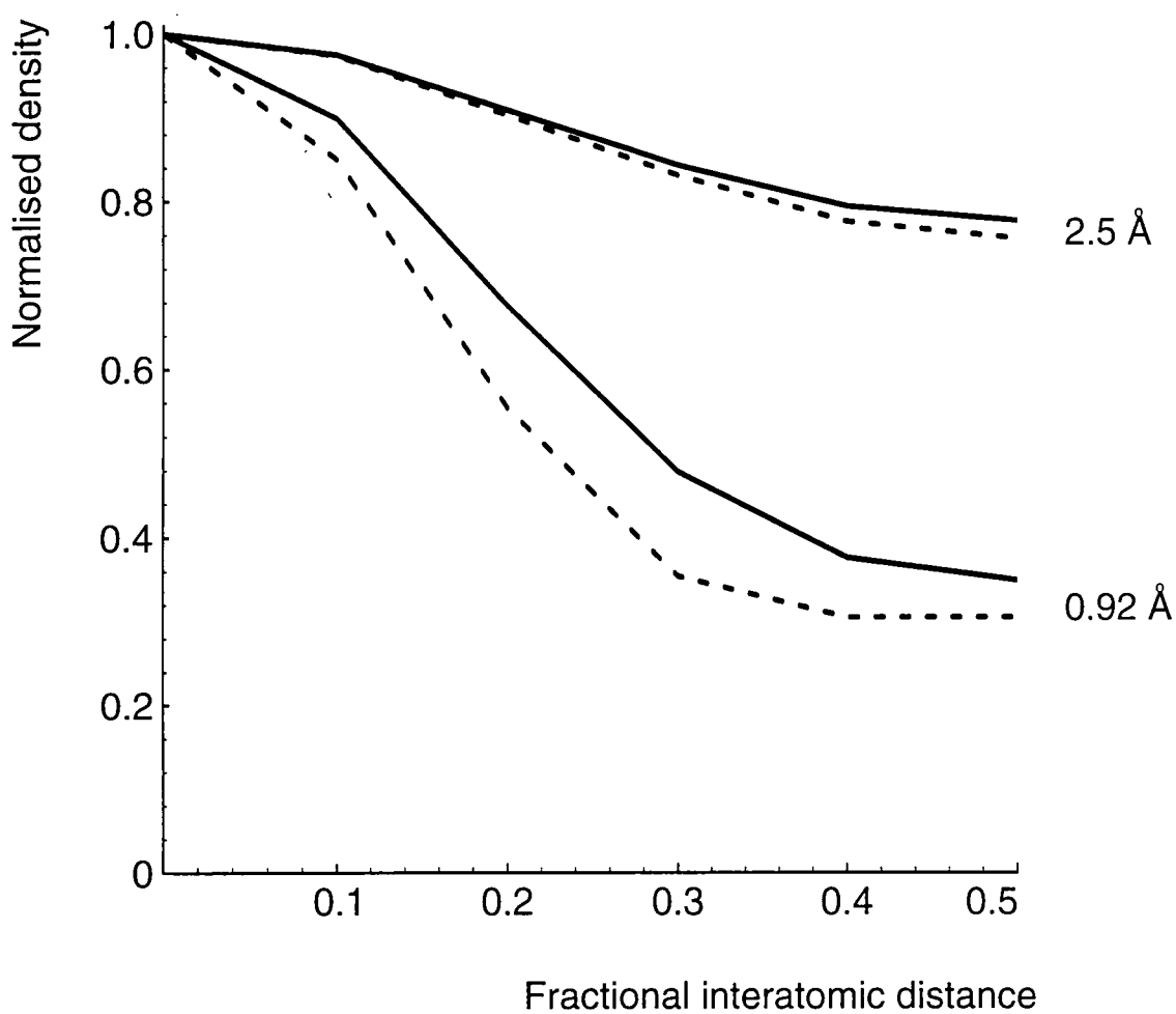
Figure 5a. The resolvability of solvent atoms.
