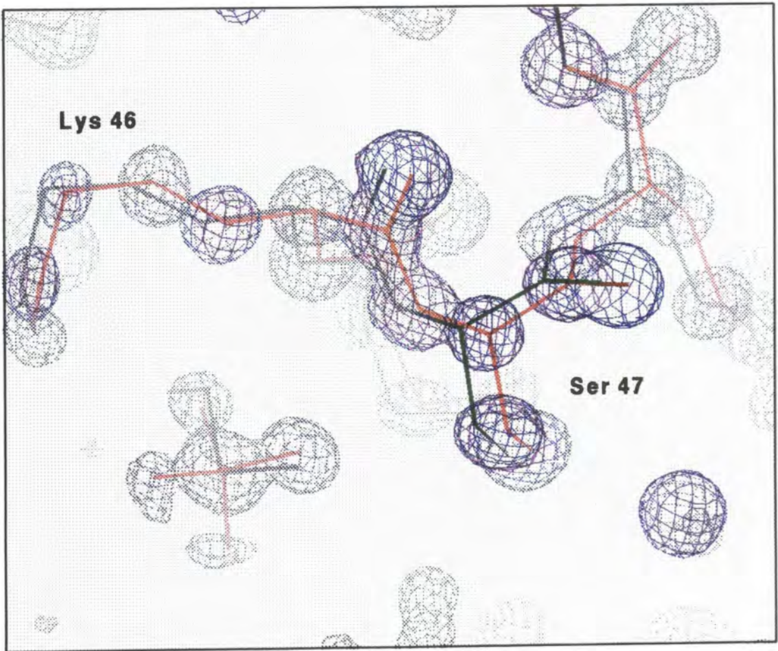
Figure 6. The sulphate binding site. The major chain conformation and sulphate are shown in red, the minor chain conformation, in green. The (3F_o - 2F_c) electron density is plotted. Using QUANTA.
