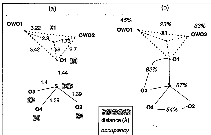
Figure 2, stages in modelling of the disordered sulphate ion
