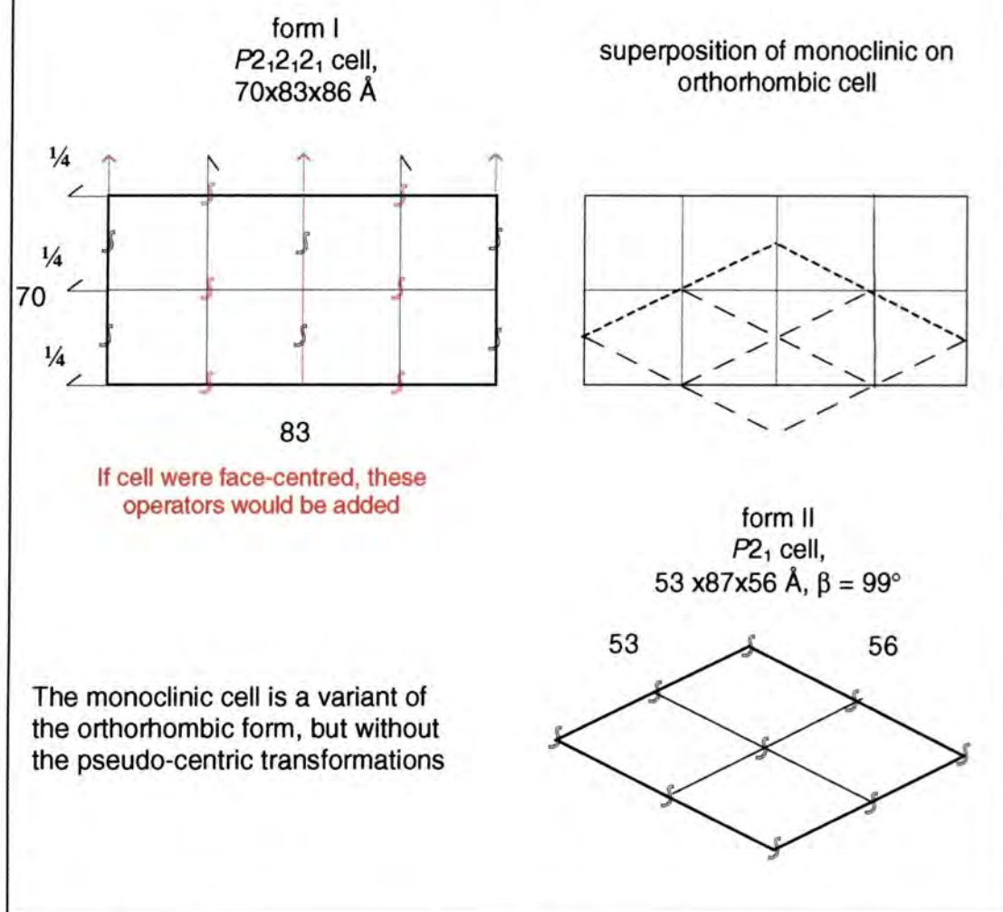
Figure 6. Relationship between GAT domain crystal forms I and II
