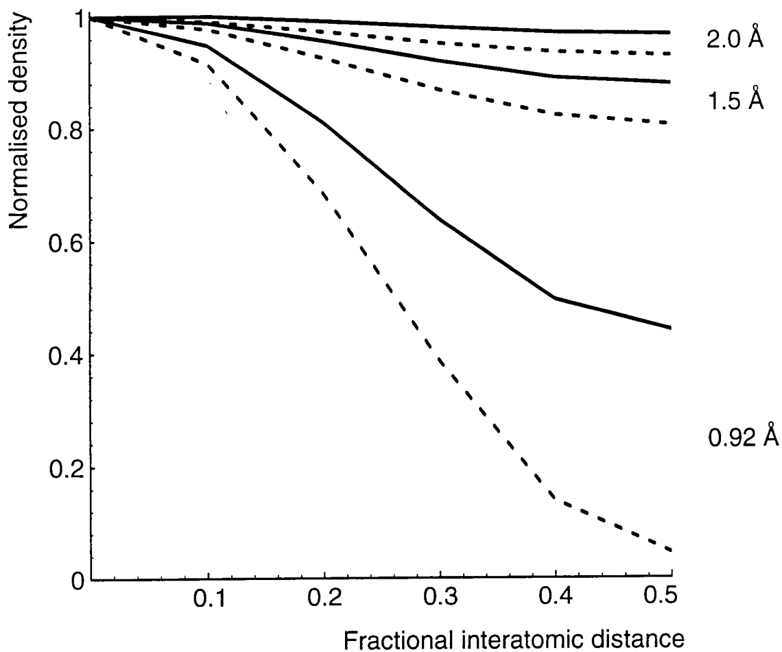
Figure 2. Average shape of the density between neighbouring atoms. Maps of rubredoxin using data of different sharpness and resolution were investigated. The normalised density values are plotted against fractional distance from the atomic centre, for E-maps (dashed line) and F-maps (continuous line) for maps with 0.92, 1.5 and 2.0 Angstrom high resolution data cutoffs applied.
