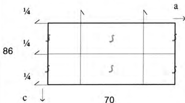
Figure 7. Relationship between monoclinic and orthorhombic symmetries of form I, and between the 4 independent molecules in the monoclinic cell
