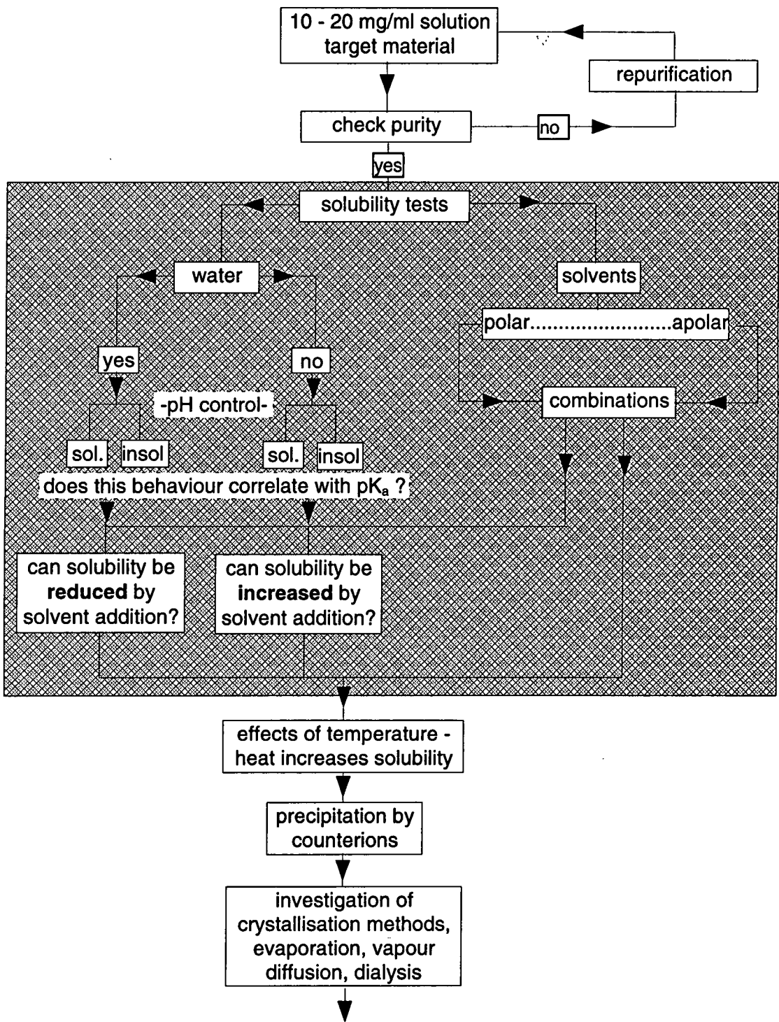
Figure 3. The search for crystallisation conditions for a peptide of medium length
