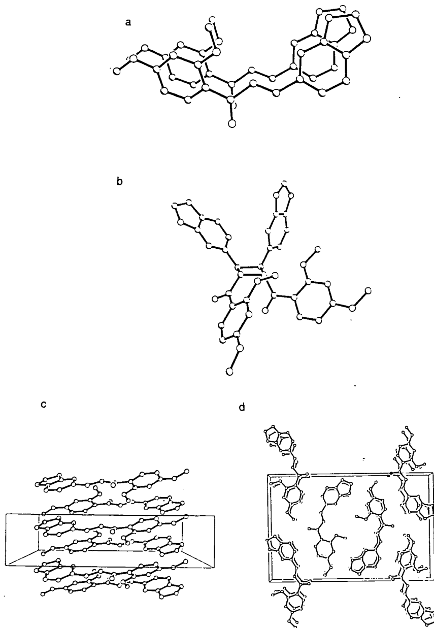
Figure 9. The chalcone XXII monomer and dimer structures
