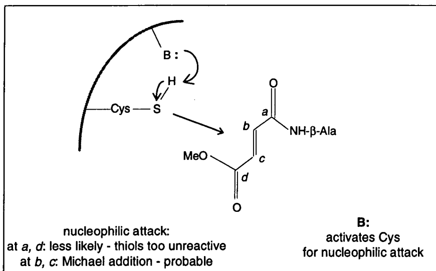
Figure 2. Possible mechanisms proposed for formation of Cys1 - FMDP complex
