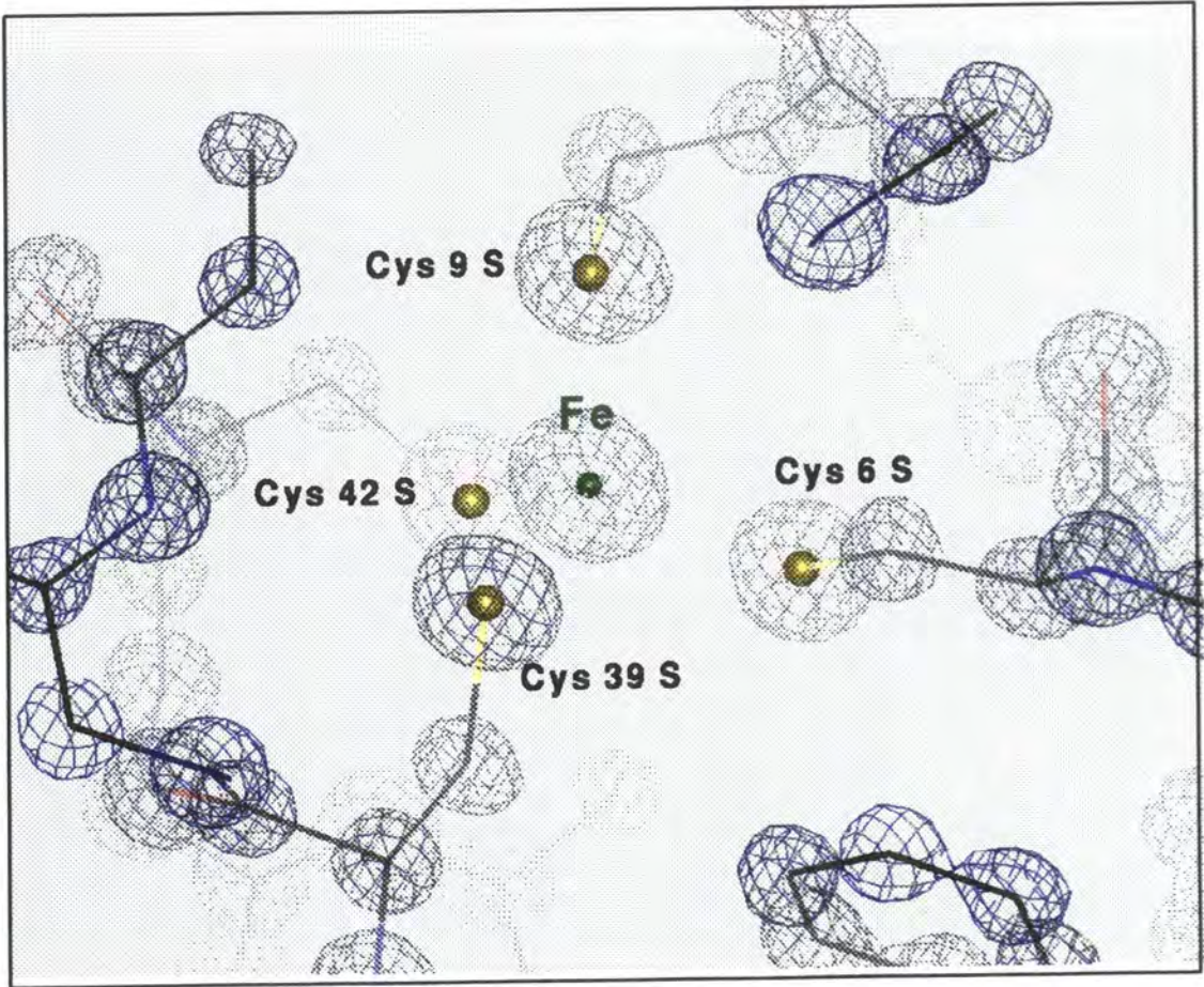
Figure 5. The Fe(Cys)4 cluster. 3Fo - 2Fc density.
