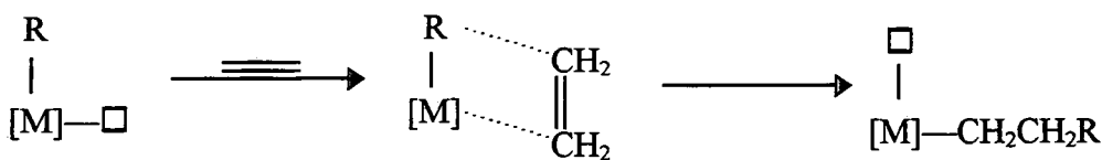
Scheme 1: The Cossee mechanism
