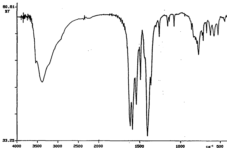
Figure 4.2 IR spectrum of zinc/copper basic trimellitate, (\text{Zn}_x\text{Cu}_{1-x})_{2.5}(\text{OH})_2\text{TM} \cdot 2\text{H}_2\text{O} (for the spectrum shown x=0.9 , y=1 ).
