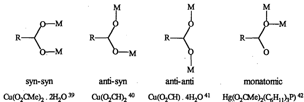
Figure 2.3 Carboxylate bridges.
