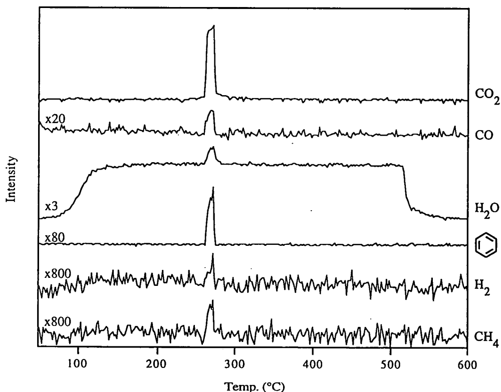
Figure 6.20 TPDec profile of \text{Cu}_2\text{PM} \cdot 6\text{H}_2\text{O} under oxygen.
