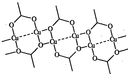
Figure 2.6 Polymeric structure of copper(I) acetate.
