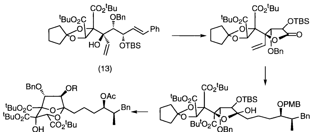
Scheme 1.5.2a
