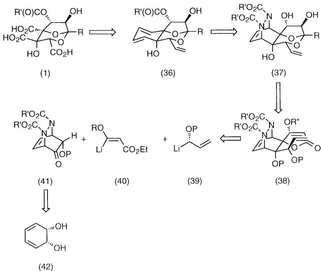
Scheme 1.6.1
