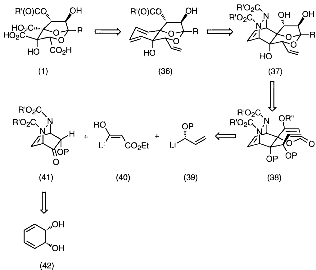
Scheme 1.6.1
