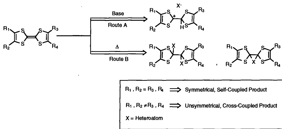
Scheme 1.3.1 Synthesis of Tetrathiafulvalene Derivatives
