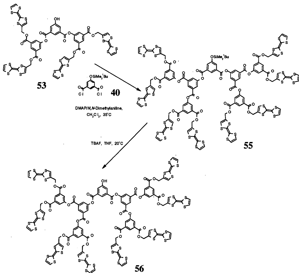
Scheme 2.3.8 Synthetic Pathway to Third Generation Dendron Wedge 56
