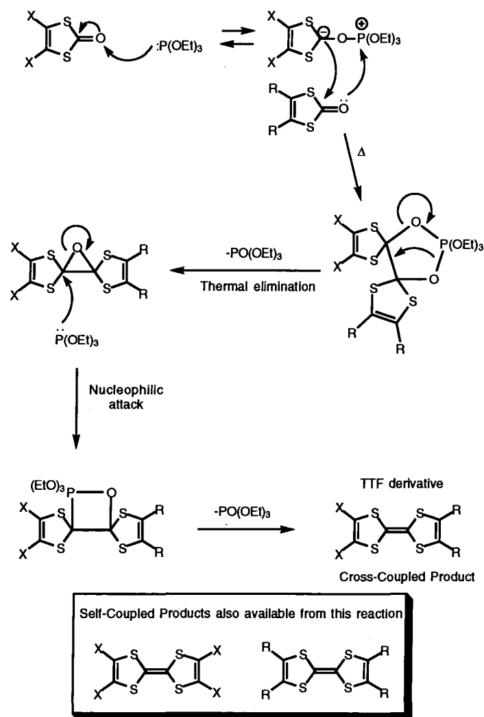
Scheme 1.3.2 Mechanism for Synthesis of Tetrathiafulvalene Derivatives via Phosphite-Induced Coupling
