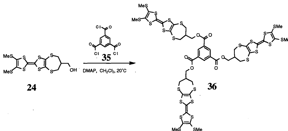
Scheme 2.3.1 Reaction to Produce Model Compound 36
