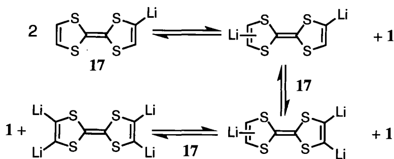
Scheme 1.3.4 Multi-Lithiated Species Formed by the Action of LDA on Tetrathiafulvalene
