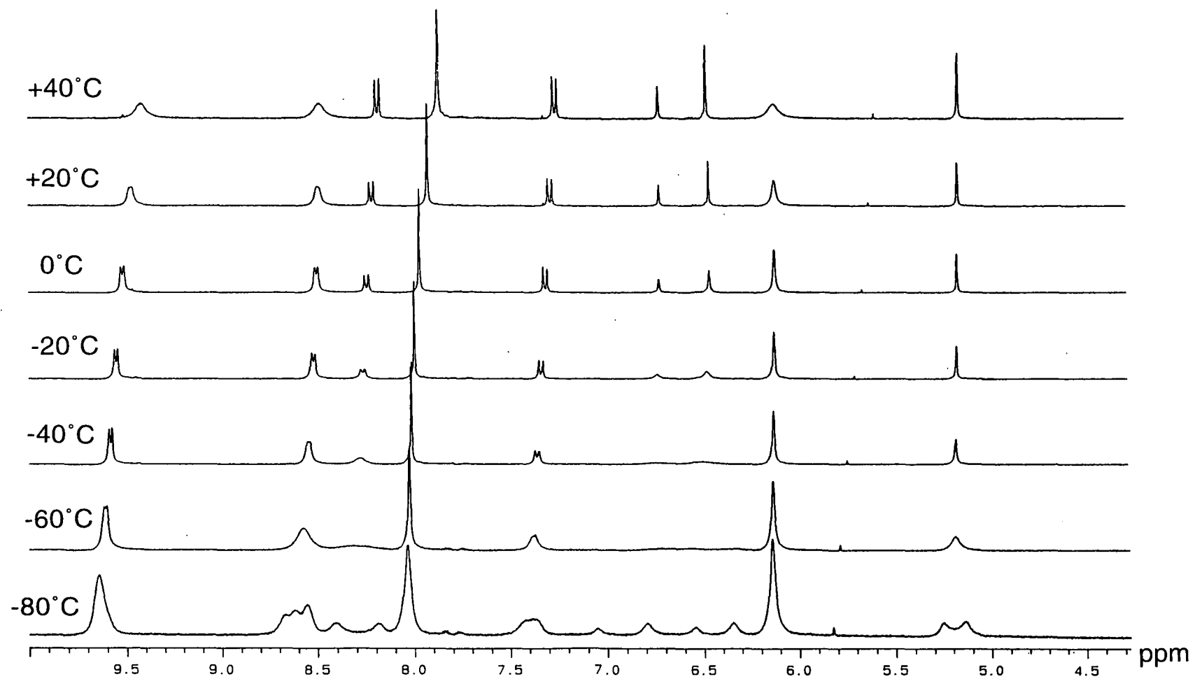
Figure 4.2.1 Variable Temperature 1 H NMR Spectra of [2]Pseudorotaxane 76 from +40°C to -80°C
