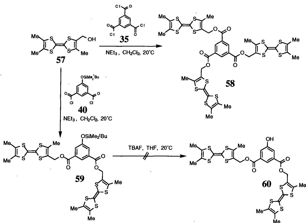
Scheme 2.3.9 Attempted Synthesis of Dendron Wedge 60
