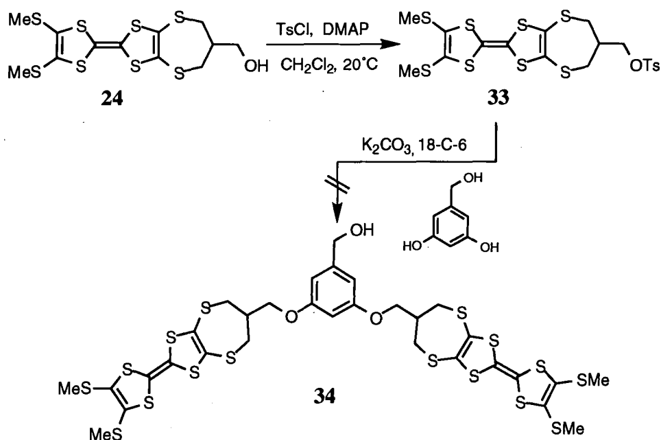
Scheme 2.2.2 Attempted Reaction of Tosylate 33 with 3,5-dihydroxybenzyl alcohol
