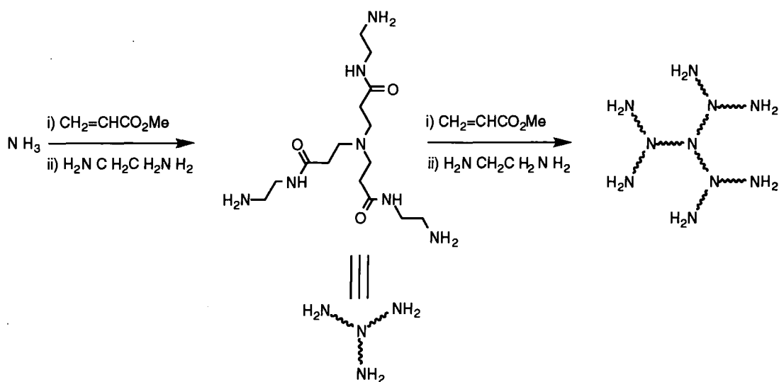
Scheme 1.2.1 A Schematic Representation of the Assembly of PAMAM Dendrimers 7a
