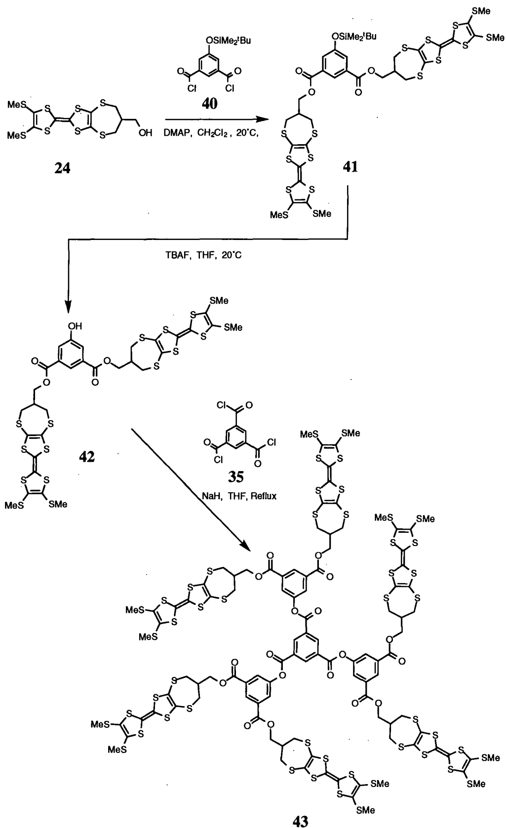
Scheme 2.3.3 Reaction Pathway to Assemble Second Generation Dendrimer 43
