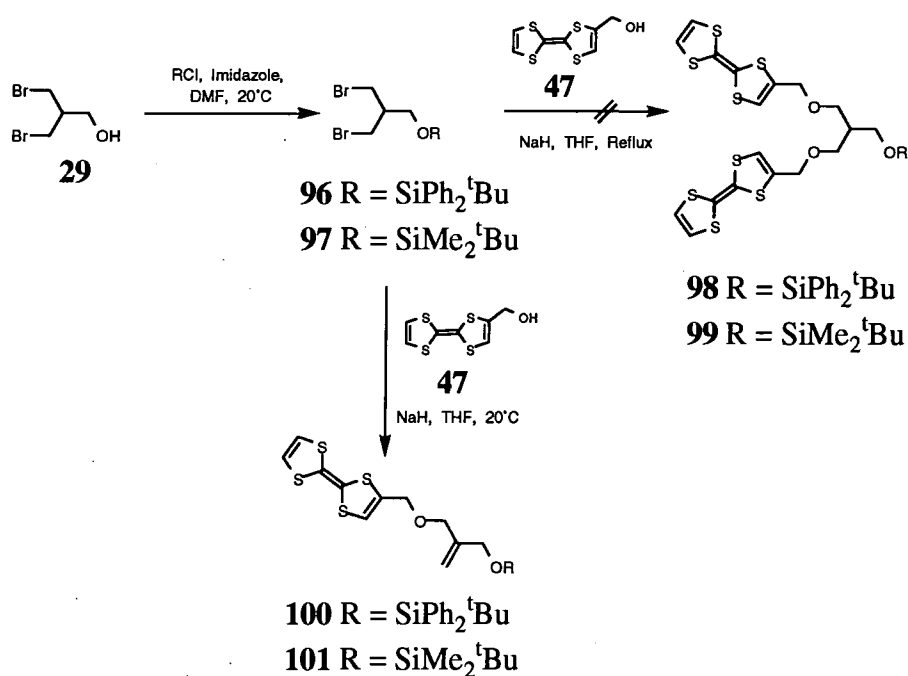
Scheme 5.3.1 Attempted Synthesis of Bis(TTF) Ether Derivatives
