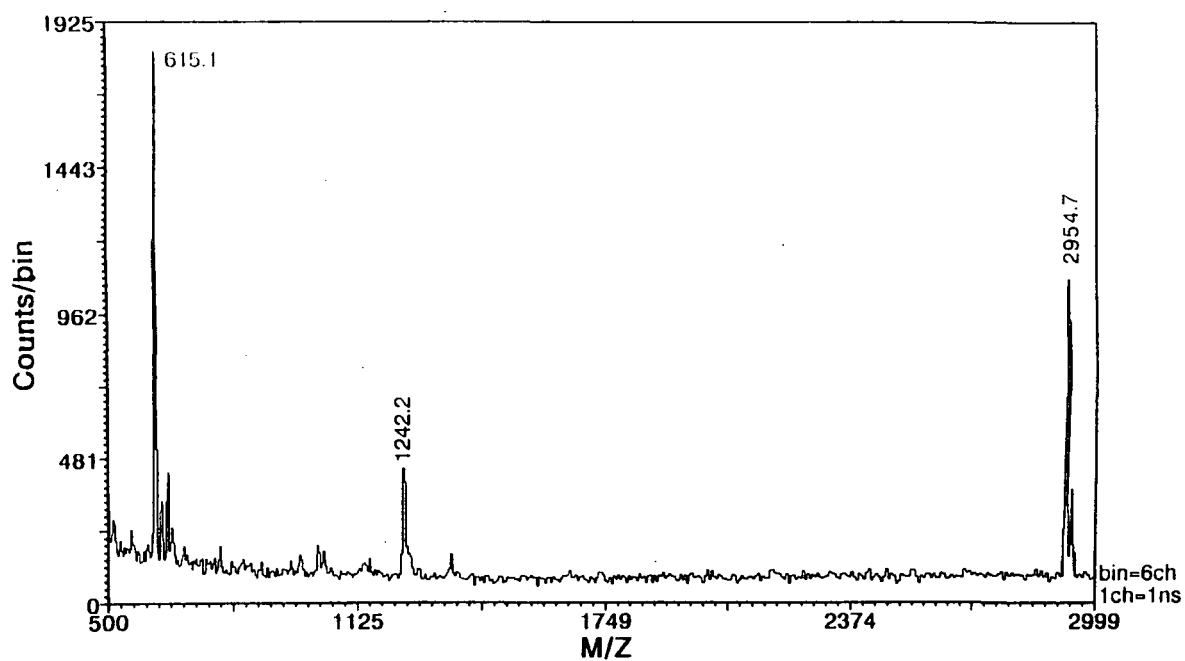
Figure 3.2.1 PDMS Spectrum of Compound 70
