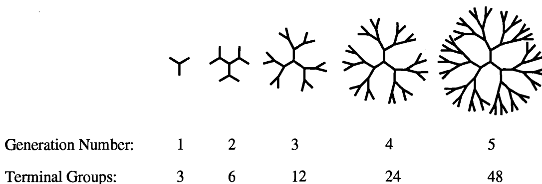
Figure 1.2.5 A Dendrimer Series Illustrating Growth in Size as a Function of Generation Number
