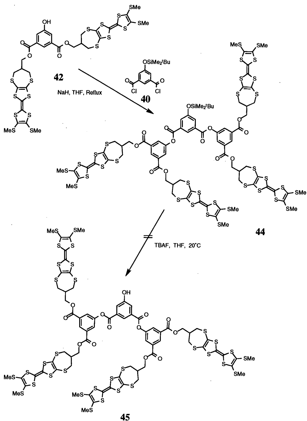
Scheme 2.3.4 Attempted Synthesis of Dendron Wedge 45
