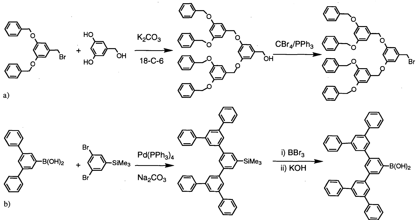
Figure 1.2.8 Examples of Dendron Wedges for Convergent Synthesis of a) Poly(benzylether) Dendrimers 23b b) Hydrocarbon Dendrimers 23c
