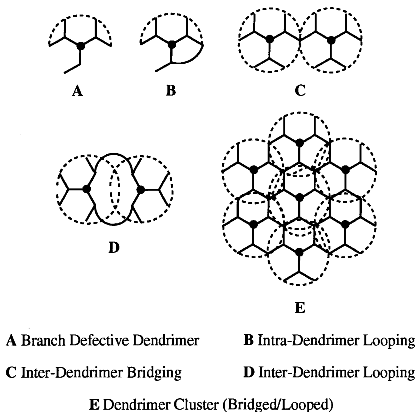
Figure 1.2.7 Schematic Representation of Dendrimer Defects 7d
