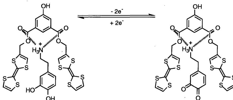
Figure 2.4.5 Reversible Oxidation of Dopamine 62
