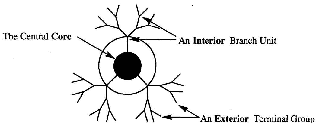
Figure 1.2.2 The Architectural Regions of a Dendrimer
