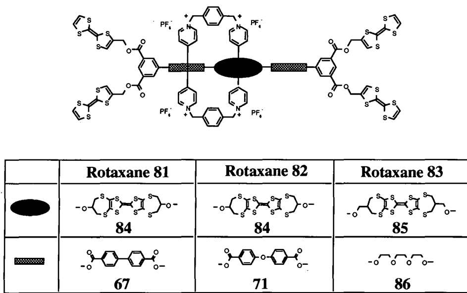
Figure 4.3.1 [2]Rotaxane Design Targets
