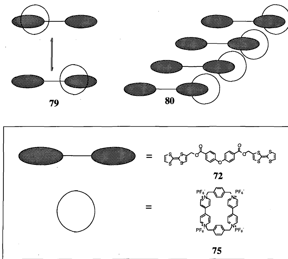
Figure 4.2.3 Conformations of a Complex of Thread 72 and Cyclophane 75
