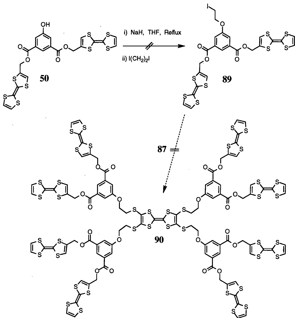
Scheme 5.2.1 Attempted Synthesis of Nona(TTF) 90
