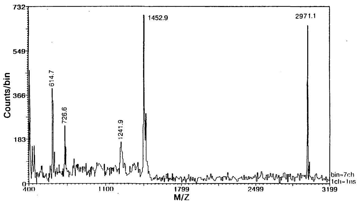
Figure 3.2.2 PDMS Spectrum of Compound 74
