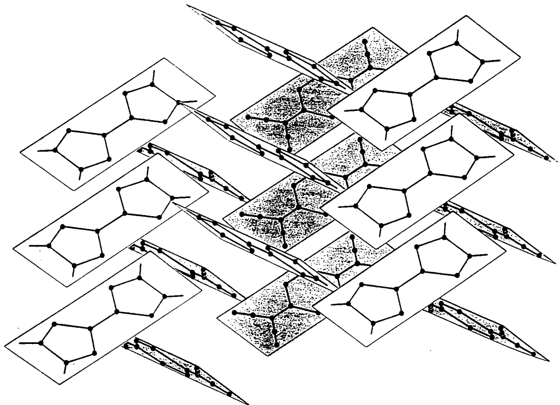
Figure 1.3.2 The 'Herringbone' Crystal Structure of the TTF-TCNQ Charge-Transfer Complex
