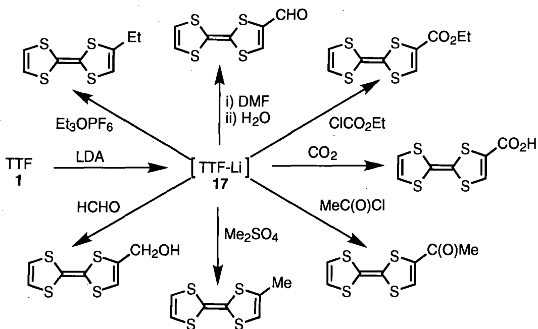
Figure 1.3.4 Substituted Tetrathiafulvalenes via the TTF Anion
