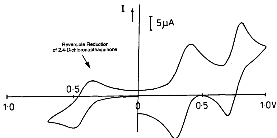
Figure 2.4.1 Classical Voltammogram of Dendrimer 54
