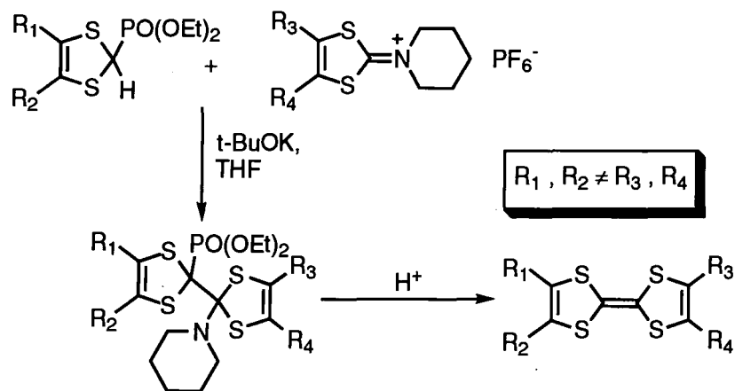
Scheme 1.3.3 Synthesis of Tetrathiafulvalene Derivatives by Reaction of Phosphonate Esters and Iminium Salts
