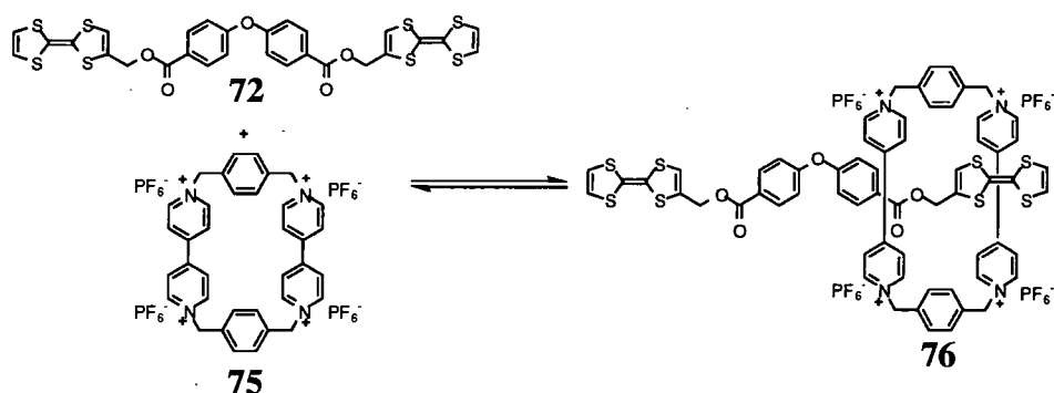
Scheme 4.2.1 Formation of [2]Pseudorotaxane 76
