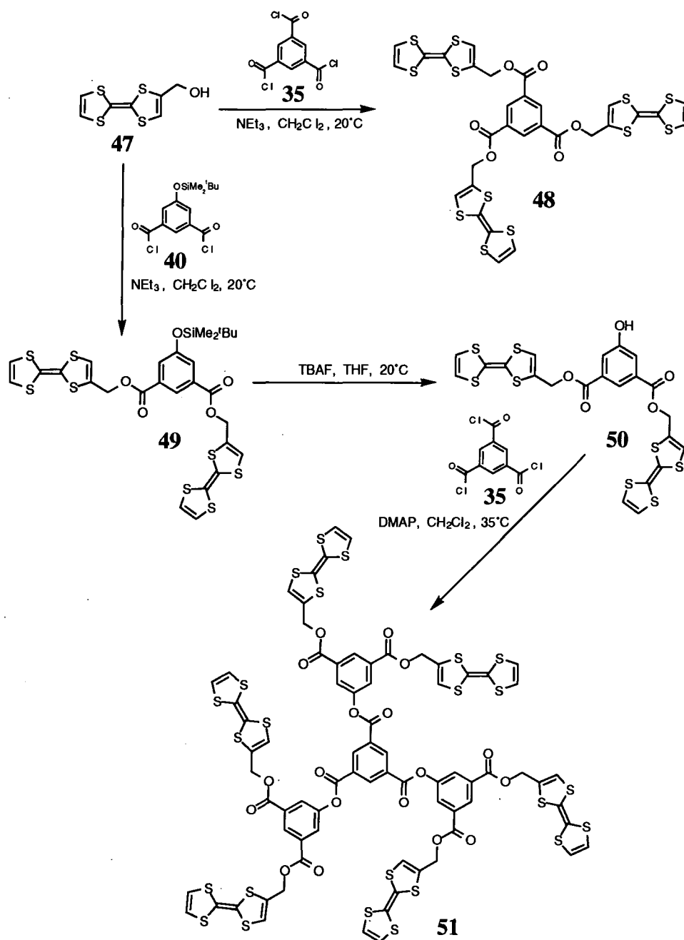
Scheme 2.3.6 Synthetic Pathway to Second Generation Dendrimer 51
