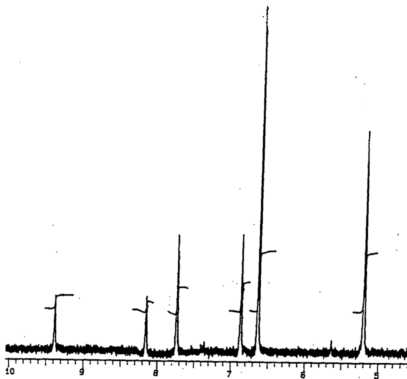
Figure 2.3.1 ^1\text{H} NMR Spectrum of Second Generation Silyl Ether 52
