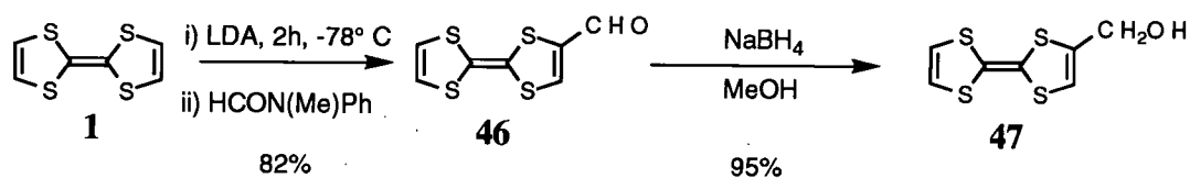
Scheme 2.3.5 Synthesis of 4-(Hydroxymethyl)tetrathiafulvalene 47
