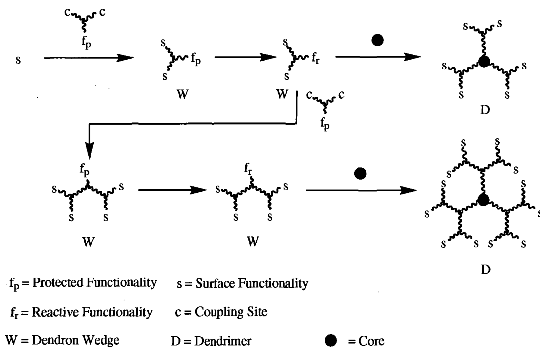
Figure 1.2.6 A Schematic Representation of Convergent Methodology
