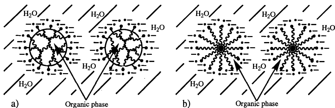
Figure 1.2.3 Comparison of a) a Unimolecular Micelle and b) a Classical Micelle
