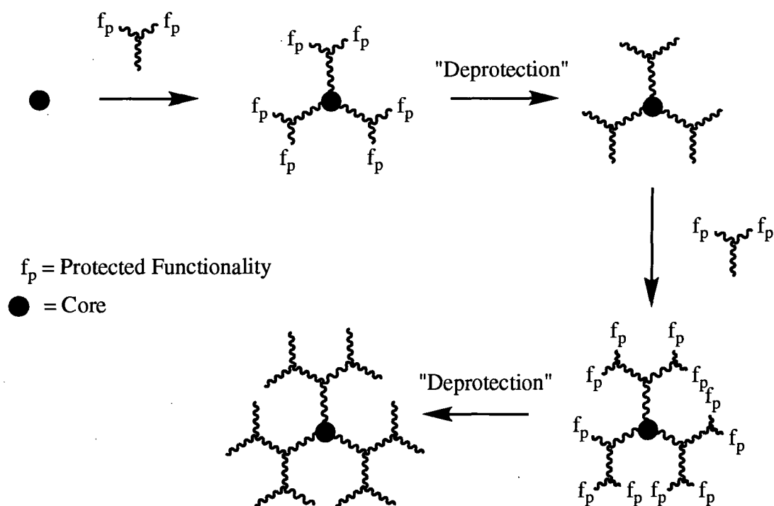
Figure 1.2.4 A Schematic Representation of Divergent Growth Methodology
