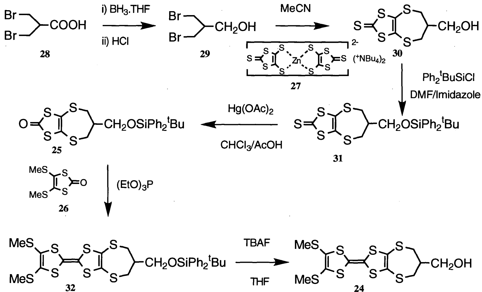
Scheme 2.2.1 Synthesis of 4,5-Di(methylthio)-4',5'-[2-(hydroxymethyl)propylene-1,3-dithio]tetrathiafulvalene
