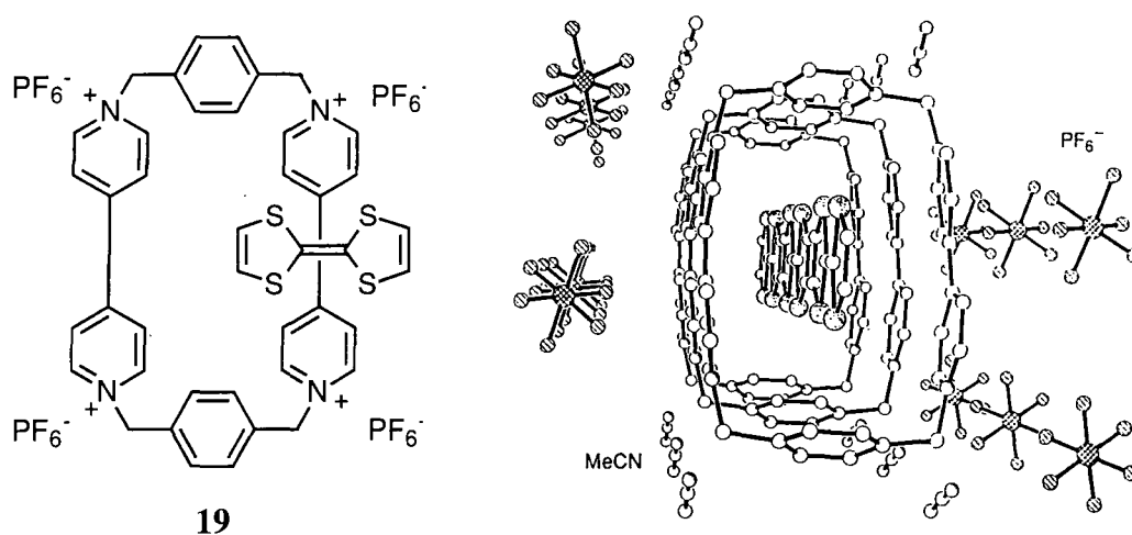
Figure 1.3.5 A Schematic Representation & X-Ray Crystal Structure of a [2]Pseudorotaxane Incorporating Tetrathiafulvalene
