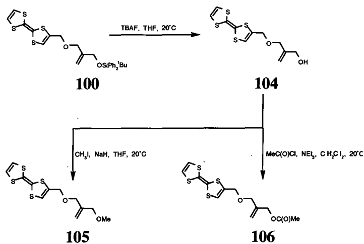
Scheme 5.3.3 Functionalisation of Alcohol 104
