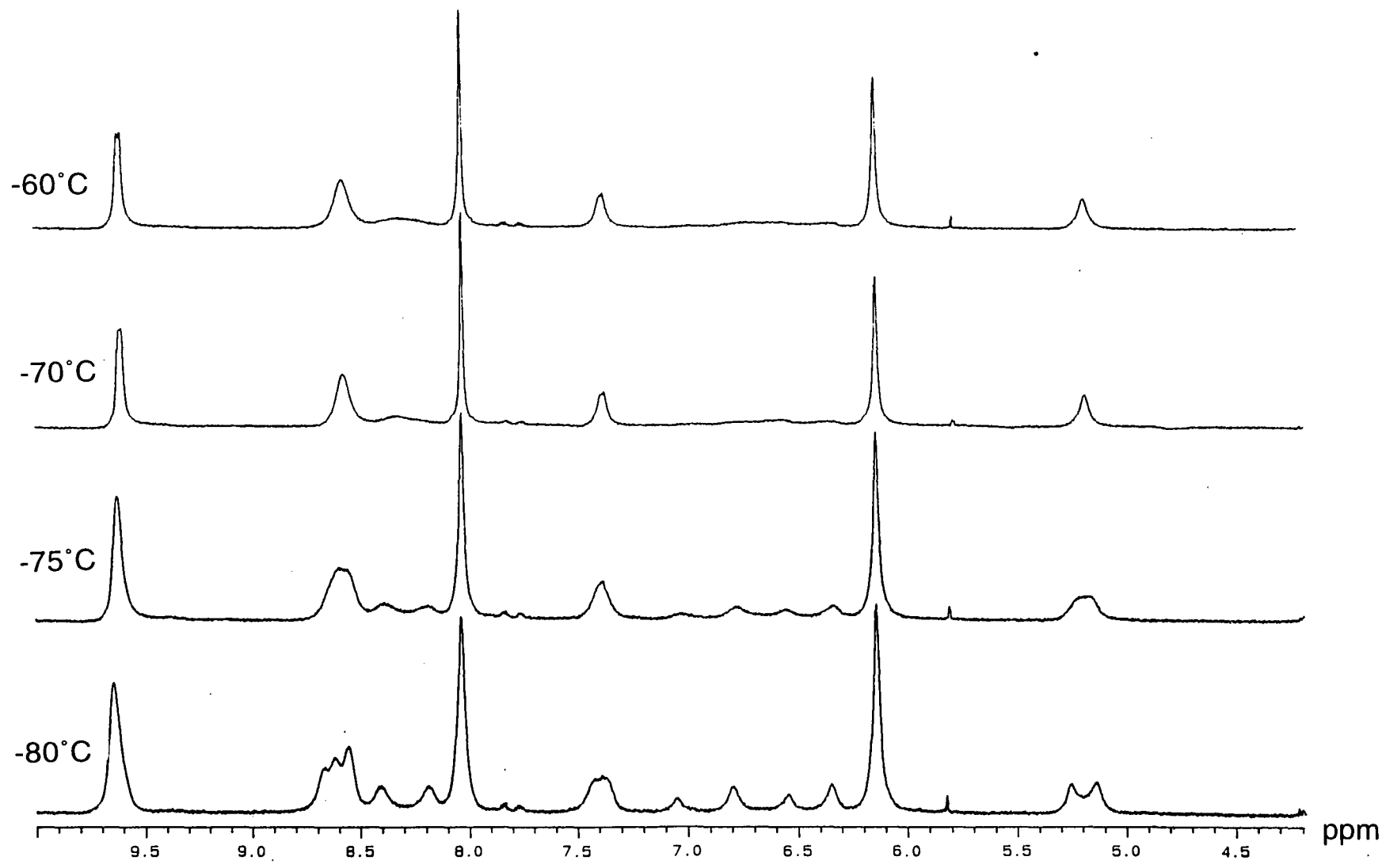
Figure 4.2.2 Variable Temperature ^1\text{H} NMR Spectra of [2]Pseudorotaxane 76 from -60°C to -80°C
