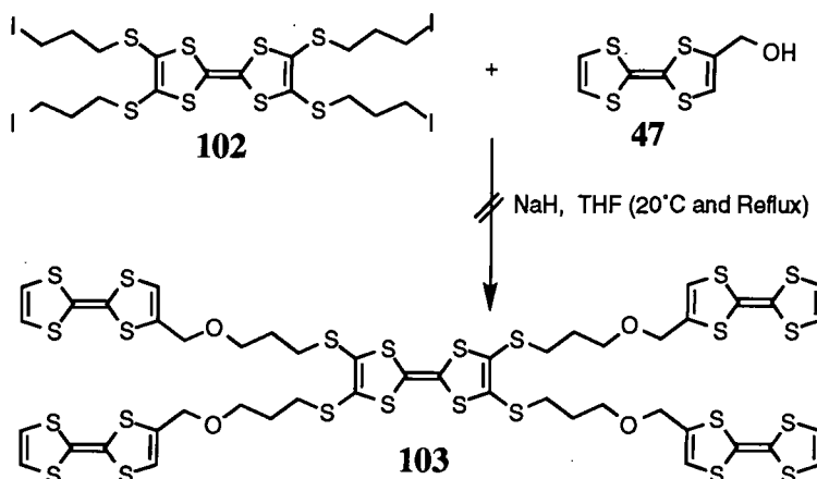
Scheme 5.3.2 Attempted Synthesis of Pentakis(TTF) 103
