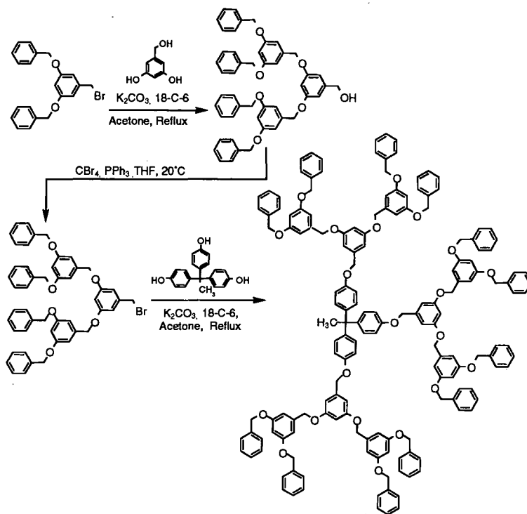
Scheme 2.1.1 The Fréchet Convergent Methodology
