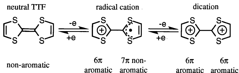
Figure 1.3.1 The Redox Behaviour of Tetrathiafulvalene
