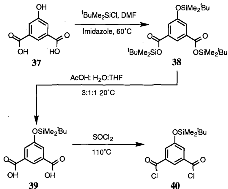
Scheme 2.3.2 Synthesis of Dendritic Monomer 40
