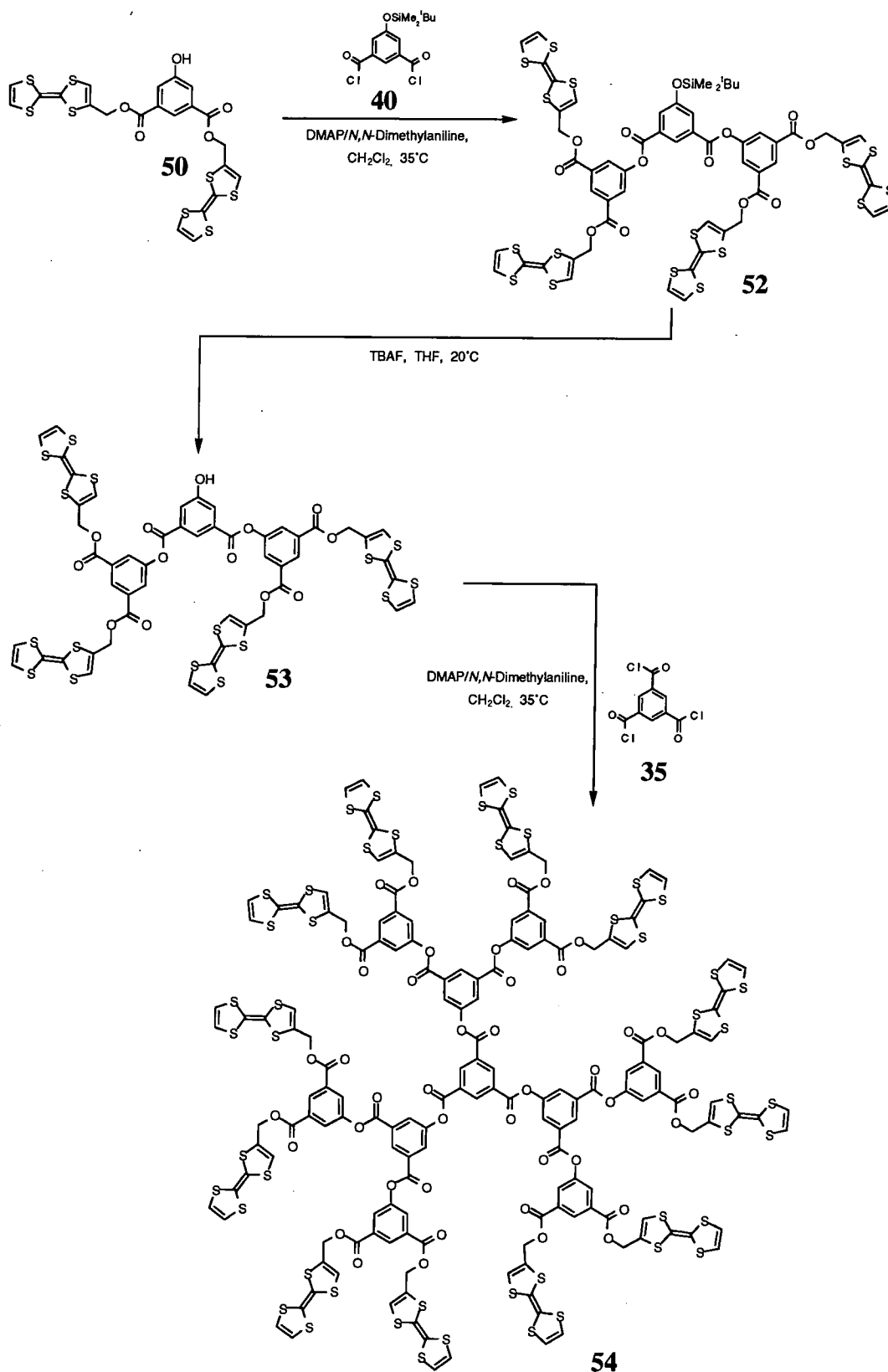
Scheme 2.3.7 Synthetic Pathway to Third Generation Dendrimer 54
