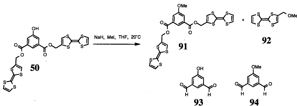
Scheme 5.2.2 Synthesis of Methyl Ether 91
