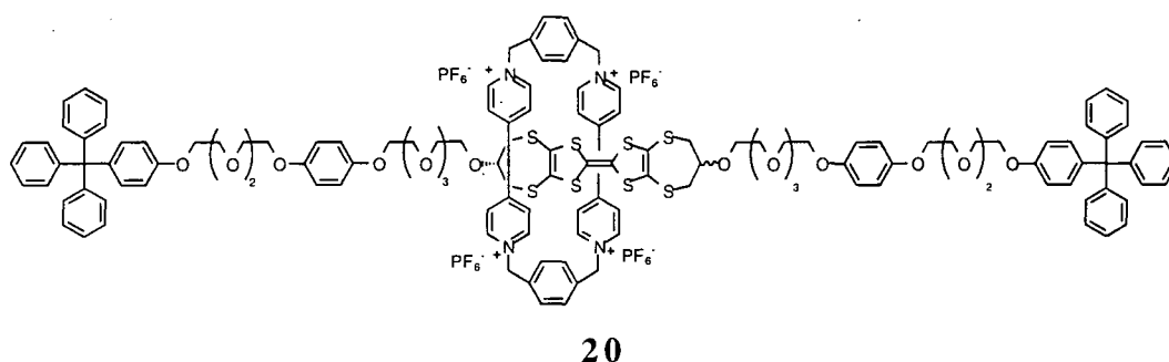
Figure 1.3.5 A Schematic Representation & X-Ray Crystal Structure of a [2]Pseudorotaxane Incorporating Tetrathiafulvalene
