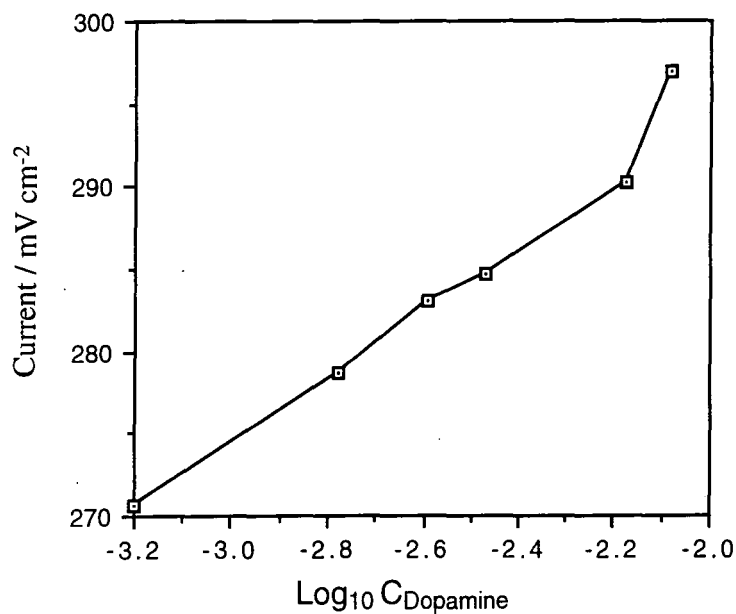
Figure 2.4.4 Graph of Current Response as a Function of Dopamine 62 Concentration
