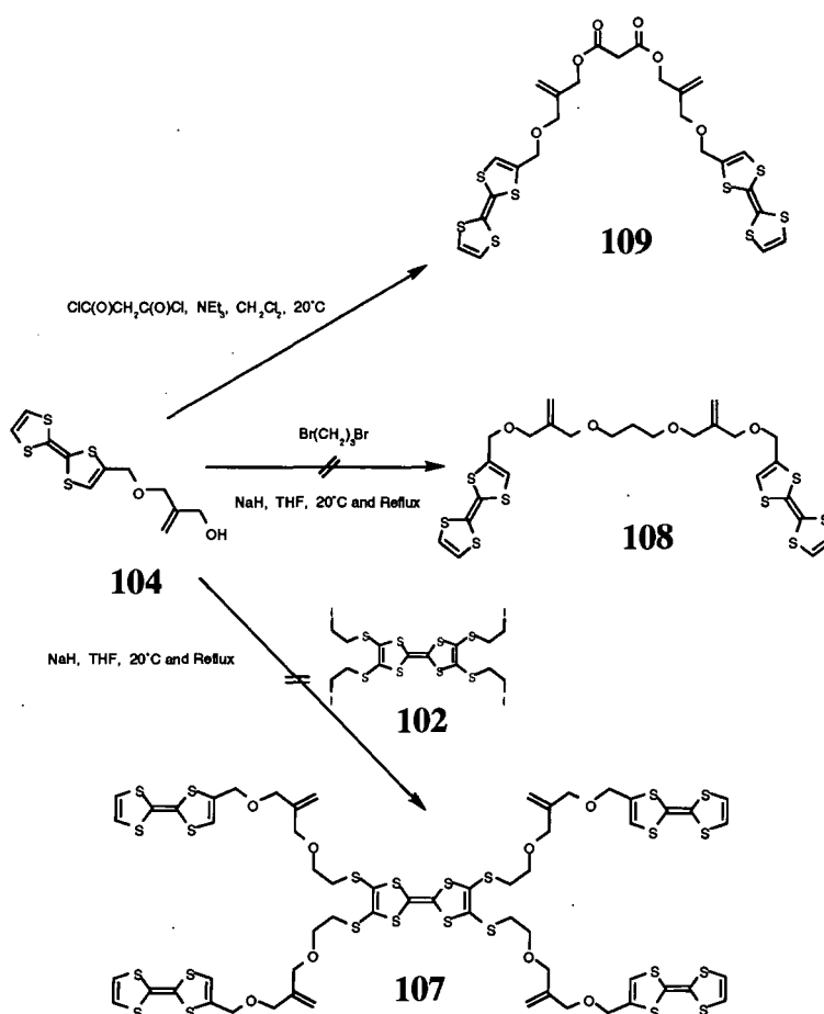
Scheme 5.3.4 Alkyl Multi-TTF Assemblies
