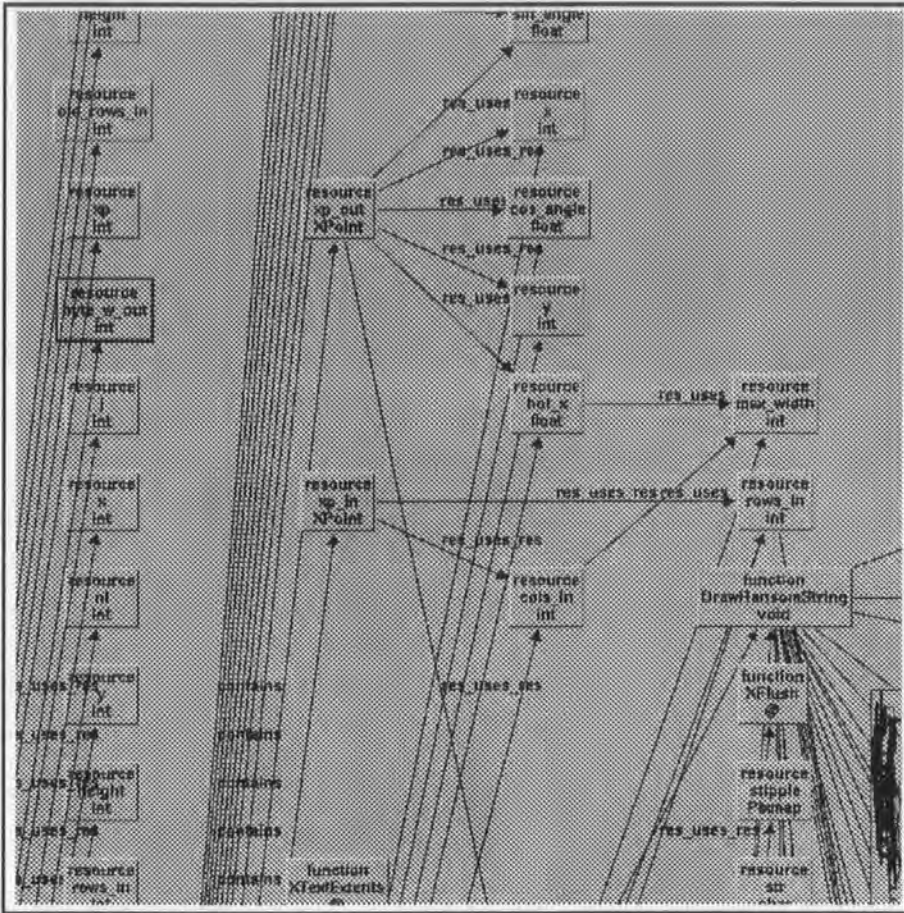
Figure 48 : Sub-graph of the Dependencies for “gtest”.
