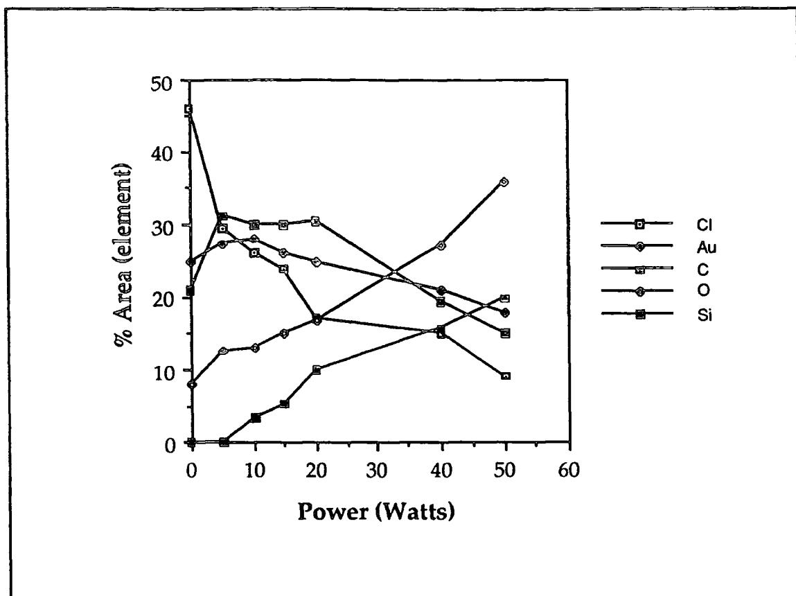
Fig. 5.10 50% AuCl 3 on Glass as a function of Power, Treatment Time of 10 mins.
