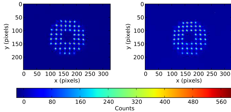
Figure 3.8: Example SH spot pattern from two single Andor Luca EMCCD cameras. The target stars had an angular separation of 16'' . There are still off-axis aberrations but very little windshake.
