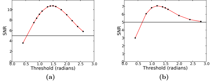
Figure 4.6: SNR obtained as a function of threshold for observing a faint companion at 2\lambda/D and \delta m = 7.7 with a D = 1 m telescope (a) and \delta m = 11.7 with a D = 8 m telescope (b). The solid black line shows the SNR for the un-masked system.
