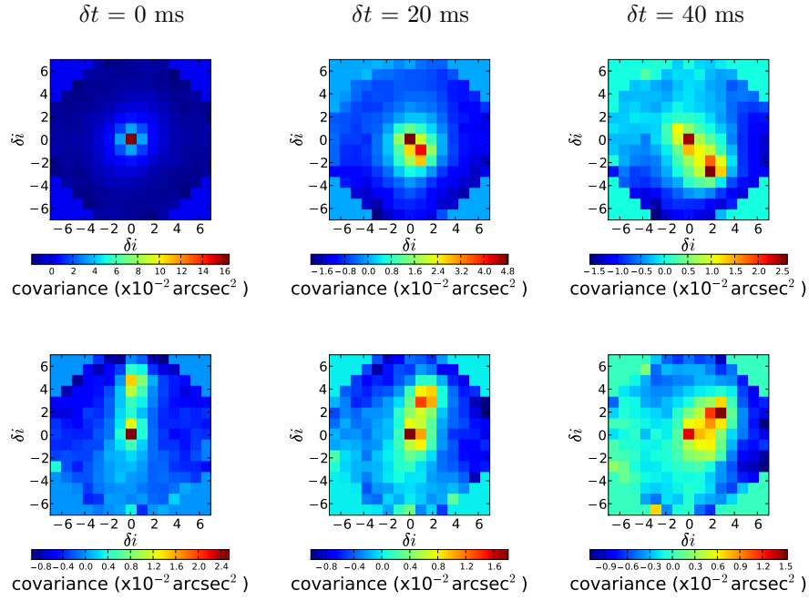
Figure 2.22: Example 2D auto-covariance and cross-covariance maps with increasing temporal offset, \delta t . By correlating one set of centroids with another set taken a time, t , later and measuring how far the correlation peak has moved we can estimate the wind speed of the turbulent layer. The top row shows the auto-covariance and the bottom row shows the cross-covariance with a temporal delay of 20 ms per frame. The data shows that on this occasion the turbulence was dominated by the surface layer. This is because the moving peaks in the cross and auto-correlation plots move in the same direction and at the same speed suggesting that it is very likely they are the same layer and there are no other obvious peaks in the auto-correlation. The residual peak in the centre is because the data has not been filtered for tube seeing.
