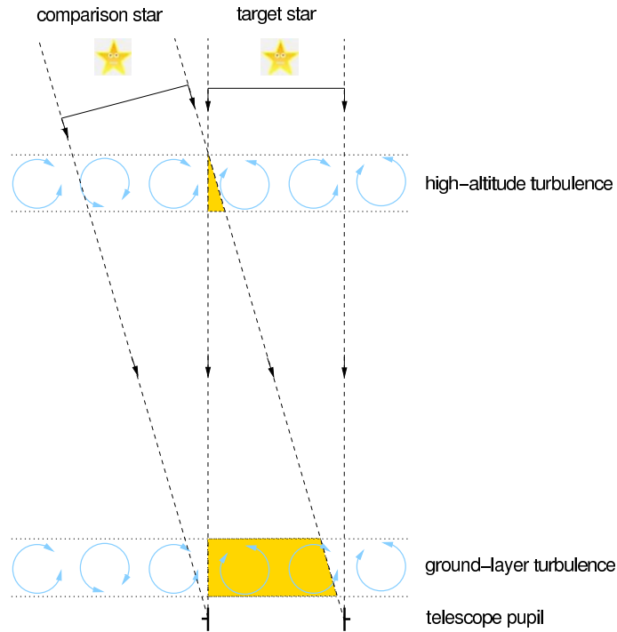
Figure 5.7: In differential photometry the intensity of the target star is calibrated by the intensity from a second comparison star. As the scintillation is caused by high altitude turbulence the two light cones do not sample the same turbulence and hence there will be very little correlation between the two. By conjugating the telescope to the high-altitude layer we remove the scintillation from this layer and it is replaced by scintillation from the surface turbulent layer instead. However, as the two light cones sample the same region of turbulence near the ground they will have very similar scintillation patterns, allowing one to be corrected by the other. The angle of separation of the two stars can be large as the surface layer is generally found to be thin. (Diagram courtesy of V. Dhillon)
