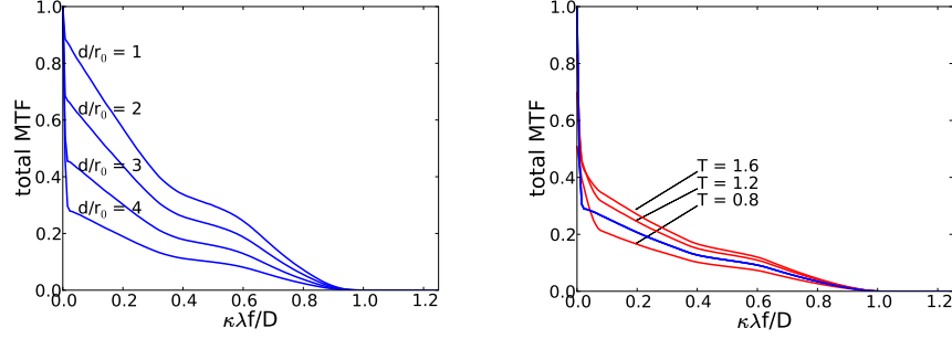
Figure 4.15: Combined MTF from the telescope and atmosphere, MTF_{\text{atmos}} \times MTF_{\text{tel}} . The plot on the left shows the total MTF for AO correction with d/r_0 values of 1, 2, 3 and 4. Although it appears that the MTF curves do not all converge to 1 at \kappa = 0 this is not true. The telescope diameter was chosen to be 8 m and MTF_{\text{atmos}} drops to its convergent value very quickly ( \sim \kappa\lambda f/d (figure 2.10)) therefore MTF_{\text{atmos}} can be considered constant. The plot on the right shows the total MTF for an 8 m telescope with 16 \times 16 AO, d/r_0 = 4 and threshold values of 0.8, 1.2 and 1.6.
