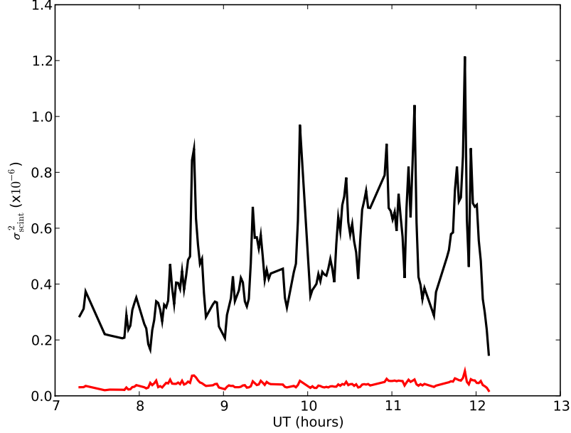
Figure 5.18: Predicted scintillation variance as a function of time for the night of 19 th May 2000. The black line is the expected scintillation variance for differential photometry and the red line is the scintillation corrected variance.
