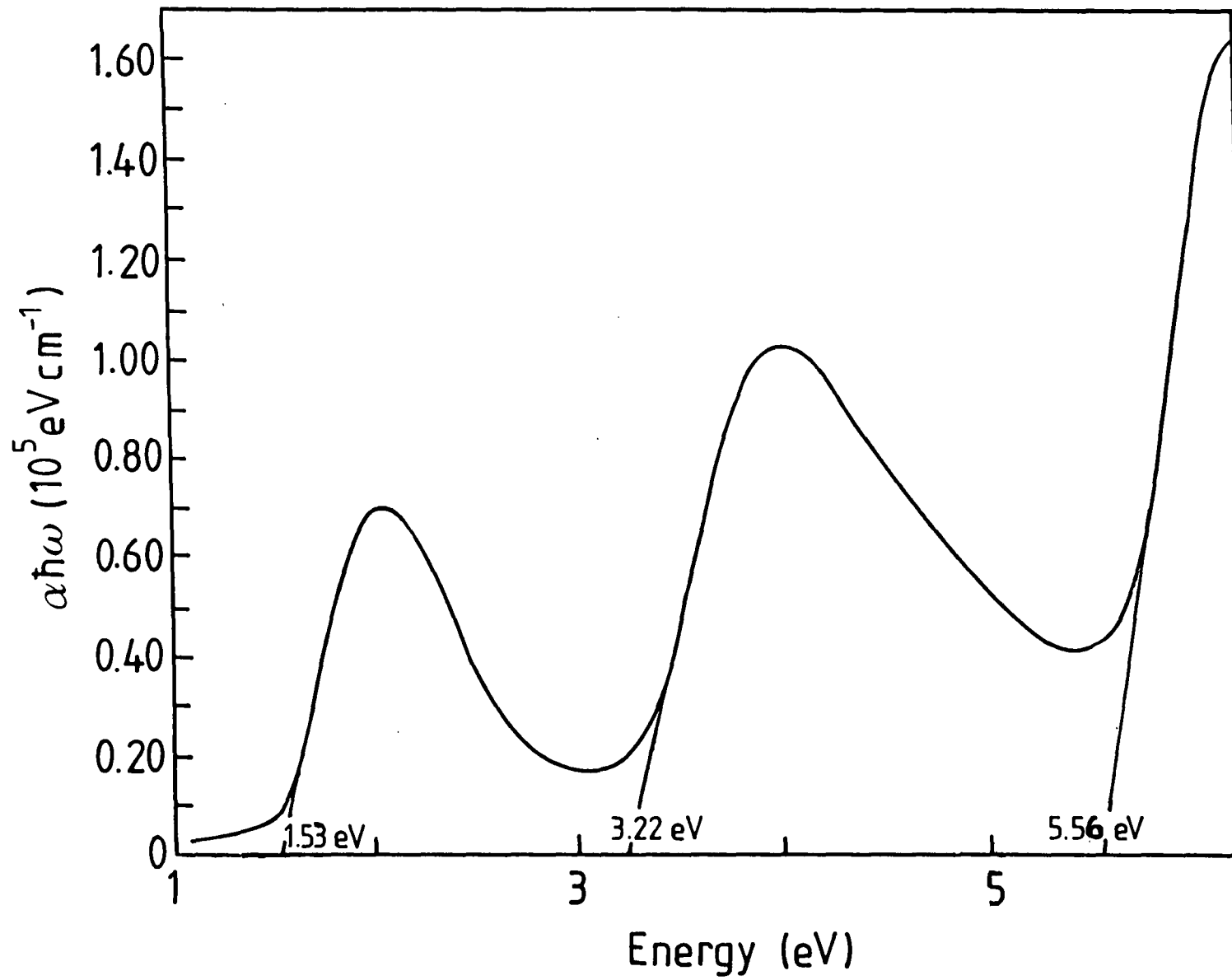
Figure 3.12. The variation of \alpha h\omega , with energy for a centrifuged solution which has been spun on a sapphire substrate to a thickness of 0.180 \mu\text{m} .
