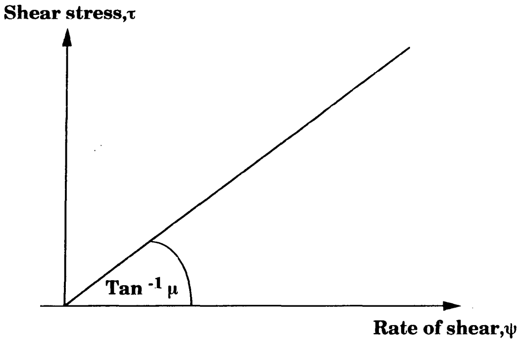
Figure 2.17. The relationship between viscosity \mu , shear stress \tau and rate of shear \psi , for a Newtonian fluid. A film of equal thickness is formed.
