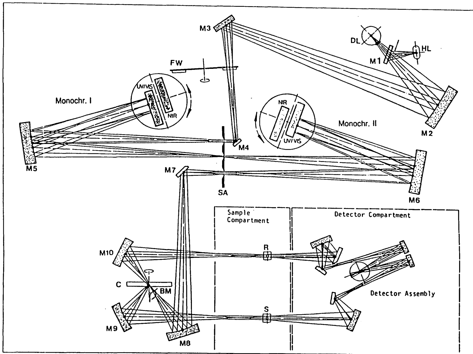
Figure 3.3. The layout of the spectrophotometer.
