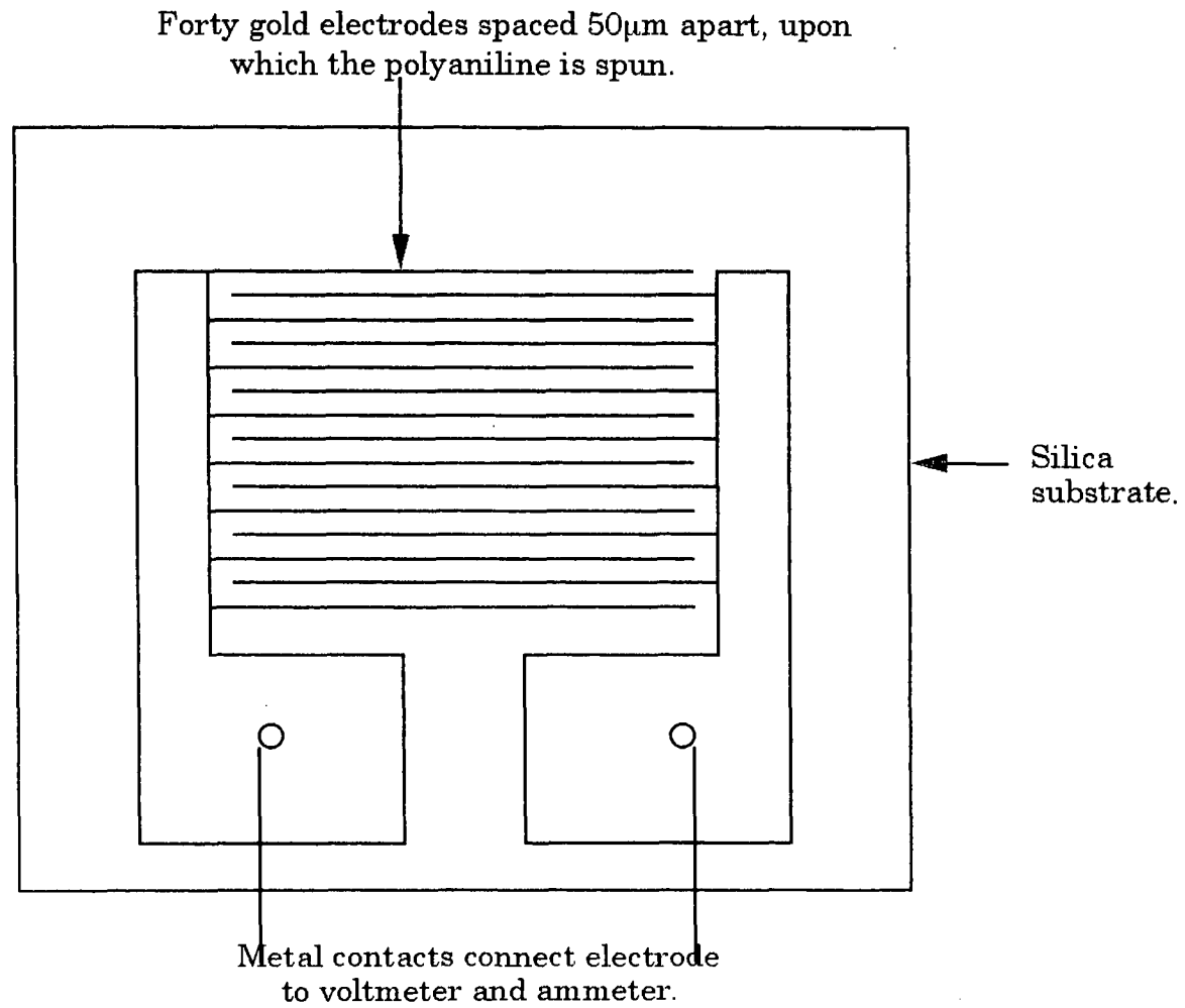
Figure 4.4. This shows the interdigitated electrodes used for the gas sensing experiments.
