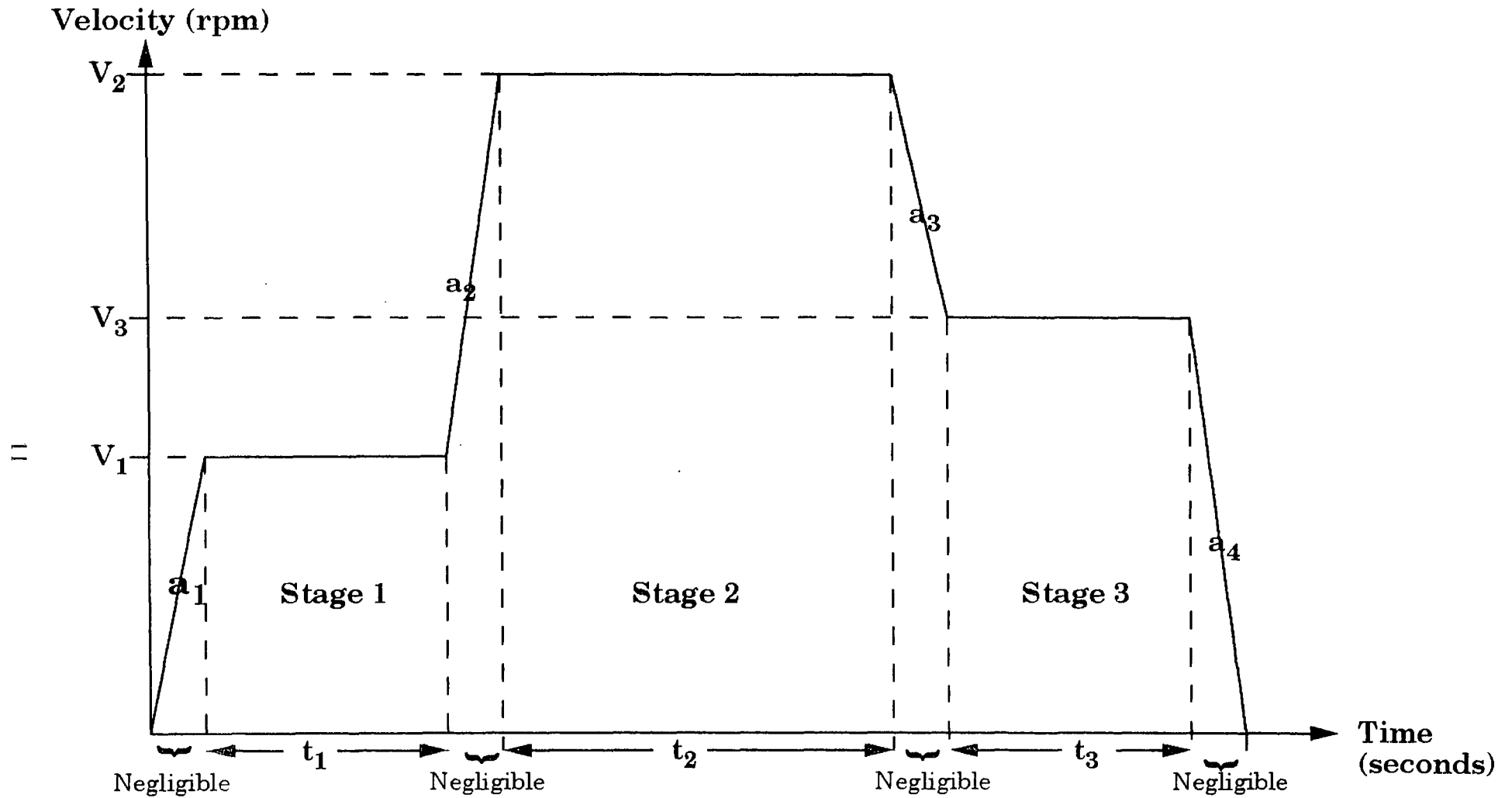
Figure 2.4. The three stages of the spinning process.
