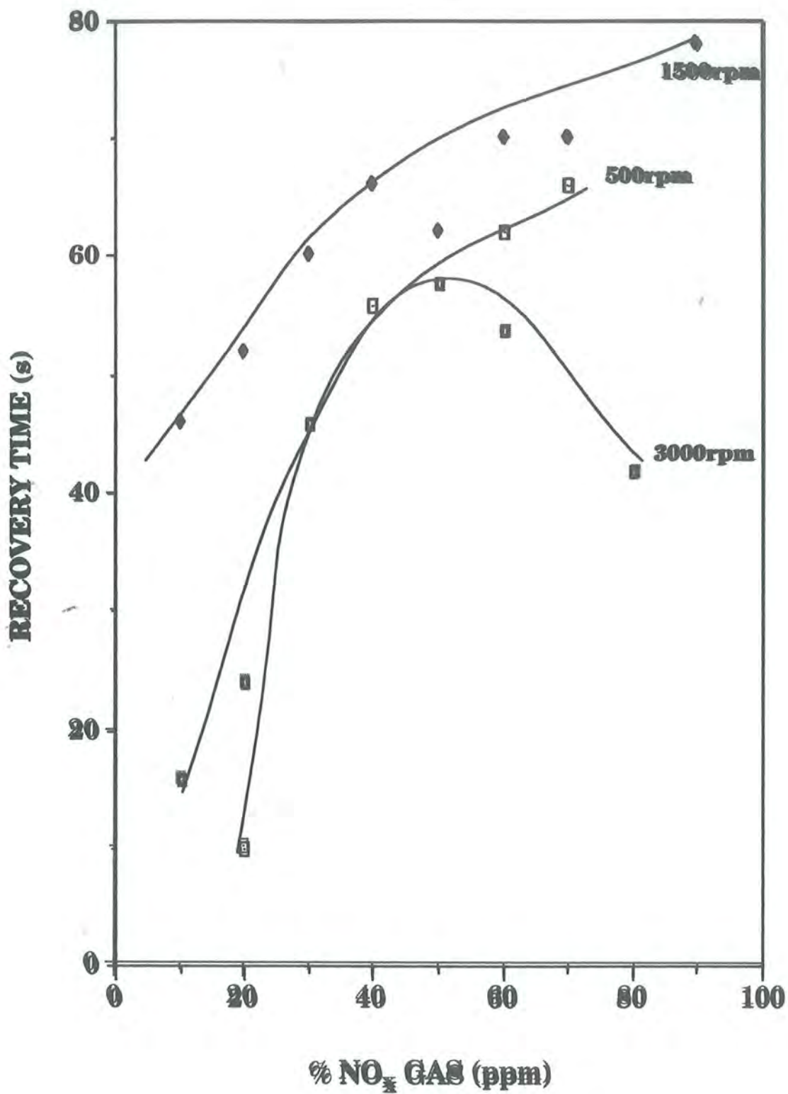
Figure 4.11. The time taken for each device to recover after exposure to each % concentration of NO x gas.
