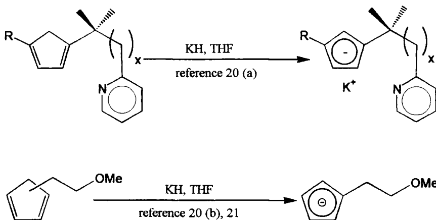
Figure 1.3.2: Potassium salts of Lewis-base functionalised cyclopentadienide anions
