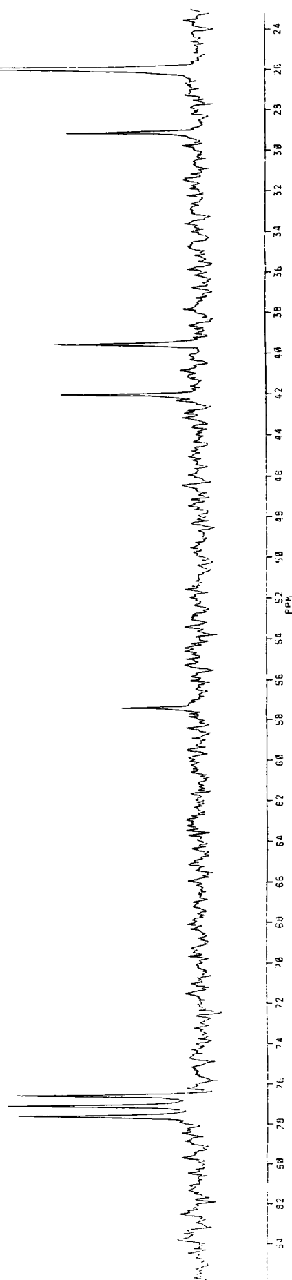
Figure 2.8.4: The 13 C{ 1 H} NMR spectrum of pure 2.4 at 62.5 MHz in CDCl 3 (marked S)
