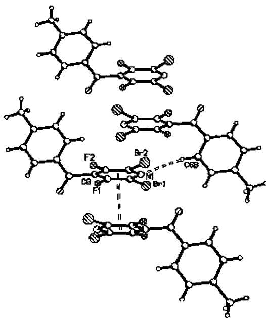
Fig 1: two neighbouring molecules of (31)
