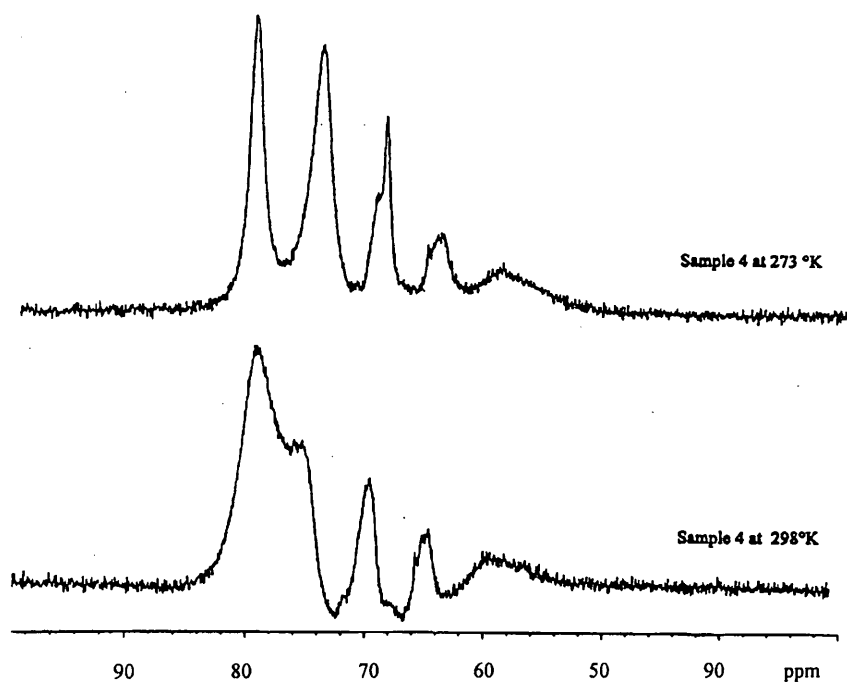
Figure 4.9. Stacked plot of high-resolution 156.3 MHz ^{27}\text{Al} NMR spectra at 0°C and 25°C of TMAOH aluminosilicate solutions with the ratio \text{Si}/\text{Al} = 6 and Si and Al concentrations 0.084 and 0.014 M respectively (sample 4). The spectra were taken two months after mixing. Spectrum conditions: Spectral width 50000.0 Hz. Acquisition time 0.205 s. Recycle delay 0.100 s. Pulse duration 45.0 \mu\text{s} (192.9 degree). Number of transients 8192.
