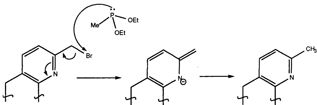
Scheme 4.13 Competing process
