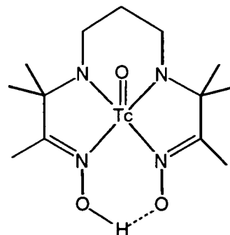
(14)Tc-HMPAO
