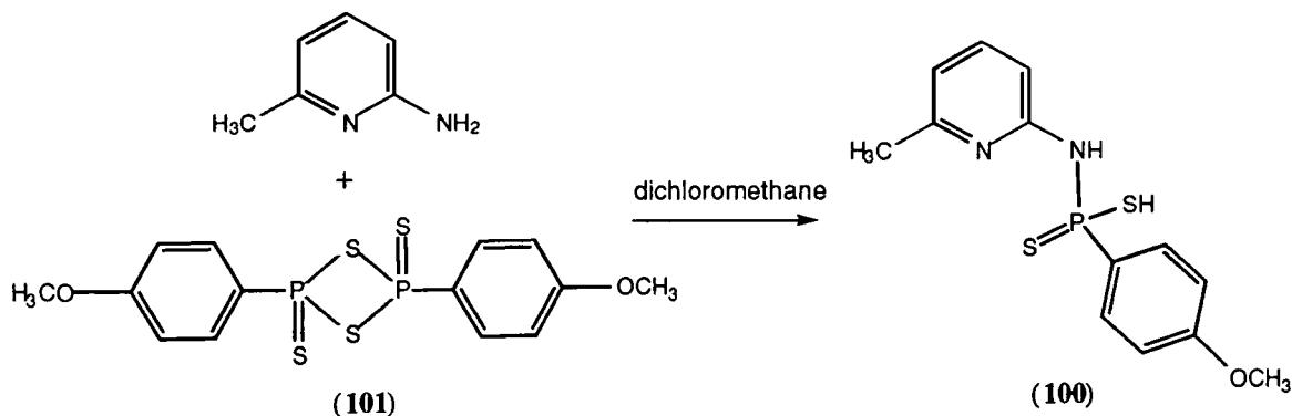
Scheme 3.14 Synthesis of dithiophosphinate ligand
