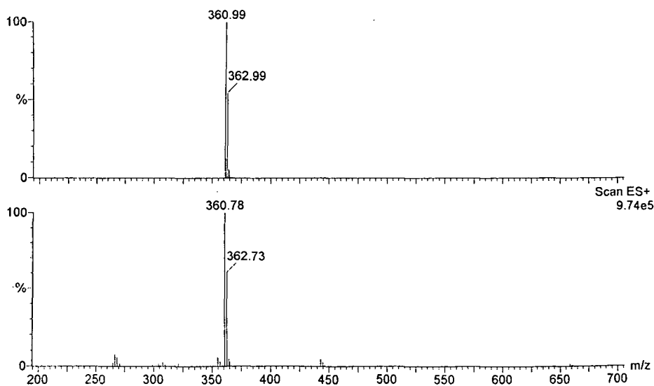
Figure 3.8 ESMS + spectrum of Cu(I)(85) showing loss of one ligand proton
