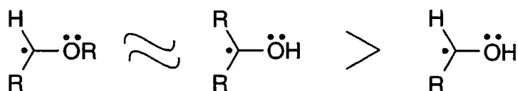
Scheme 4.4.c.i. Reactivities of oxygen-stabilised radical centres.
