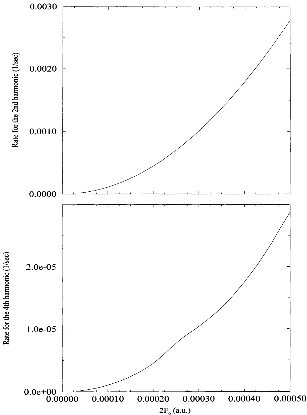
Figure 7.14: Variation of the rate for the 2nd (above) and 4th (bottom) harmonic from hydrogen with respect to dc-field strength. The ac-field intensity and wavelength are I = 10^{13} W/cm 2 and 1064 nm, respectively.
