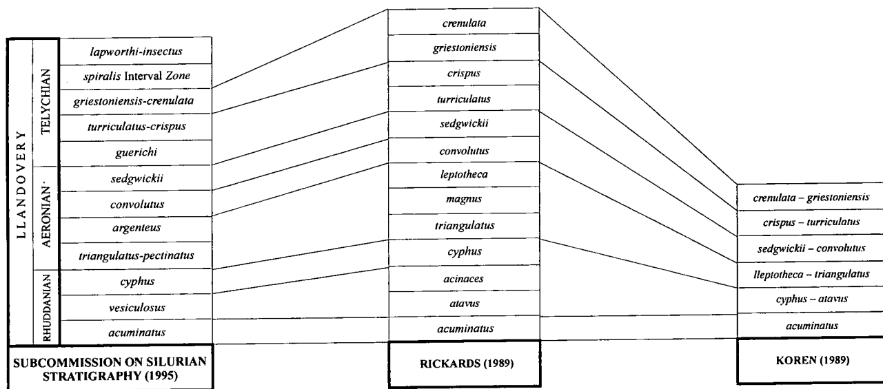
Figure 2.4 Correlation of the proposed standard graptolite biozonal schemes for the Llandovery.
