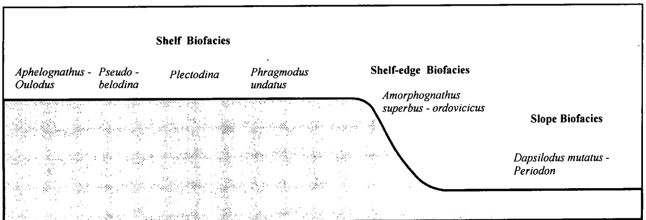
Figure 5.4 Conodont biofacies in the Upper Ordovician to the Lower Silurian around the margins of Laurentia.
