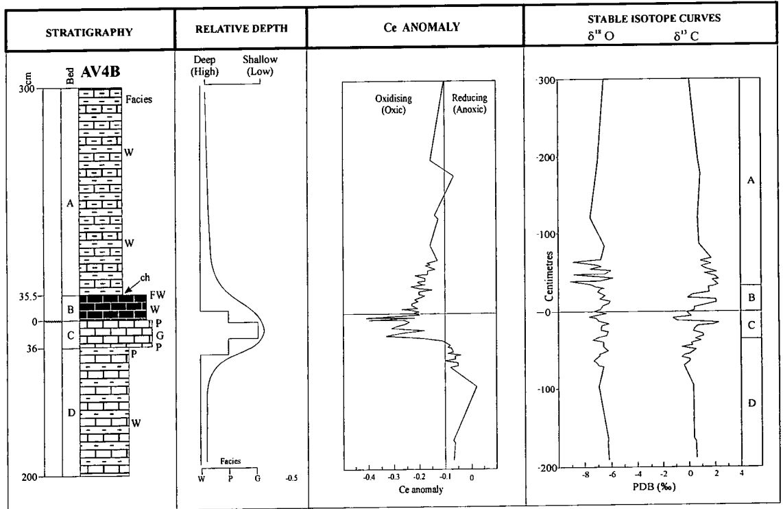
Figure 2.22 Lithological, sea-level and geochemical variations through the Avalanche Lake section. After Wang et al. (1993b). Beda D-A are within the Whittaker Formation. Symbols for microfacies: W, wackstone; P, packstone; G, peloidal grainstone; FW, floatstone in a wackestone matrix; ch, condensed horizon.
