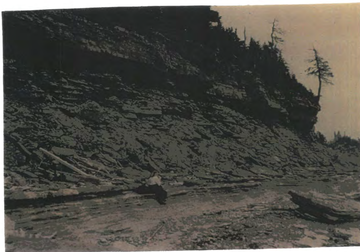
Figure 3.24 The Brisants Jumpers locality (Locality AI 5): an exposure of the Ferrum and Pavillion Members of the Jupiter Formation, overlain by the Chicotte Formation.
