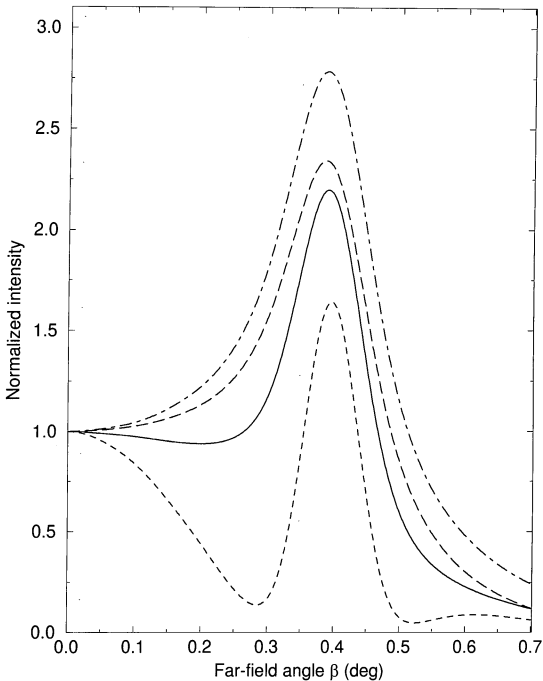
Figure 5.8: Far-field profile for a Bessel-Gauss beam ( \alpha = 1.2^\circ , b_G = 48.7 mm) as a function of the far-field angle \beta for various peak focal intensities I_f , obtained within the time-dependent approach (full calculation). Dashed line: I_f = 3 \times 10^{13} \text{ W/cm}^2 , solid line: I_f = 1 \times 10^{13} \text{ W/cm}^2 , long-dashed line: I_f = 5 \times 10^{12} \text{ W/cm}^2 , dot-dashed line: I_f = 1 \times 10^{12} \text{ W/cm}^2 .
