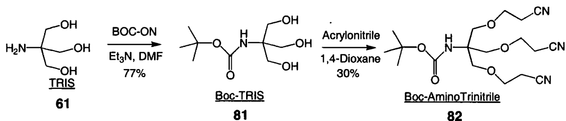
Figure 4.11 – Boc Protection of TRIS
