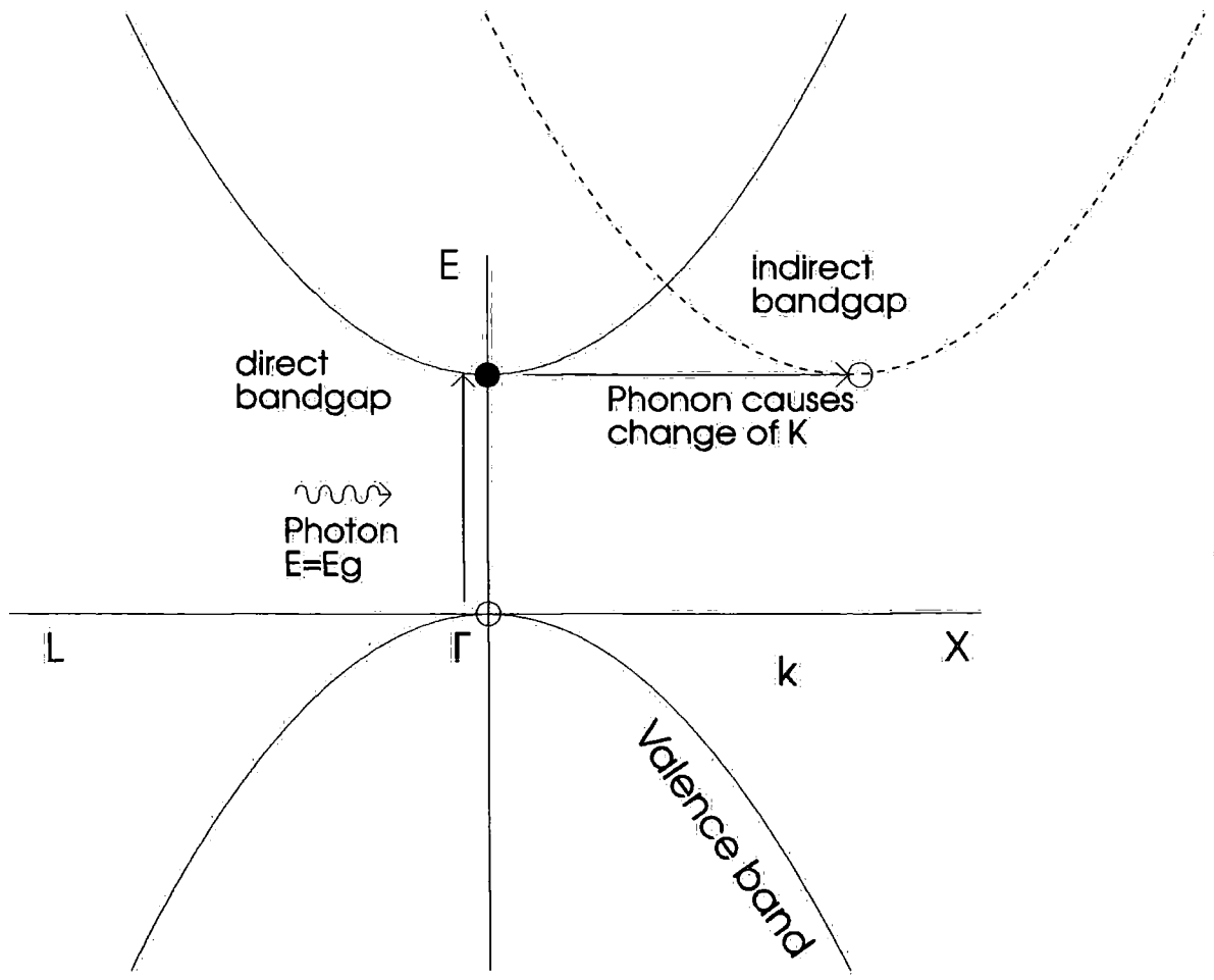
Figure 2.8: Direct and indirect bandgap semiconductor absorption.
