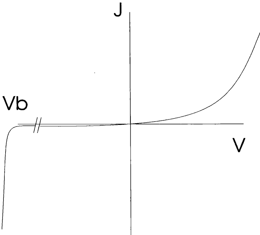
Figure 2.12: Generic J-V characteristics of a p-n junction.
