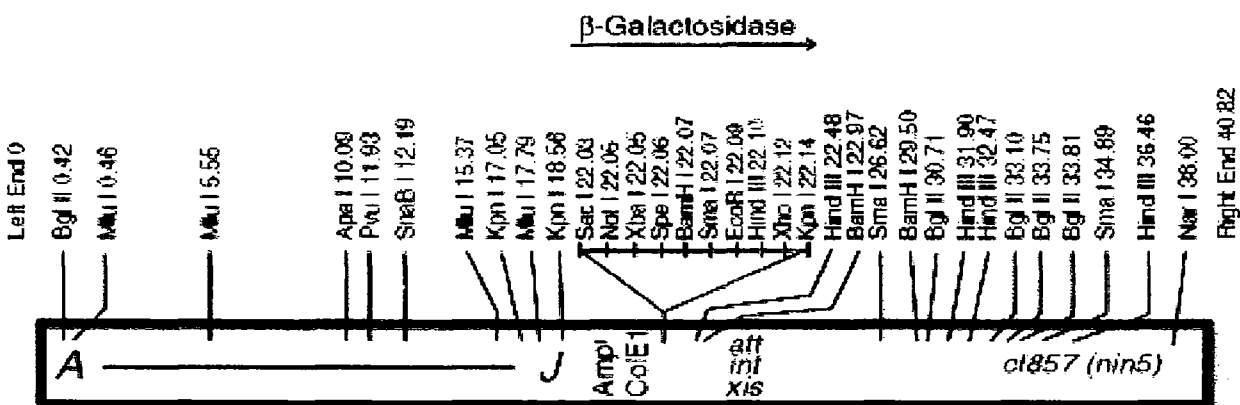
Lambda ZAP ® II vector © Stratagene
