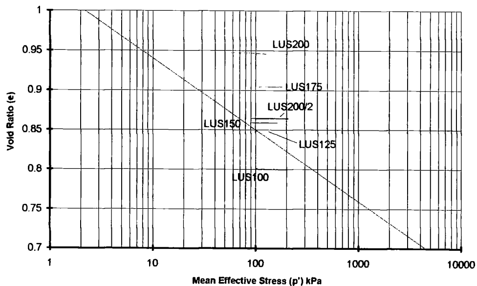
Figure 5-43 Void ratio versus mean effective stress for LUS '100-200' tests
