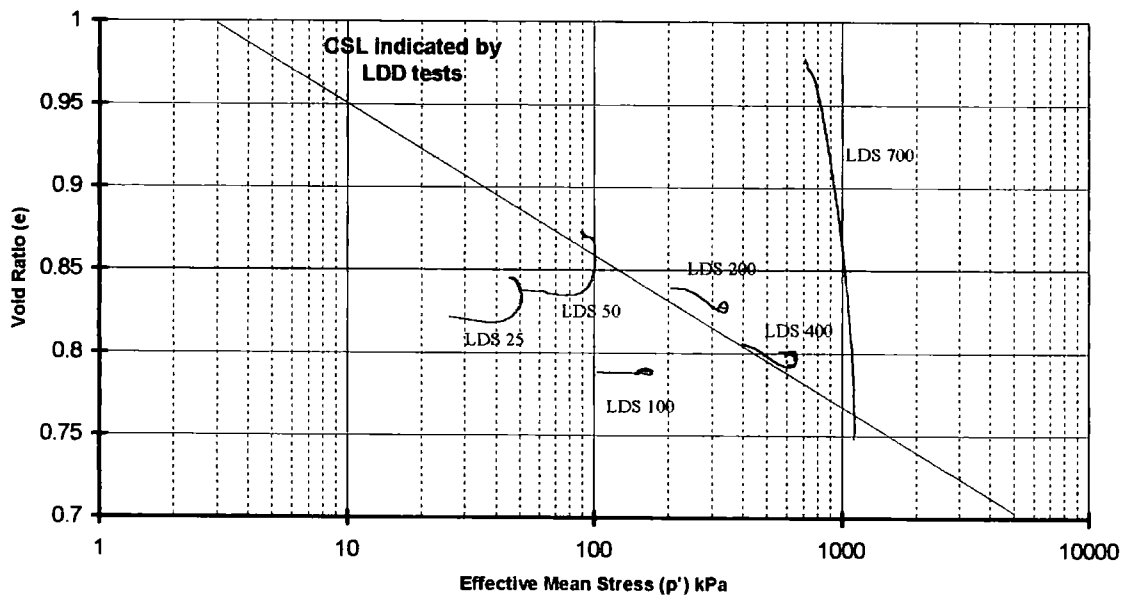
Figure 5-12 Void ratio changes against mean effective stress for LDS tests
