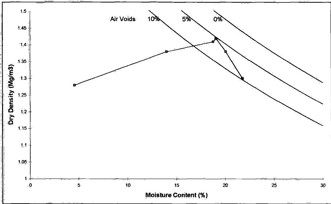
Figure 3-6 Compaction results on fly ash from Drax
