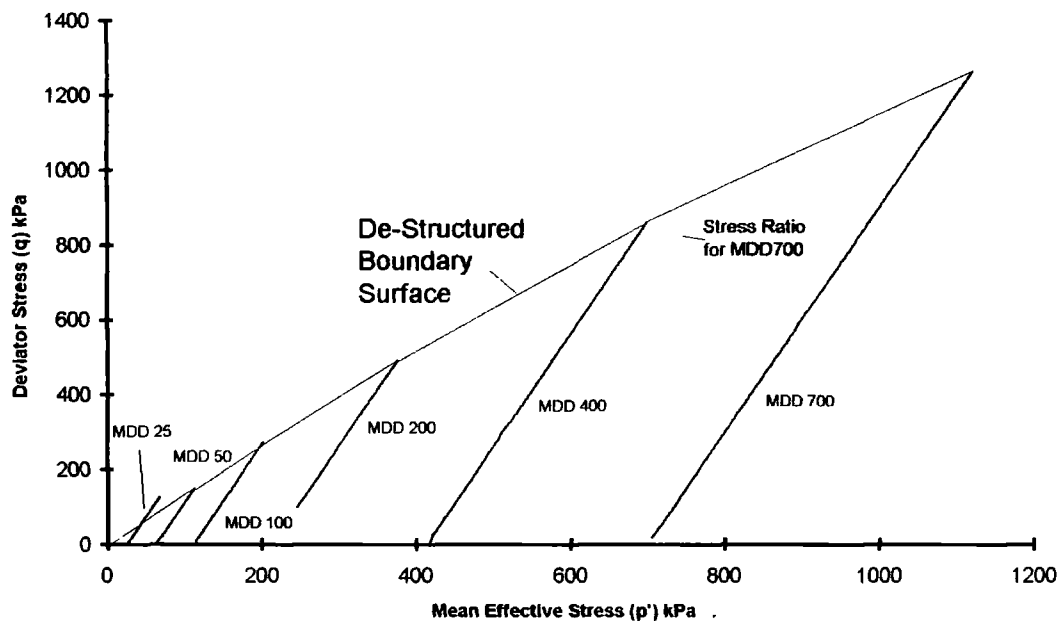
Figure 6.5 Effective stress paths for MDD tests
