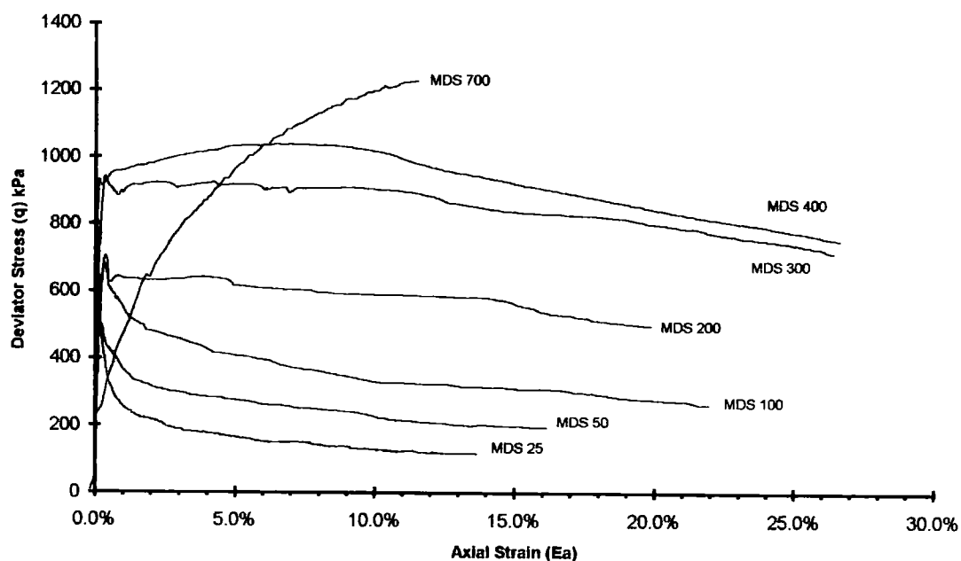
Figure 6.9a Stress against strain plot for MDS tests
