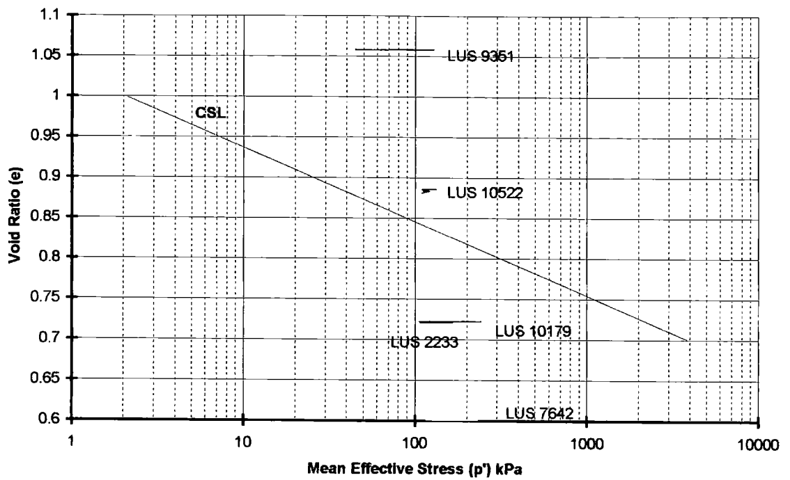
Figure 5-60 Void ratio against mean effective stress for BS406 tests at 125kPa confining pressure
