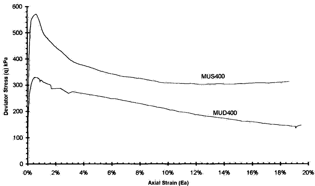
Figure 6-41 Comparison between structured and de-structured stress-strain curves for specimen tested at 400kPa confining pressure
