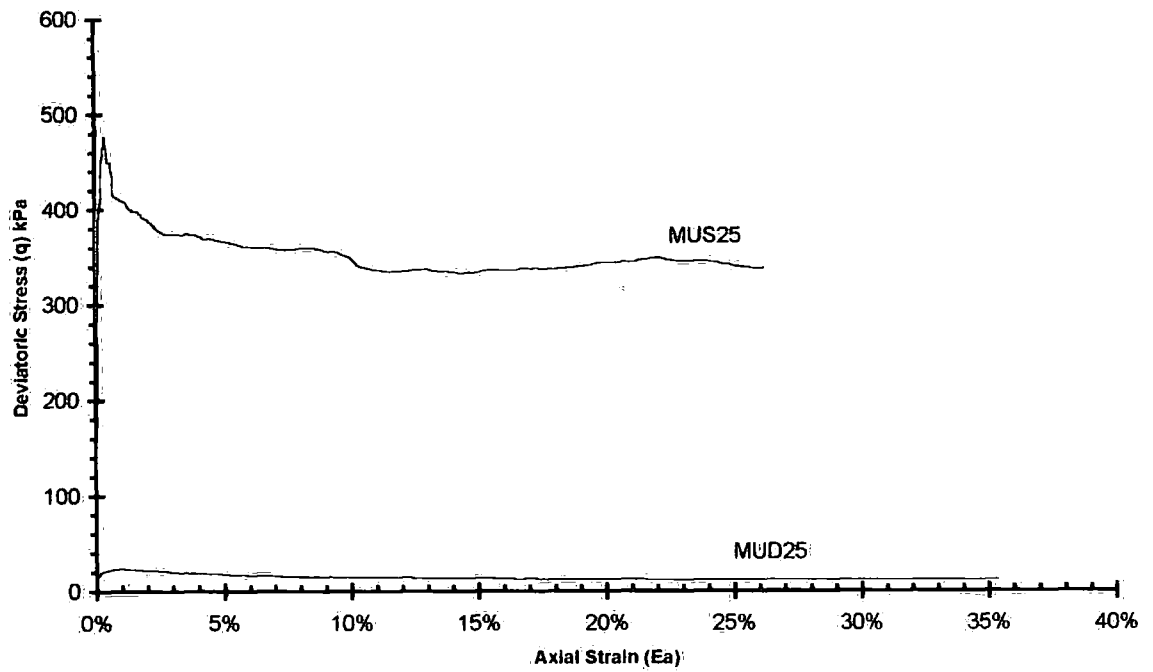
Figure 6-39 Comparison between structured and de-structured stress-strain curves for specimen tested at 25kPa confining pressure
