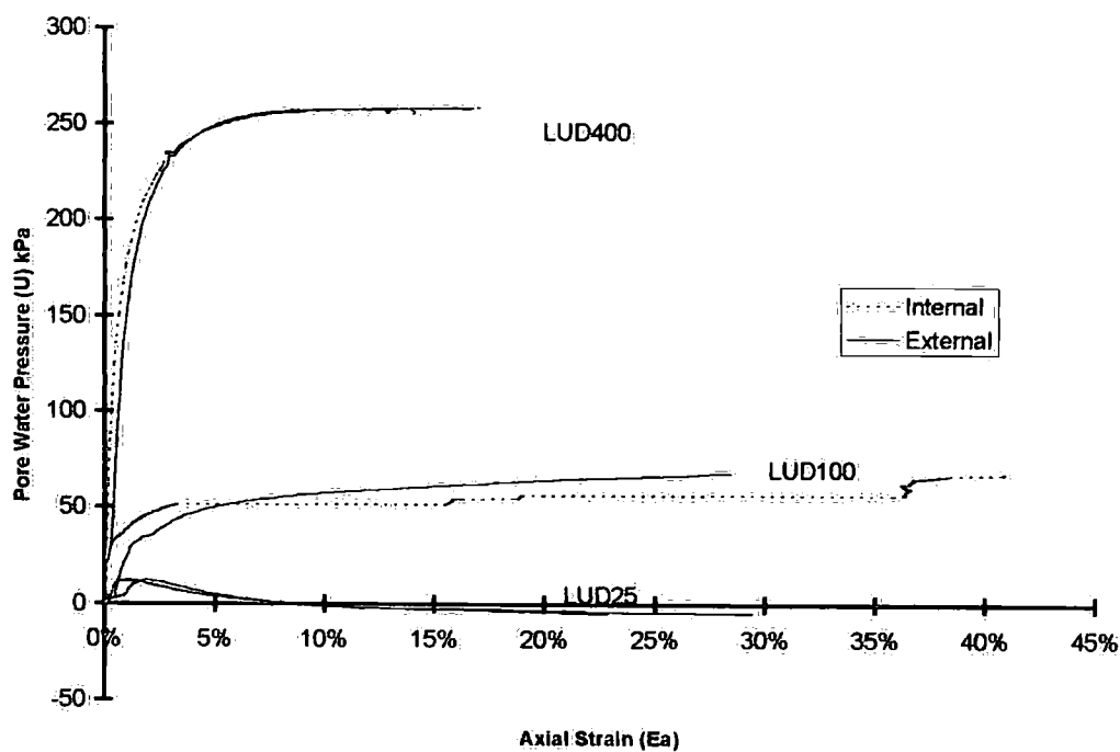
Figure 5-26b Comparison of axial strain measurement against change in pore water pressure for LUD test specimens fitted with internal strain measuring devices
