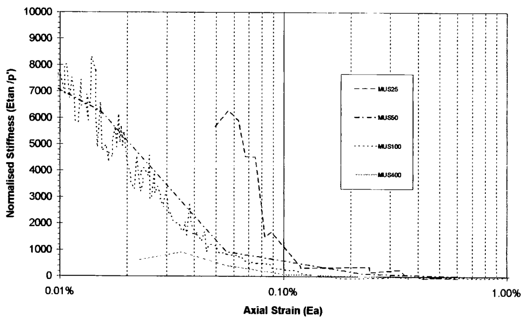
Figure 6-38 Normalised stiffness plots for MUS tests fitted with internal strain measuring devices
