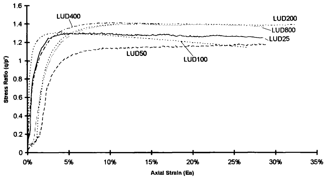
Figure 5-28 Stress ratio against strain plots for LUD tests
