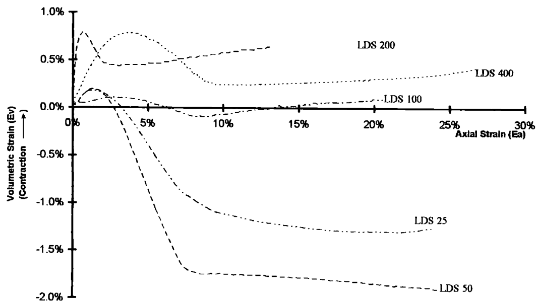
Figure 5.7a Volumetric strain versus axial strain plot for LDS tests up to 400kPa confining pressure
