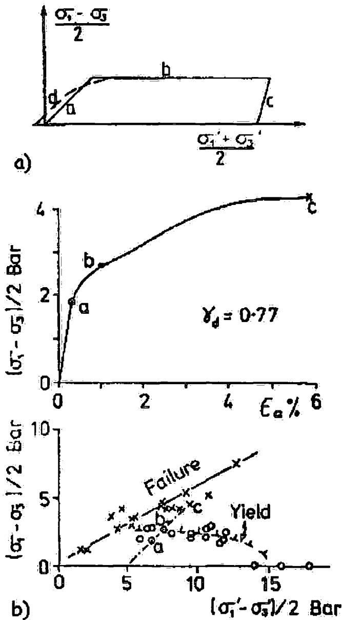
Figure 5-13 a) Sangrey (1972) postulated yield surface from Vaughan (1985) Fig. 7 b) Yield surface for altered volcanic agglomerates by Uriel and Serrano (1972) from Vaughan (1985) Fig. 8
