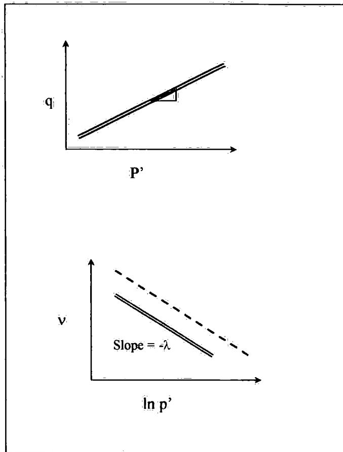
Figure 2-3 Critical State lines for Triaxial tests in a) q' - p' space, b) v - \ln p' space
