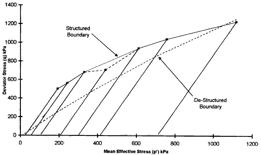
Figure 6-11 Effective stress path plots for MDS tests
