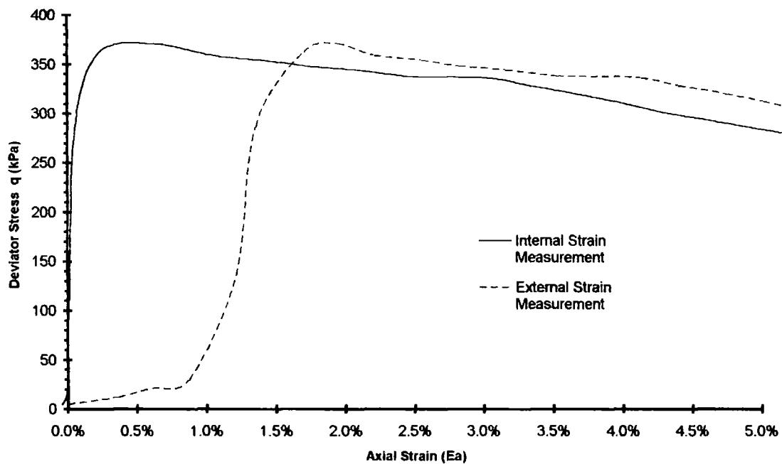
Figure 6-32 The difference between internal and external strain measurement when considering small strains (<1.0%) in LUS50
