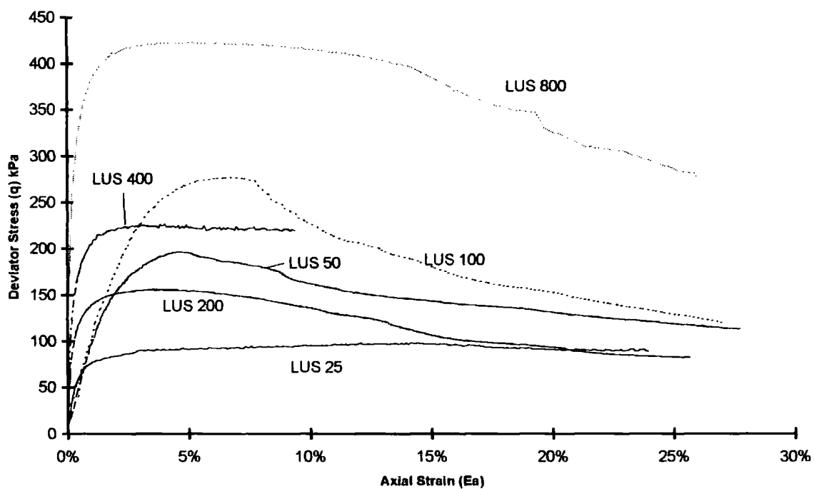
Figure 5-30a Stress against strain plot for LUS '25-800' tests using external measuring devices
