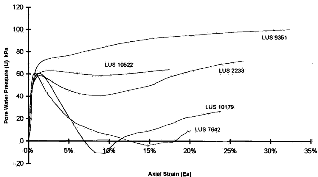
Figure 5-56 Changes in pore water pressure versus axial strain for BS406 tests at 125kPa confining pressure
