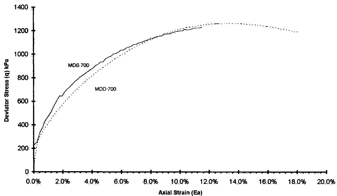
Figure 6-25c Comparison of stress-strain curves fly ash mortar specimen tested at 700kPa confining pressure
