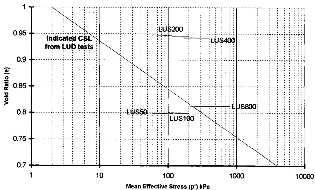
Figure 5-35 Void ratio changes against effective mean stress plot for LUS '25-800' tests
