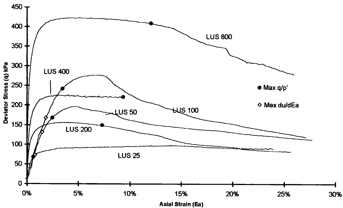
Figure 5-34 Relative position of the maximum points for LUS '25-800' test plotted stress-strain curves
