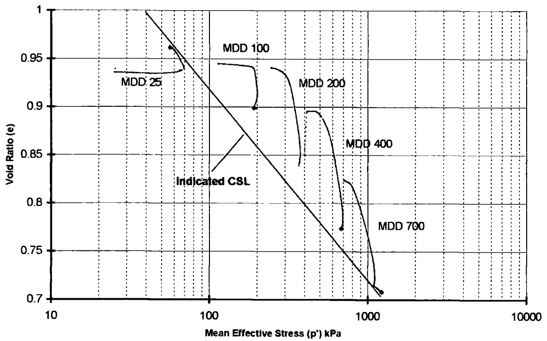
Figure 6.8 Void ratio against mean effective stress for MDD tests
