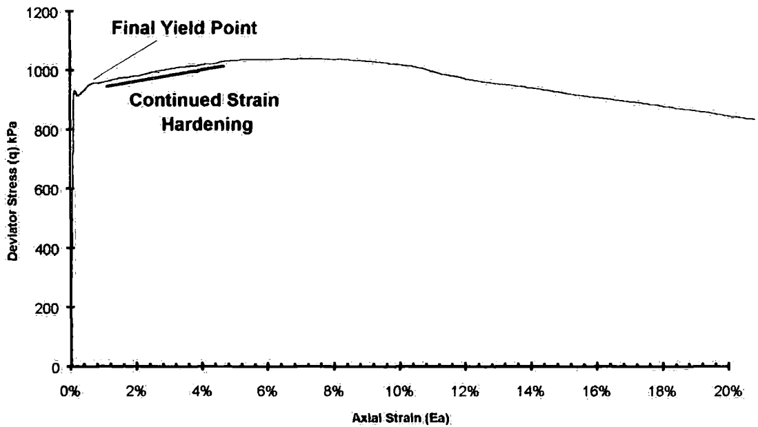
Figure 6-20a Stress-strain plot for MDS400 showing strain development after final bond yielding
