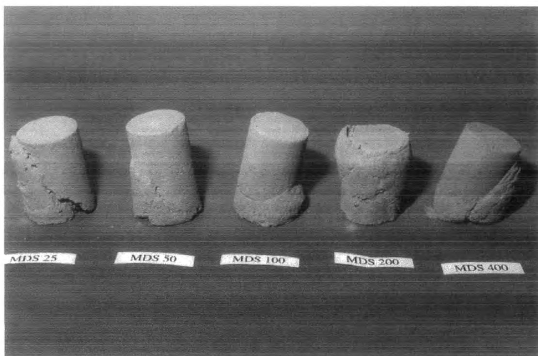
Plate 6-3 Structured fly ash mortar specimens after under going drained triaxial compression
