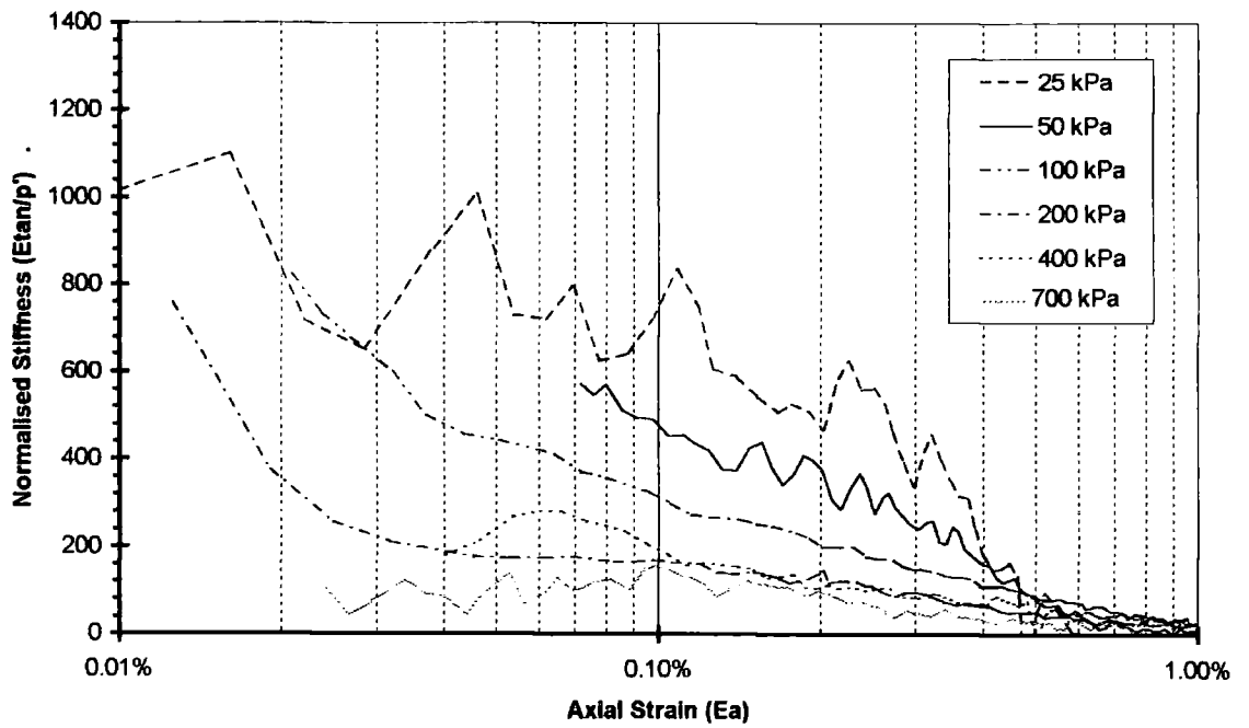
Figure 6.7 Stiffness normalised with respect to mean effective stress against strain for MDD tests
