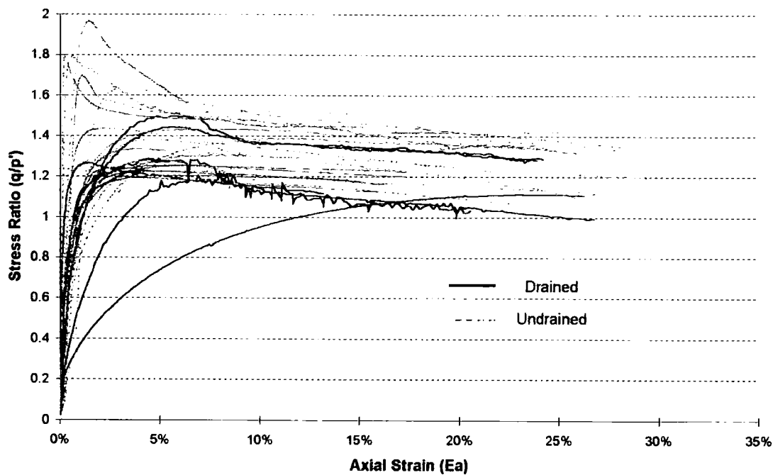
Figure 5-69 Stress ratio against strain plots for all undisturbed lagoon fly ash specimen
