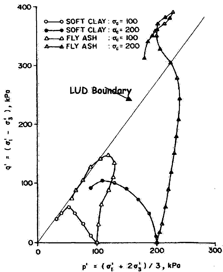
Figure 5-79 Stress paths from undrained tests on Fly ash from a disposal dump (after Indraratna et al 1990) compared to the LUD boundary.
