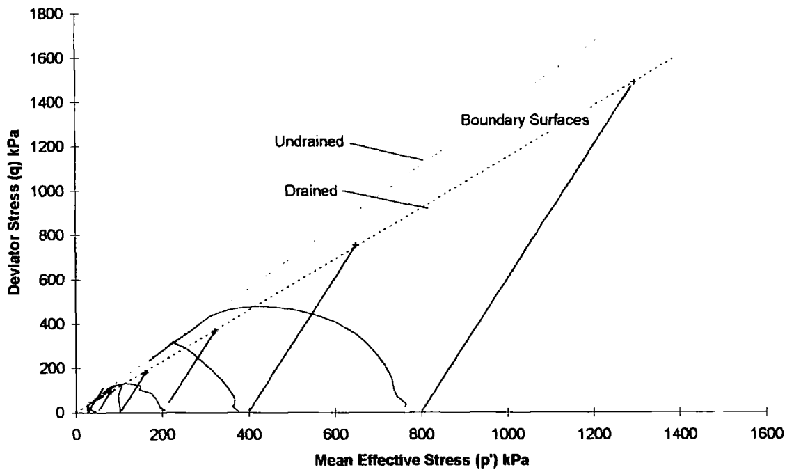
Figure 5-67 Stress paths and boundaries for drained and undrained tests on remoulded lagoon fly ash
