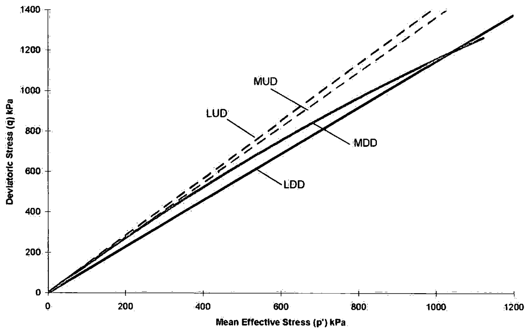
Figure 6-44 Boundary surfaces for fly ash specimens under drained triaxial conditions
