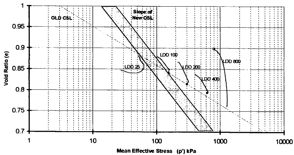
Figure 5-72 Comparison of new CSL to LDD tests
