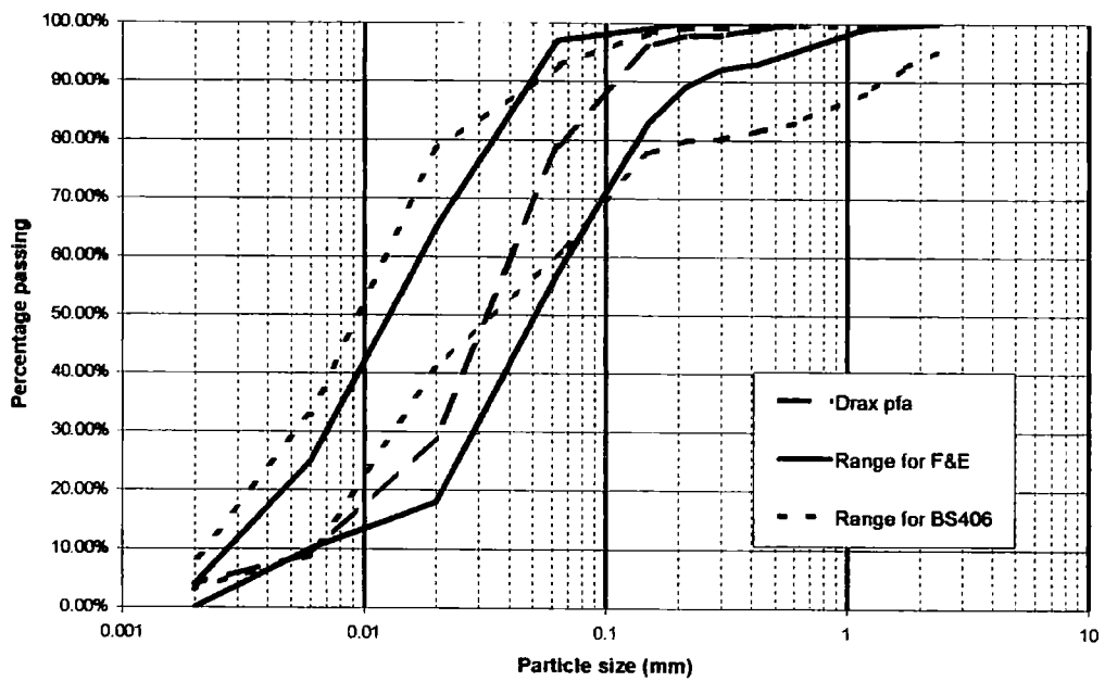
Figure 3-9 Typical ranges of fly ash particle distributions from different fly ash sources
