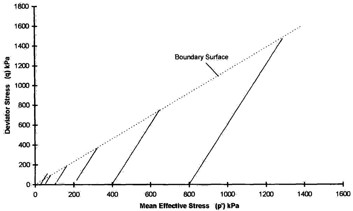
Figure 5.3 Effective stress paths for the LDD tests
