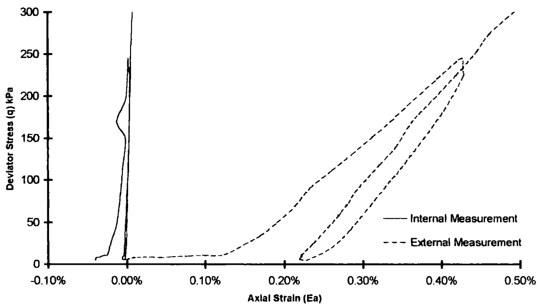
Figure 6-33 The difference between internal and external strain measurements of a small unload/reload cycle at the beginning of LUS100
