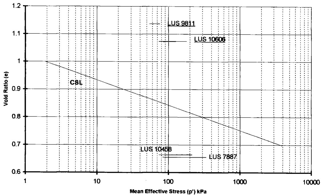
Figure 5-53 Void ratio against mean effective stress plot for BS406 tests at 75kPa confining pressure
