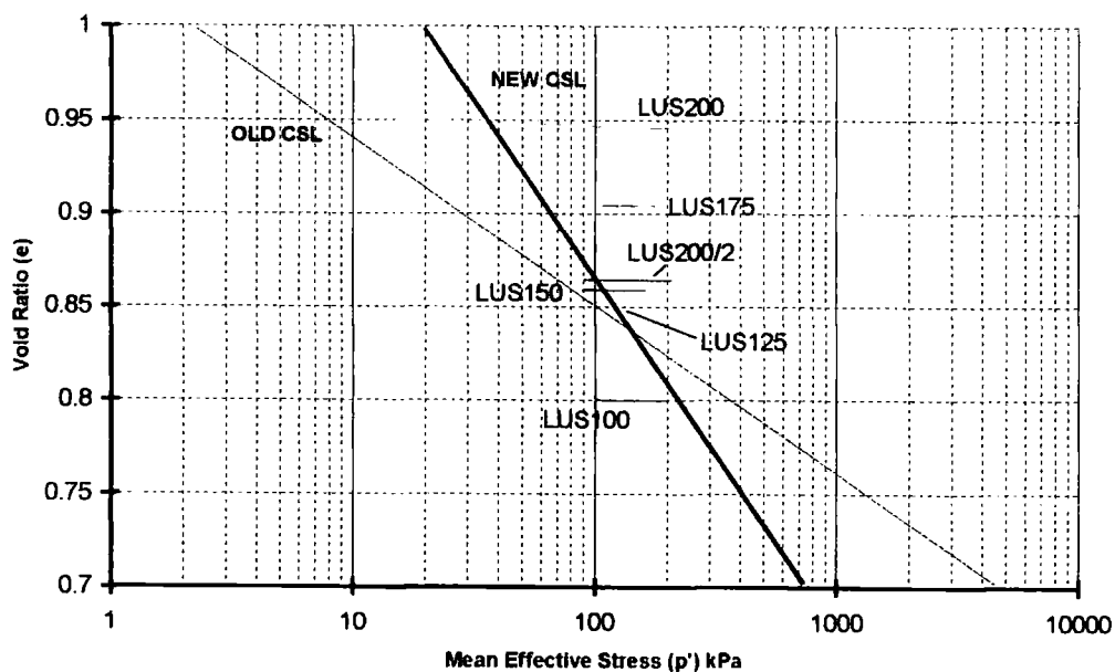
Figure 5-75b Comparison of new CSL to LUS tests '100-200'
