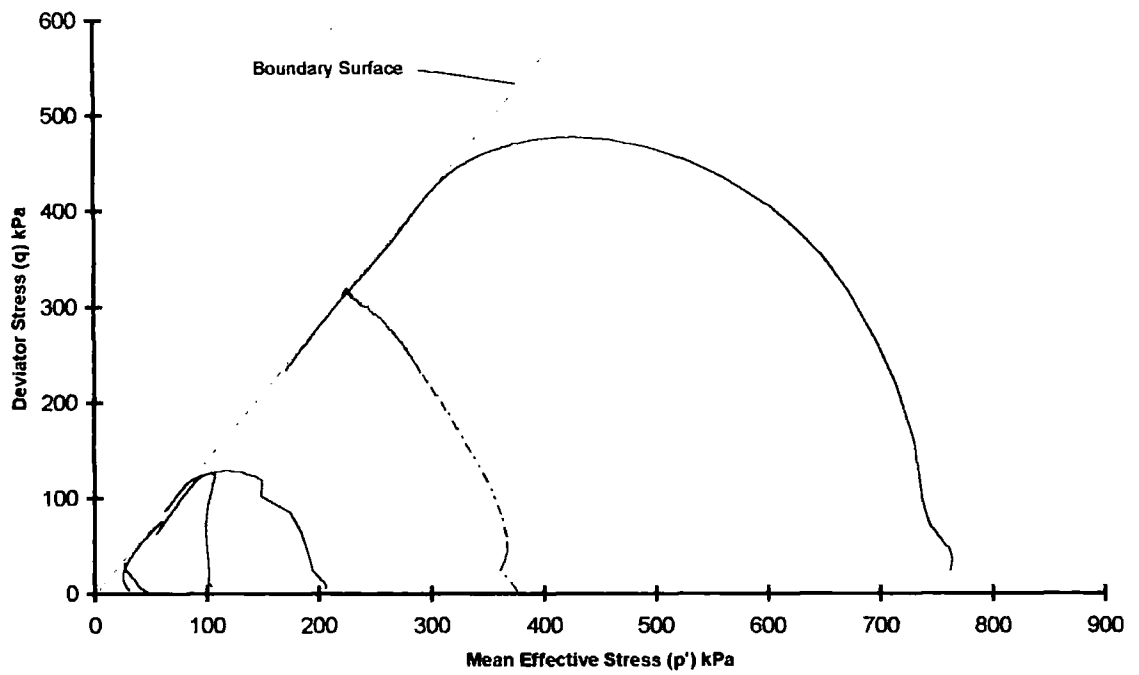
Figure 5-27 Effective stress paths for LUD tests
