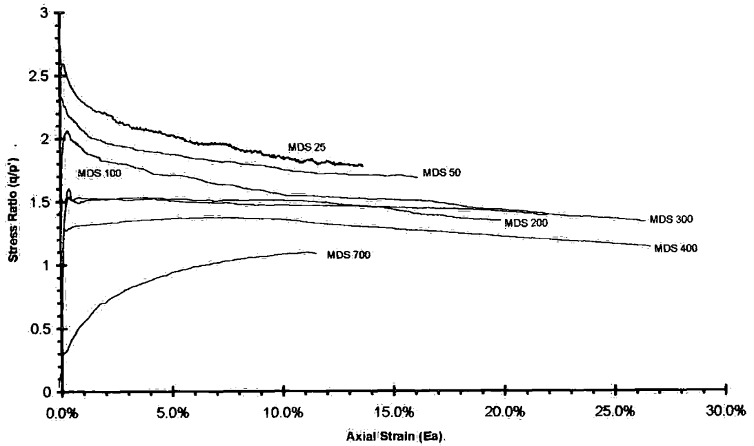
Figure 6-21 Stress ratio against strain plots for MDS tests
