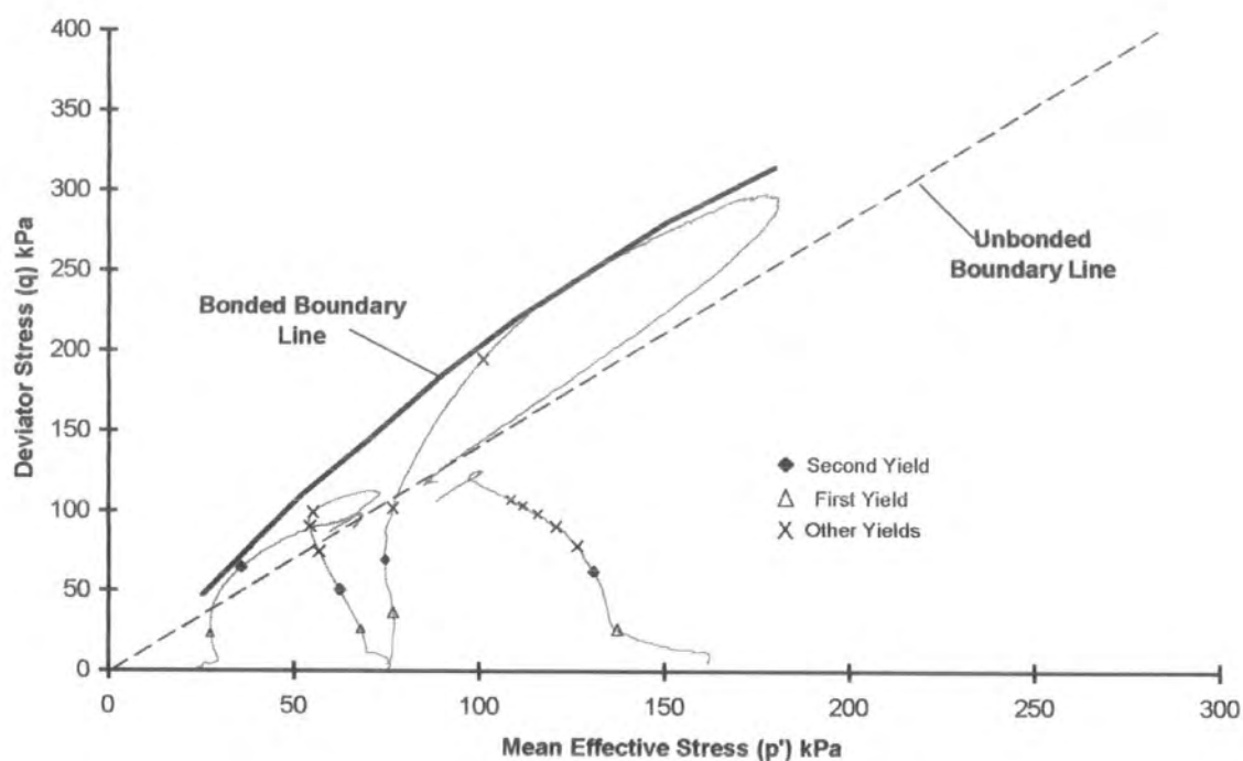
Figure 5-64 Yields plotted in stress space for undrained tests on lagoon fly ash
