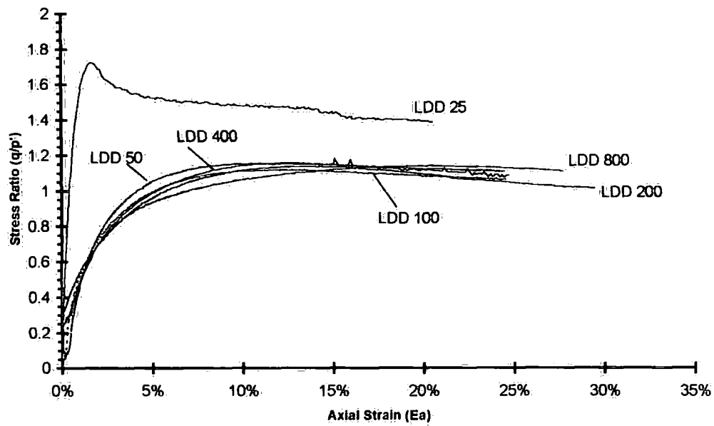
Figure 5.4 Stress ratio against strain plot for LDD tests
