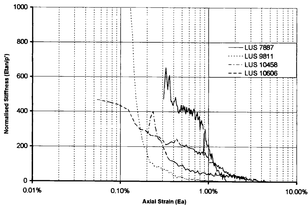
Figure 5-54 Normalised stiffness against strain for BS406 tests at 75kPa confining pressure
