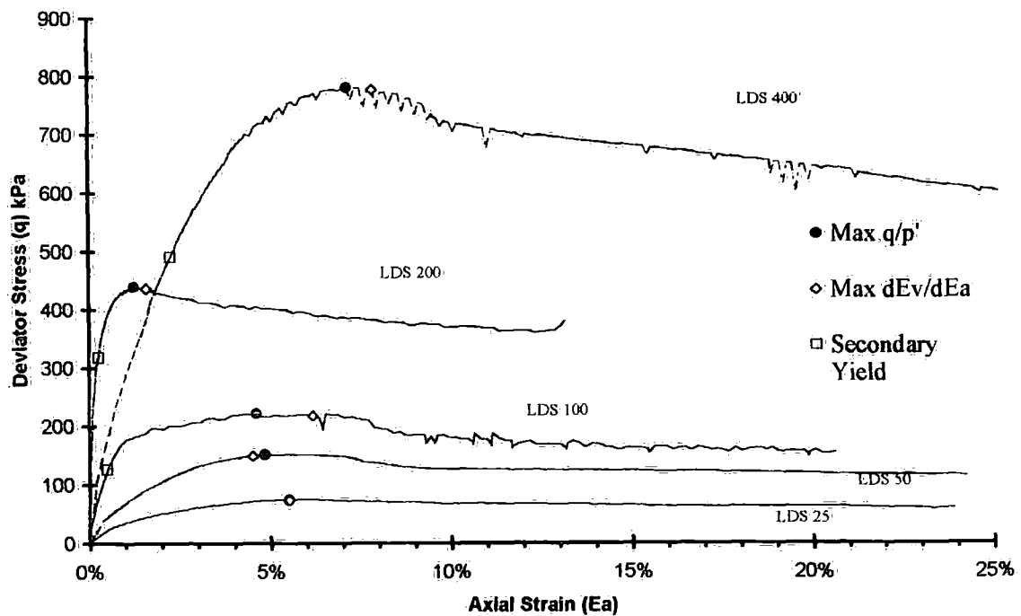
Figure 5.11 Relative position of (q/p')_{max} and (dE_v/dE_a)_{max} on stress-strain curves for LDS tests
