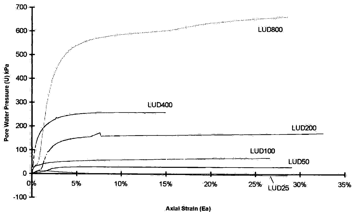
Figure 5-26a Change in pore water pressure versus axial strain plot for LUD tests
