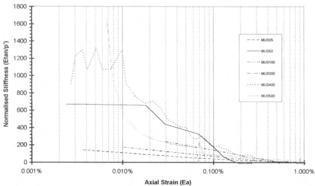
Figure 6-30 Normalised stiffness against strain plots for MUD tests
