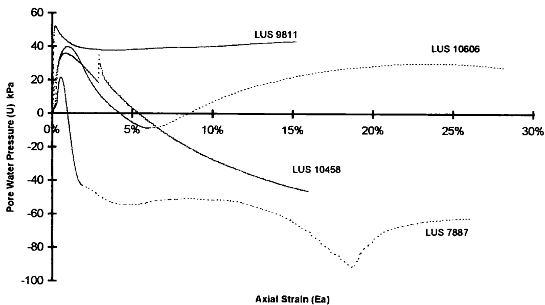
Figure 5-49 Changes in pore water pressure versus axial strain for BS406 tests at 75kPa confining pressure
