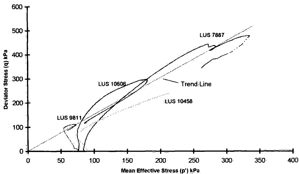
Figure 5-50 Effective stress paths for BS406 tests at 75kPa confining pressure
