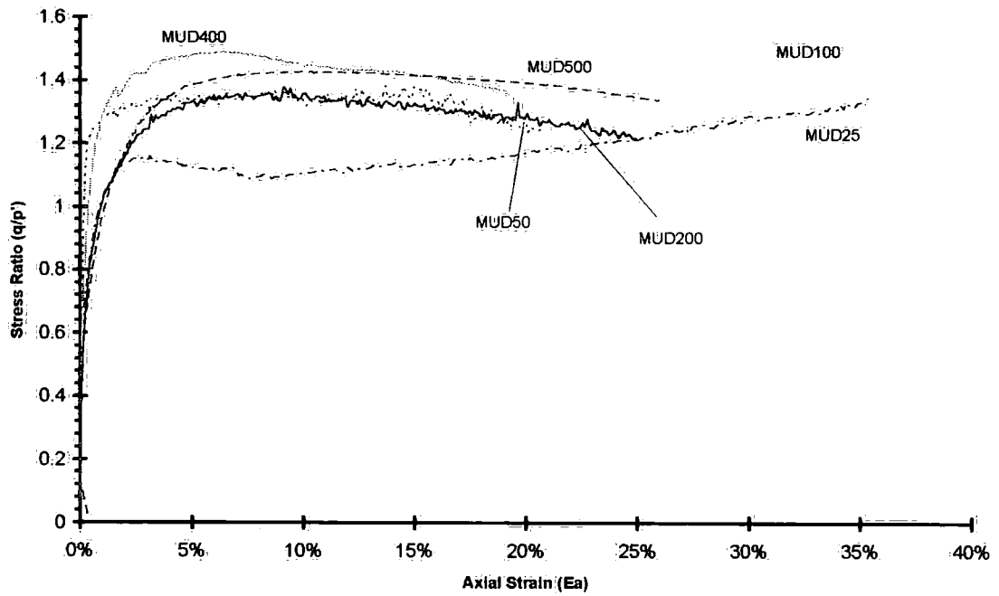
Figure 6-29 Stress ratio against strain plots for MUD tests
