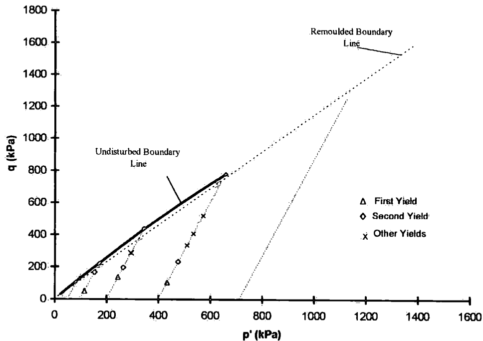
Figure 5.20 First and second yield points plotted in stress space with the boundary surfaces for LDD and LDS tests
