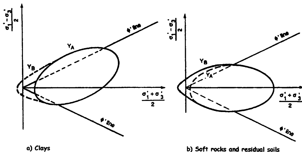
Figure 5-77 Yield curves for structured soils (after Leroueil & Vaughan 1990)
