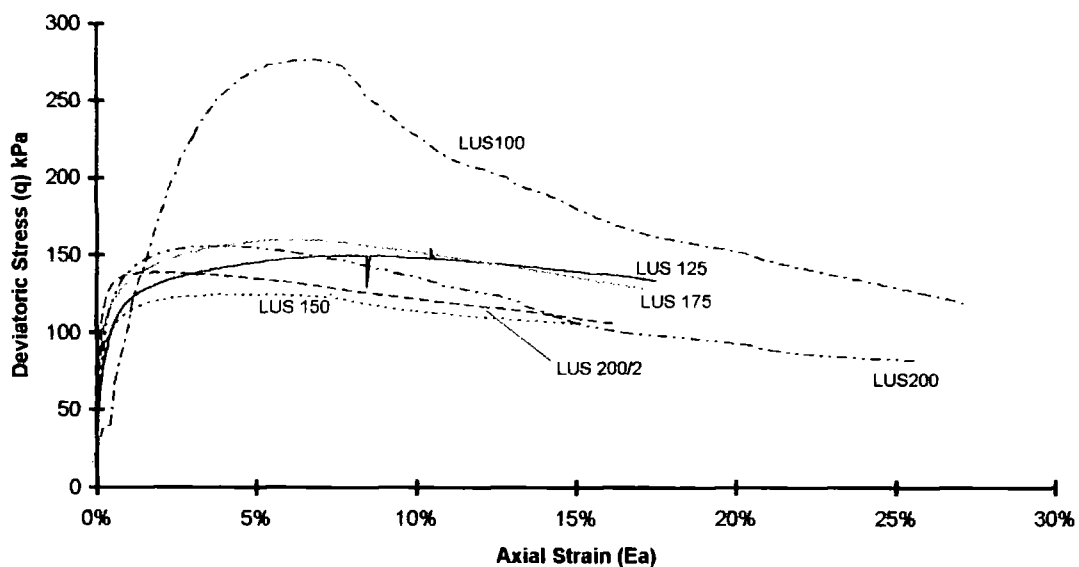
Figure 5-38 Stress against strain plot for LUS '100-200' tests, with LUS100 and LUS200
