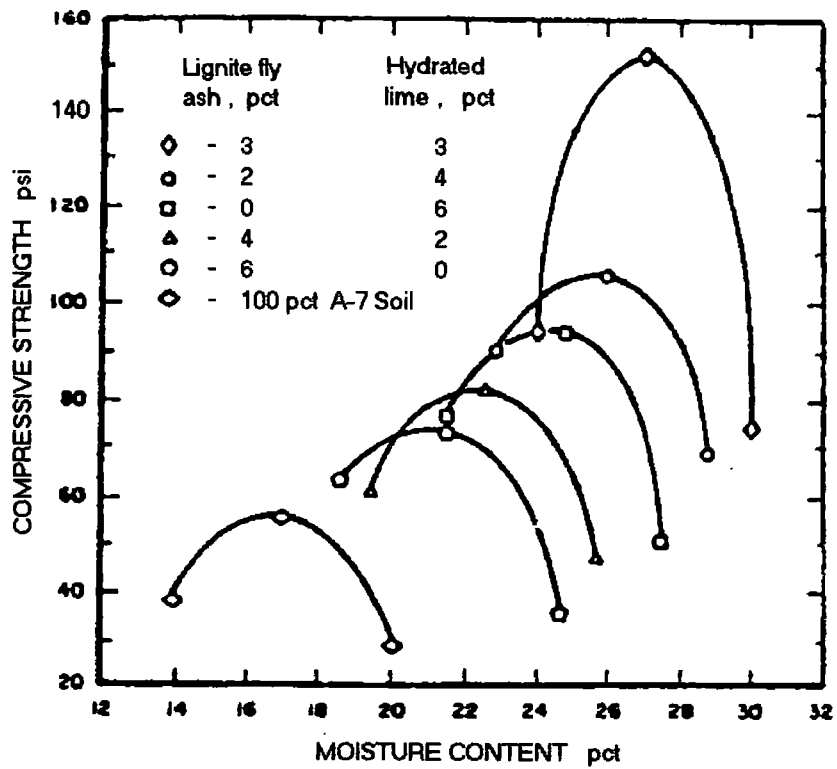
Figure 2-4 Compressive strength versus moisture content after 7 days moist curing (Manz 1984)
