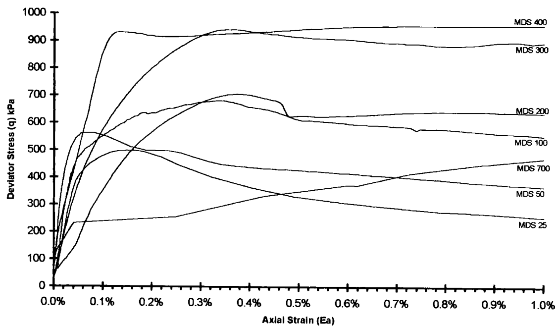
Figure 6.9b Stress-strain plot for MDS tests for the first percent axial strain
