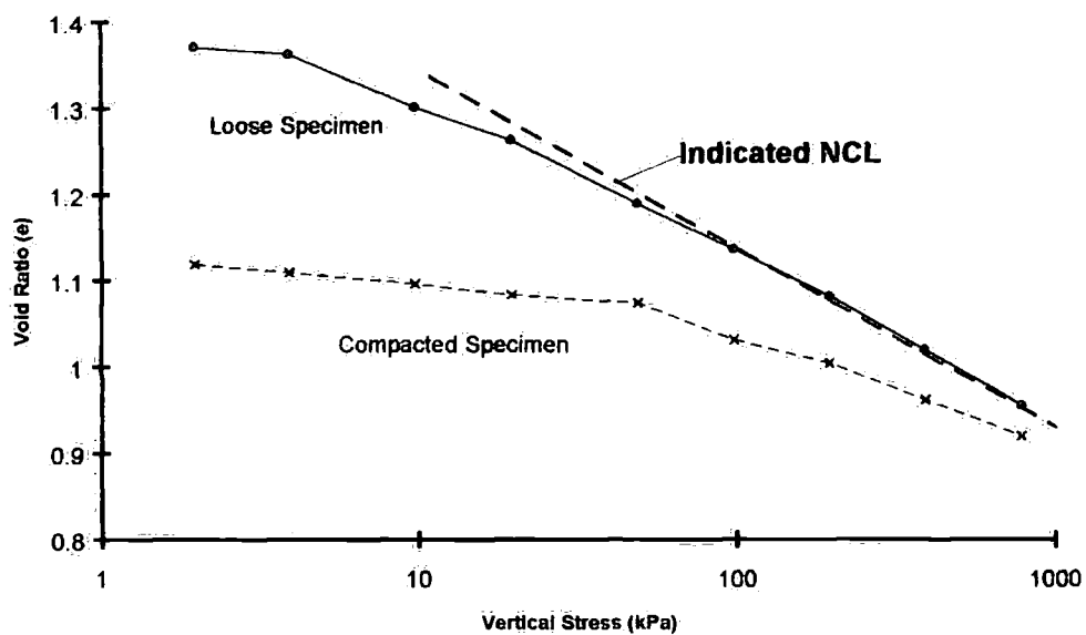
Figure 5-65 Consolidation curves for specimens of remoulded lagoon fly ash
