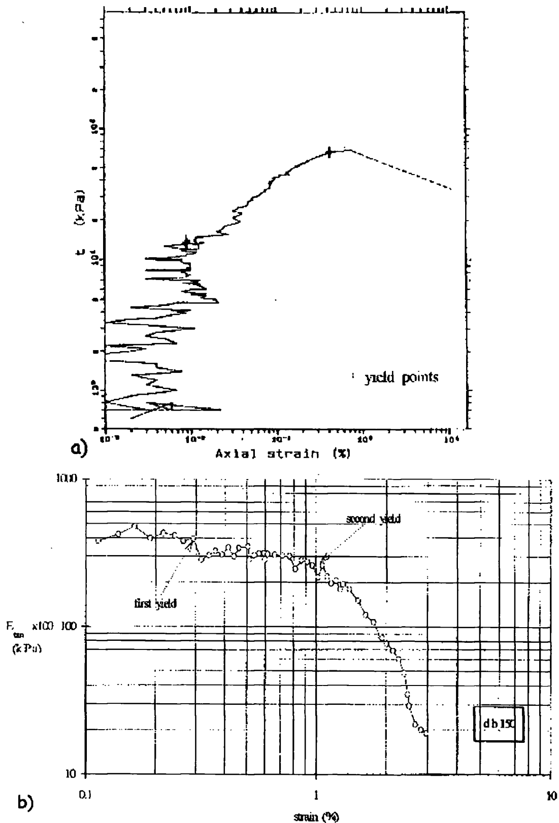
Figure 5.15 Definition of two yields by a) Vaughan (after Vaughan 1985) & b) Malandraki (after Malandraki 1994)
