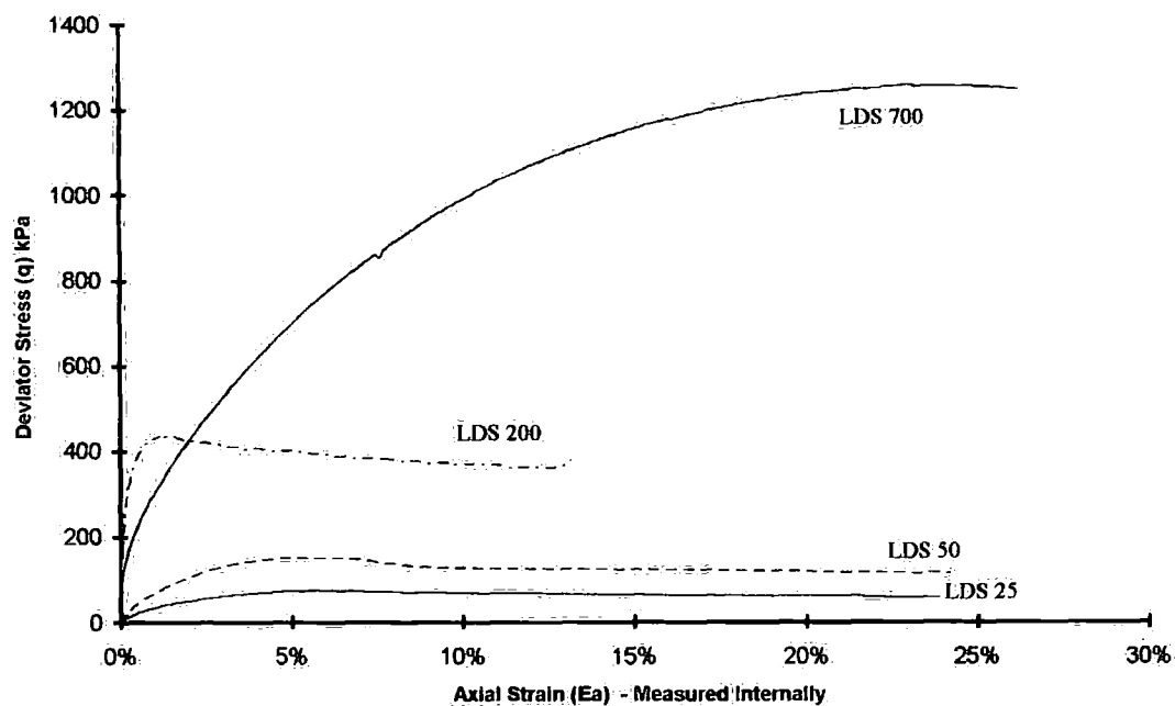
Figure 5.6a Stress against strain plot for LDS tests using direct strain measuring devices
