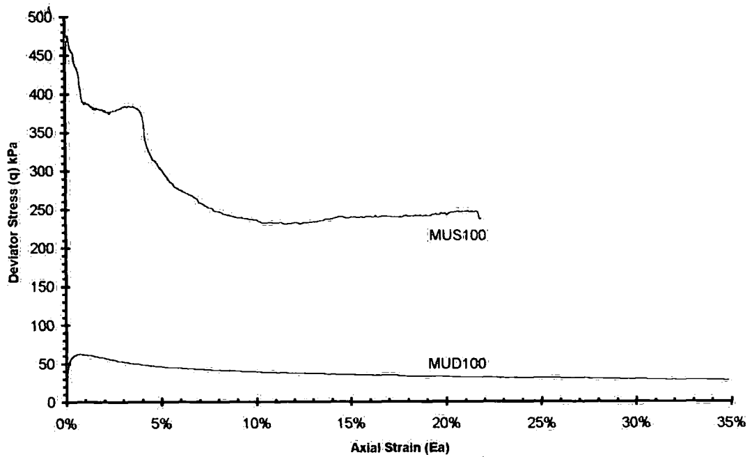
Figure 6-40 Comparison between structured and de-structured stress-strain curves for specimen tested at 100kPa confining pressure
