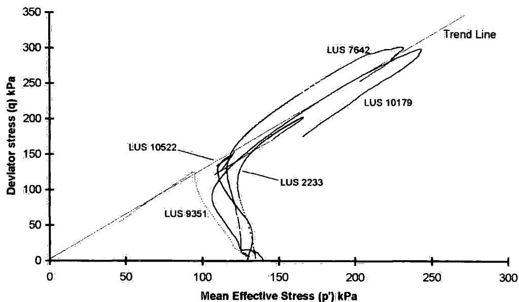
Figure 5-57 Effective stress paths for BS406 tests at 125kPa confining pressure
