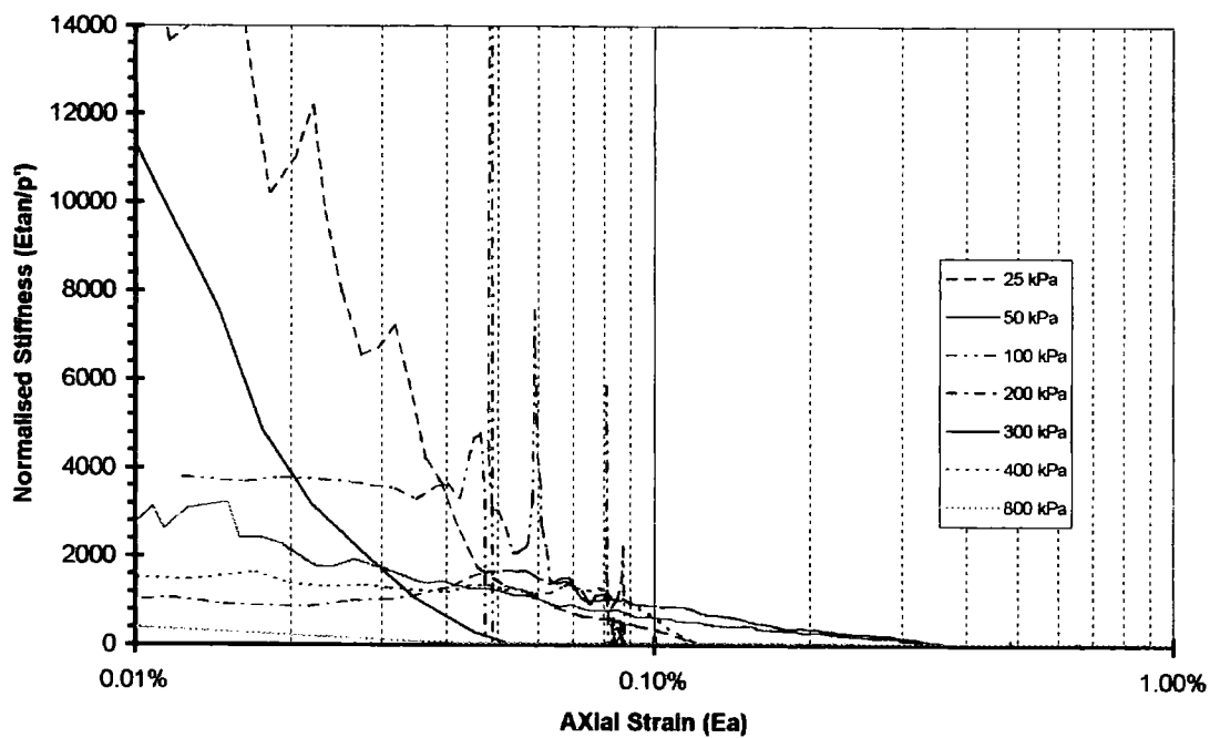
Figure 6-23 Normalised stress against strain plots for MDS tests
