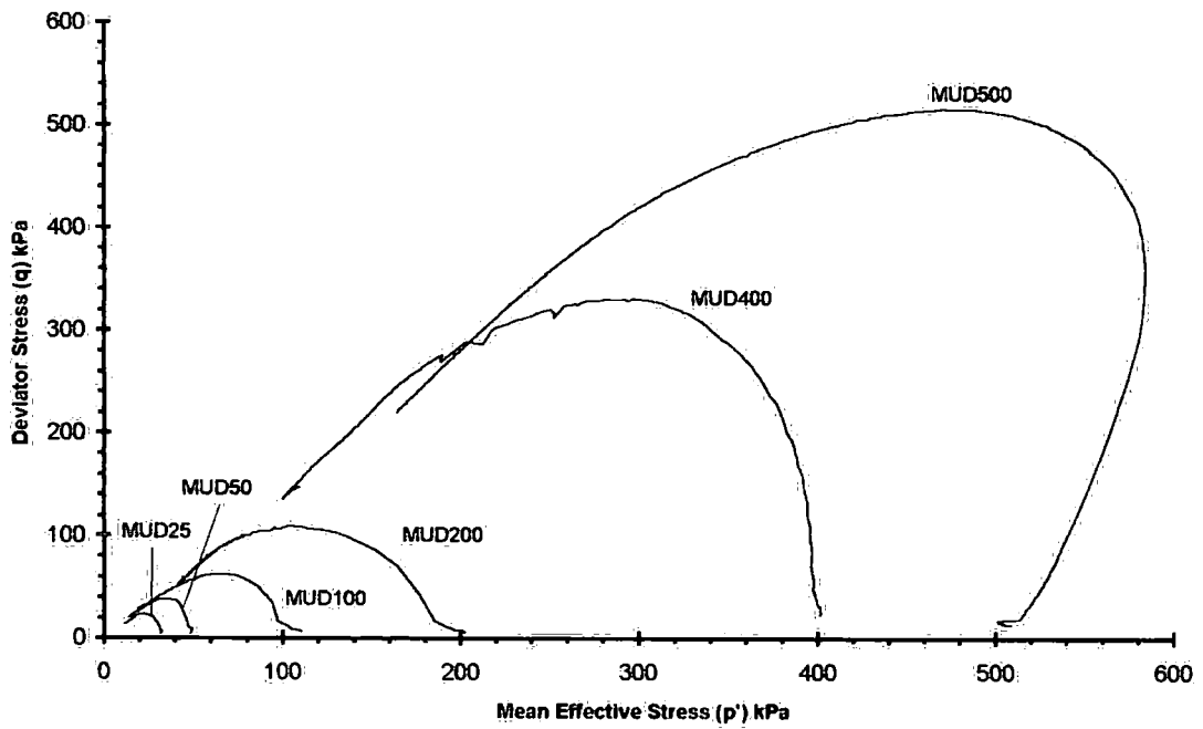
Figure 6-28 Effective stress paths plots for MUD tests in stress space
