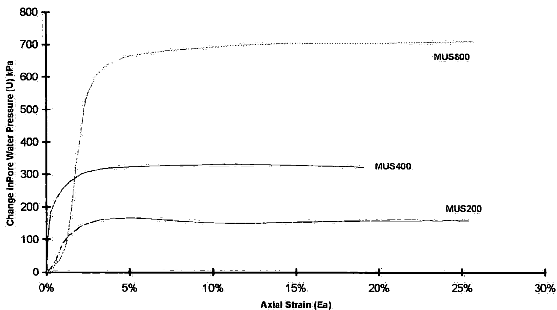
Figure 6-35 Changes in pore water pressure against strain plot for tests at 200kPa confining pressure and above
