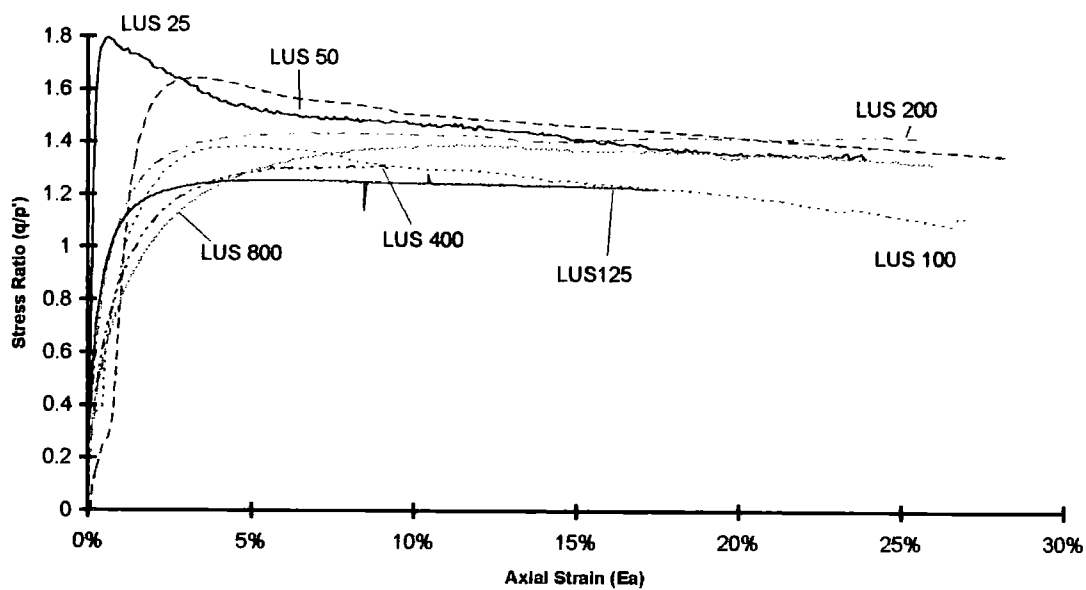
Figure 5-33 Stress ratio against strain plot for LUS '25-800' tests
