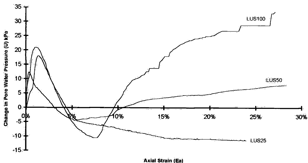
Figure 5-31a. Changes in pore water pressure versus axial strain for LUS '25-800' tests at 100kPa confining pressure and below.
