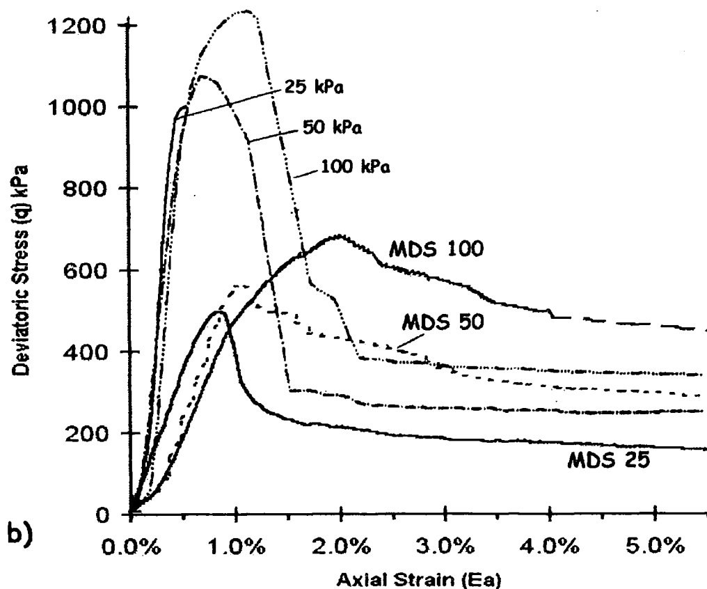
Figure 6-47 Comparison of a) LDS tests and b) MDS tests at equivalent confining pressures to the stress-strain plots for fly ash specimens of dry fly ash from Blyth power station (compacted to 95% dry of its optimum moisture content and allowed to cure for 2 months (Yang 1992)).
