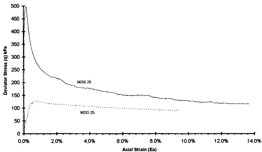
Figure 6-25a. Comparison of stress-strain curves for structured and de-structured fly ash mortar specimen tested at 25kPa confining pressure
