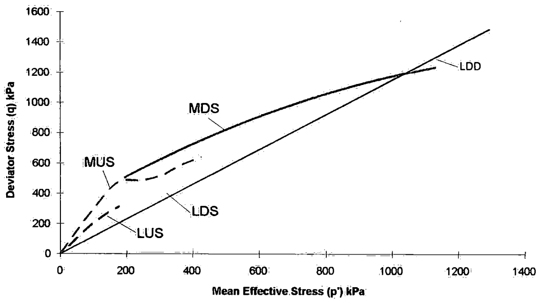
Figure 6-45 Boundary surfaces for bonded specimen
