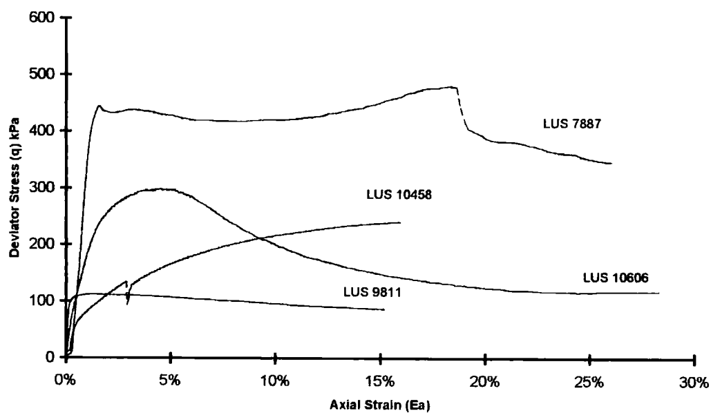
Figure 5-48 Stress against strain for BS406 tests at 75kPa confining pressure
