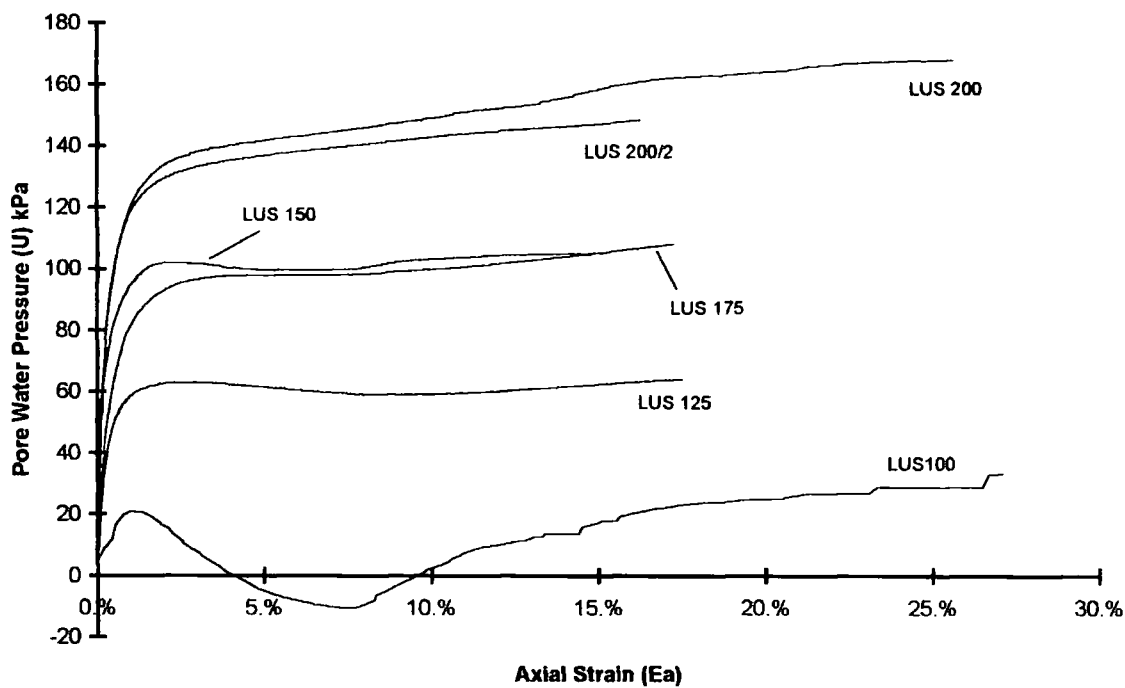
Figure 5-39 Changes in pore water pressure against axial strain for LUS '100-200' tests with LUS100 and LUS200 for comparison.
