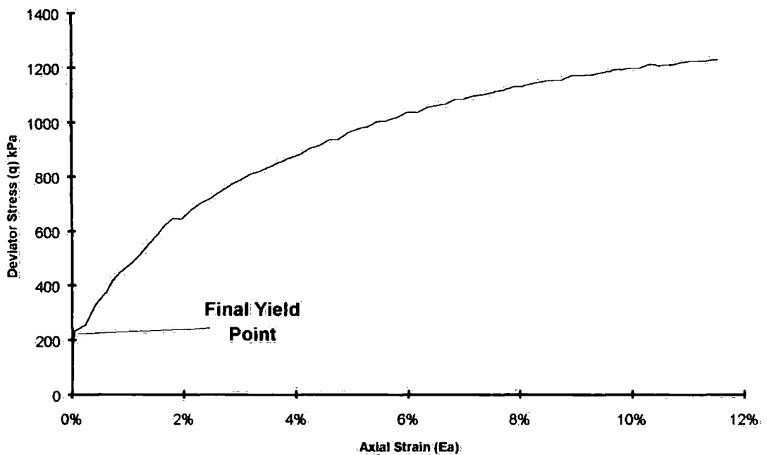
Figure 6-20b Stress-strain plot for MDS700 showing final bond yielding occurring at low stresses
