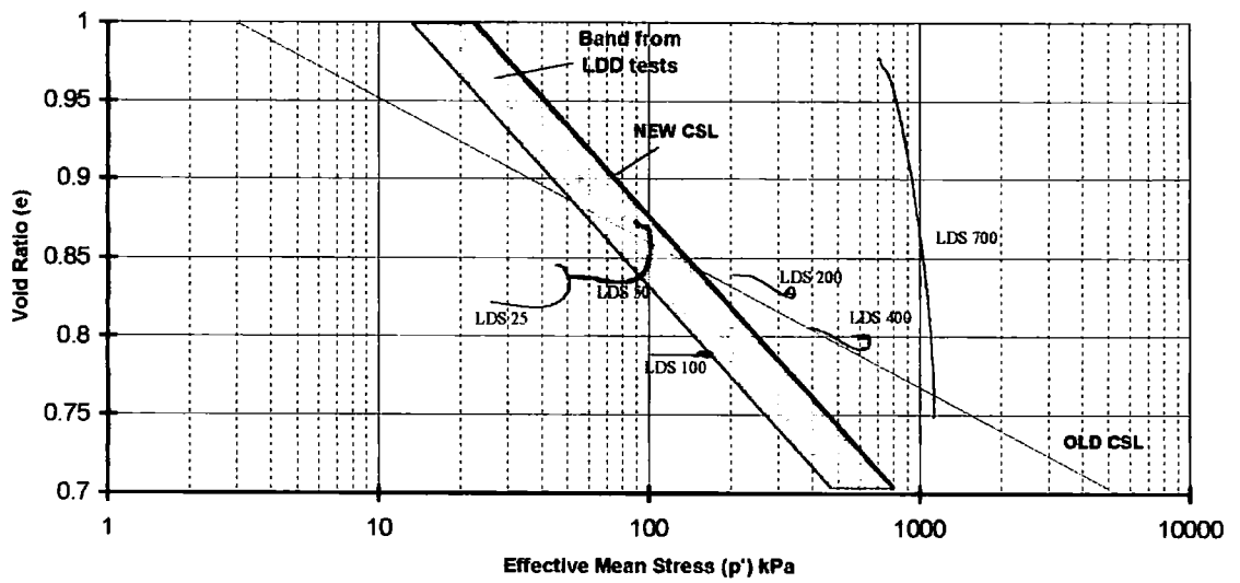
Figure 5-73 Comparison of new CSL to LDS tests
