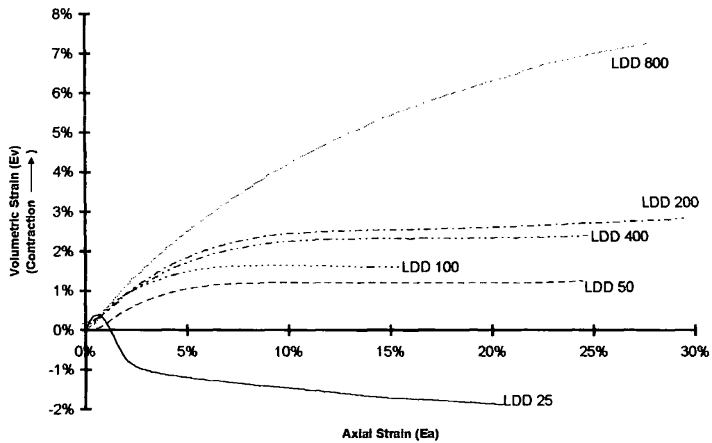
Figure 5.2 Volumetric Strain versus Axial Strain plot for LDD tests
