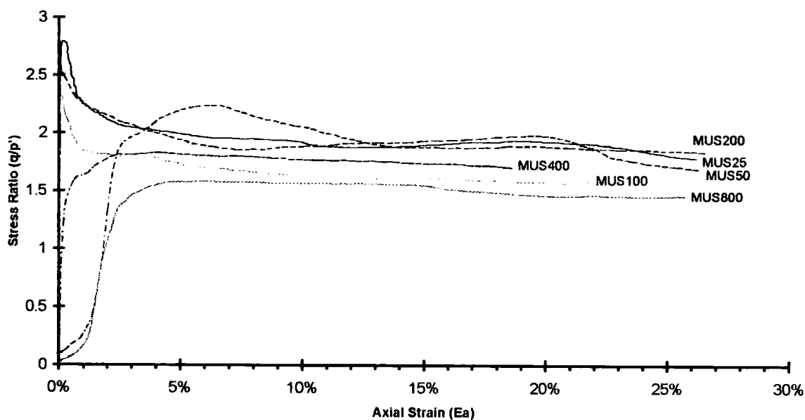
Figure 6-37 stress ratio against strain plots for MUS tests
