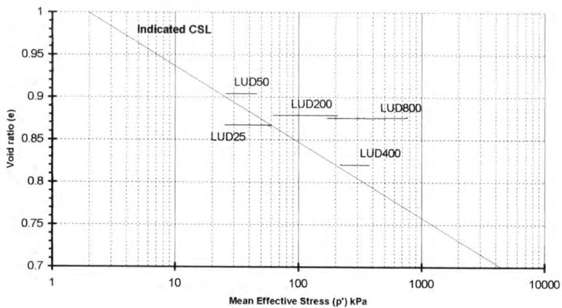
Figure 5-29 Void ratio changes against mean effective stress plot for LUD tests
