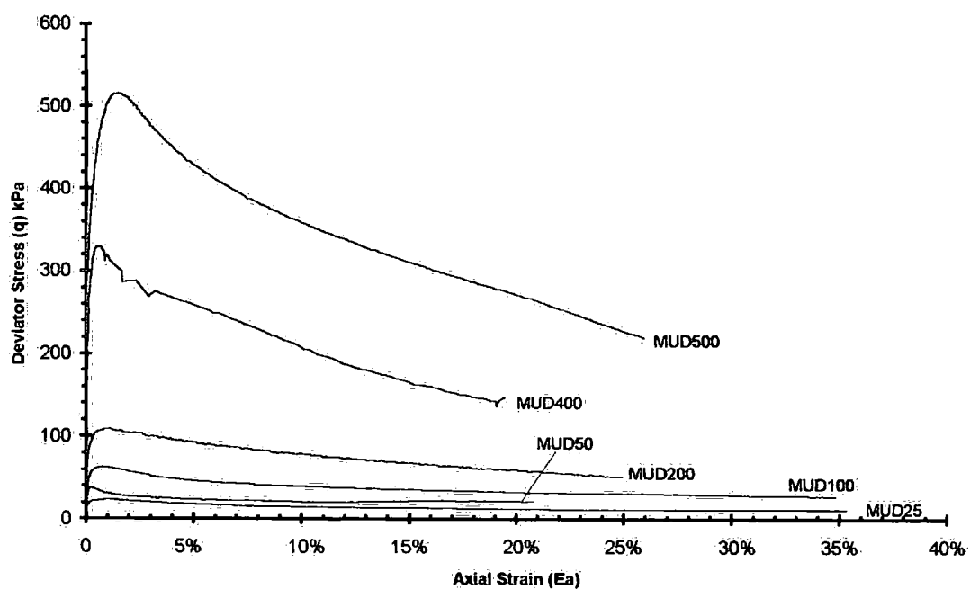
Figure 6-26 Stress against strain plots for MUD tests
