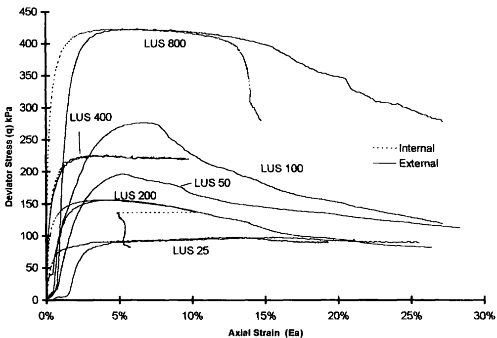
Figure 5-30b Stress against strain plots for LUS '25-800' tests showing the difference in strain measurement between internal and external devices
