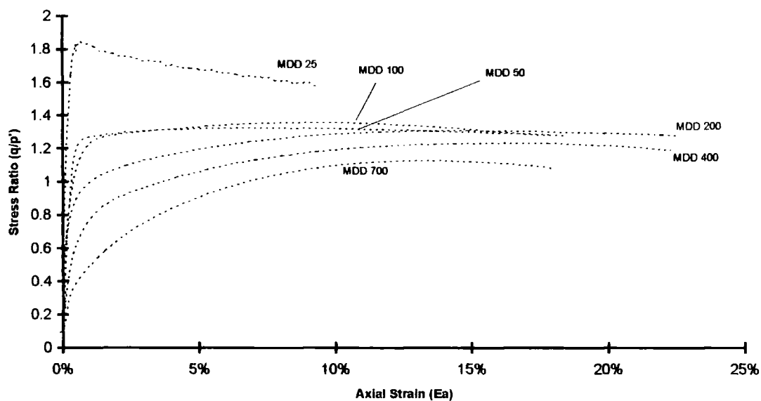
Figure 6.6 Stress ratio against strain for MDD tests
