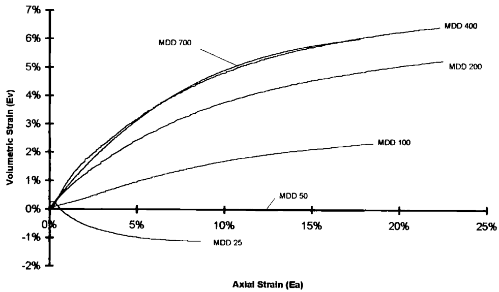
Figure 6-4 Volumetric strain versus axial strain for MDD tests
