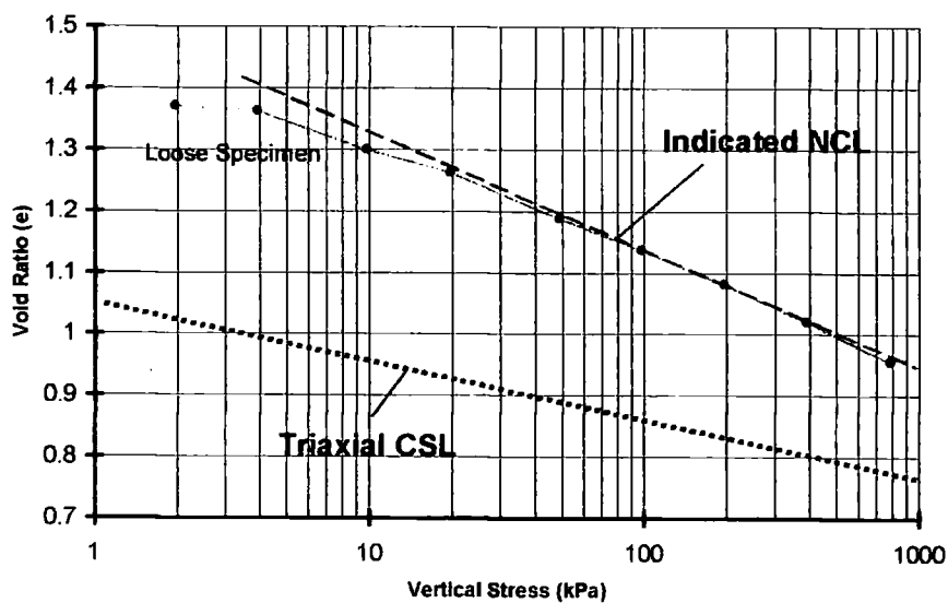
Figure 5-71 Comparison of the inferred critical state line (triaxial) and one-dimensional consolidation line
