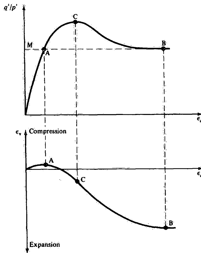
Figure 5.10 Typical relationship between stress ratio and volumetric strain for a drained triaxial test on dense sand (after Atkinson 1978)
