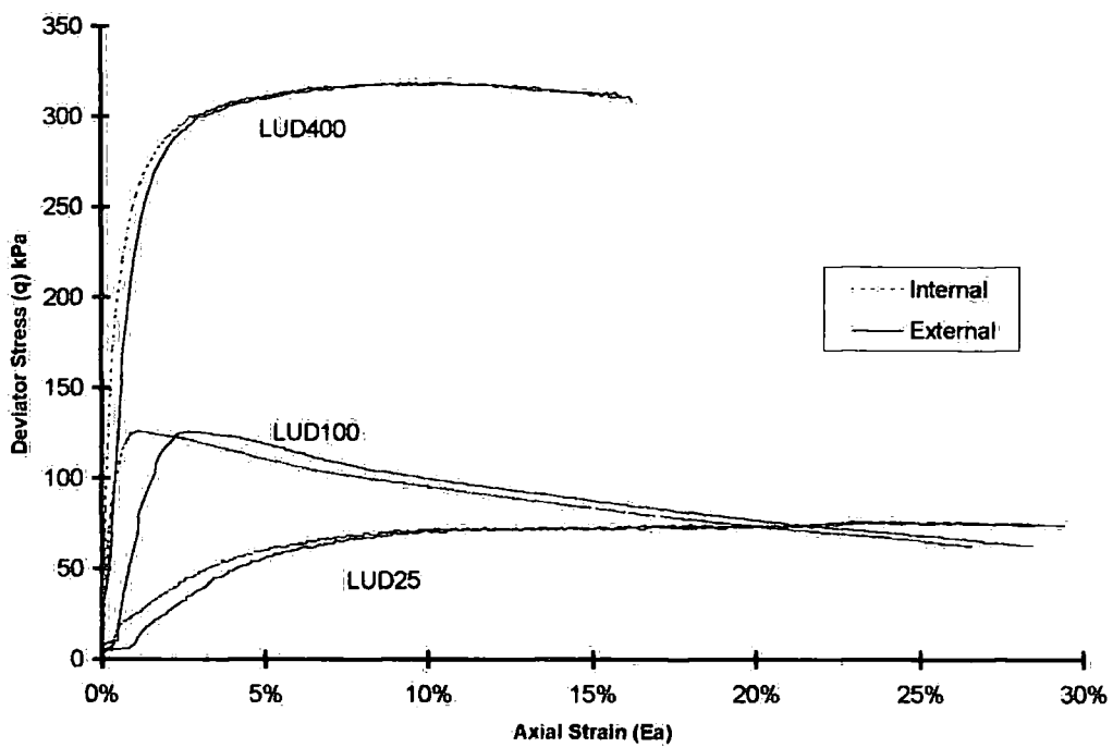
Figure 5-25b Comparison of axial strain measurement against stress for LUD test specimens fitted with internal strain measuring devices.
