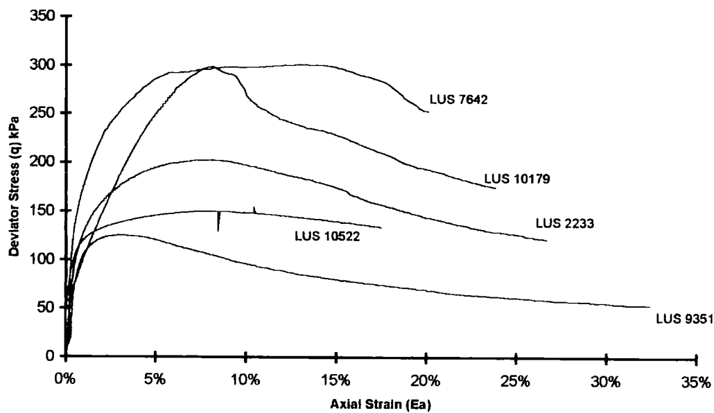
Figure 5-55 Stress against strain for BS406 tests at 125kPa confining pressure
