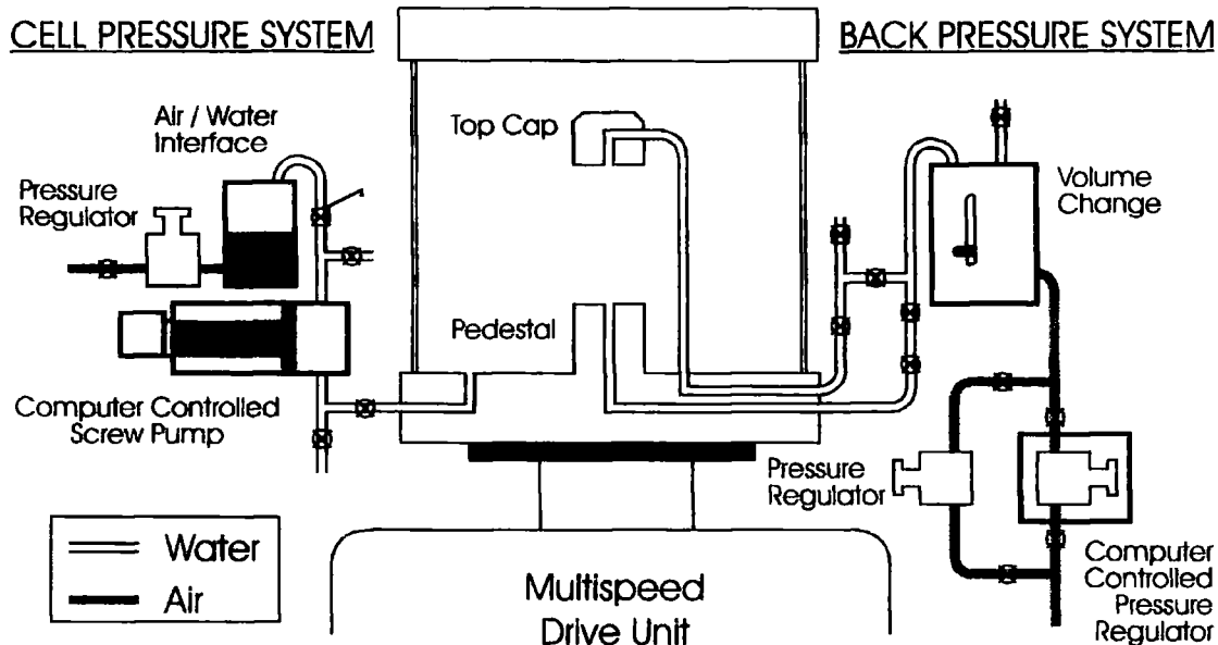
Figure 4-1 The insertion of computer controlled devices in to the Cell and Back pressure systems of the Wickham and Farrance machines.
