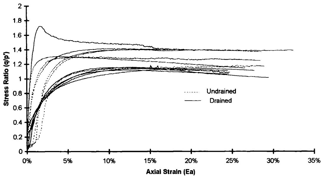
Figure 5-68 Stress ratio against strain plots for all remoulded lagoon fly ash specimen.
