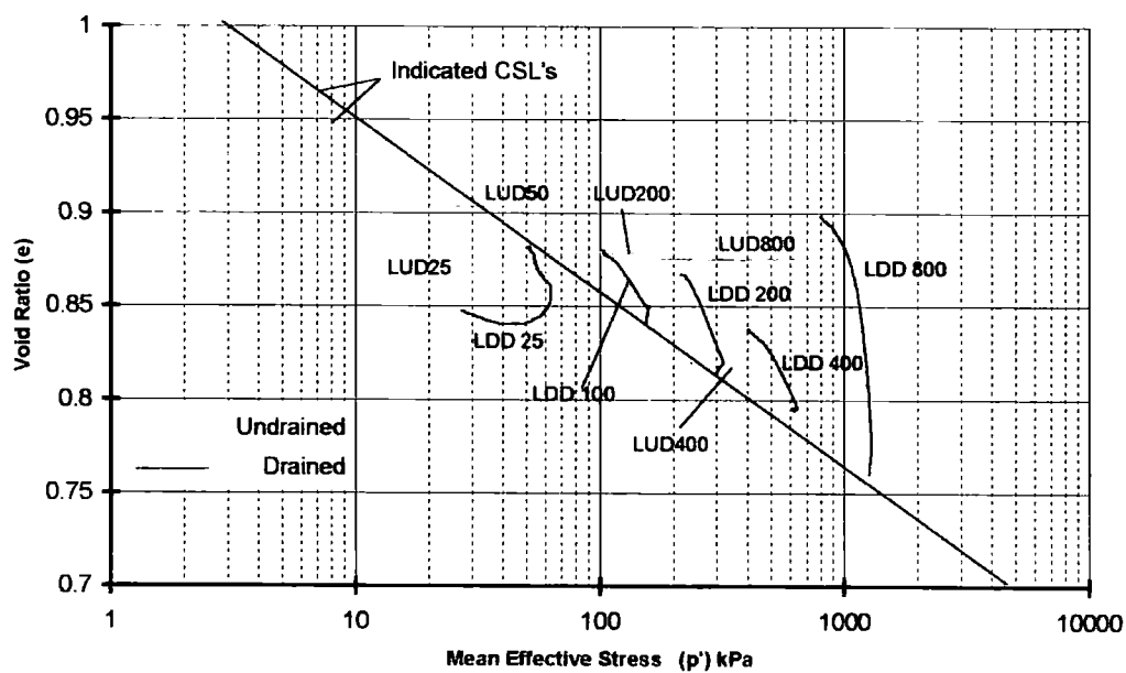
Figure 5-70 Paths of remoulded lagoon fly ash in void ratio - mean effective stress space
