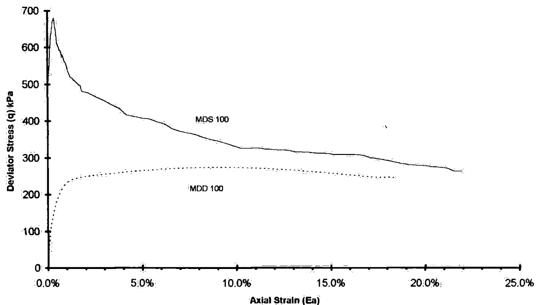
Figure 6-25b. Comparison of stress-strain curves fly ash mortar specimen tested at 100kPa confining pressure
