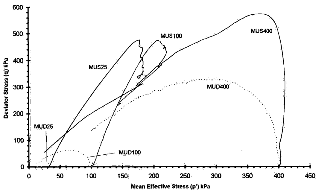
Figure 6-43 Comparison de-structured stress paths and structured stress paths for undrained triaxial tests on fly ash mortar specimen
