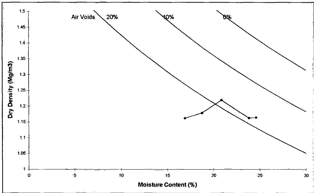
Figure 3-7 Compaction results on fly ash from BS 406
