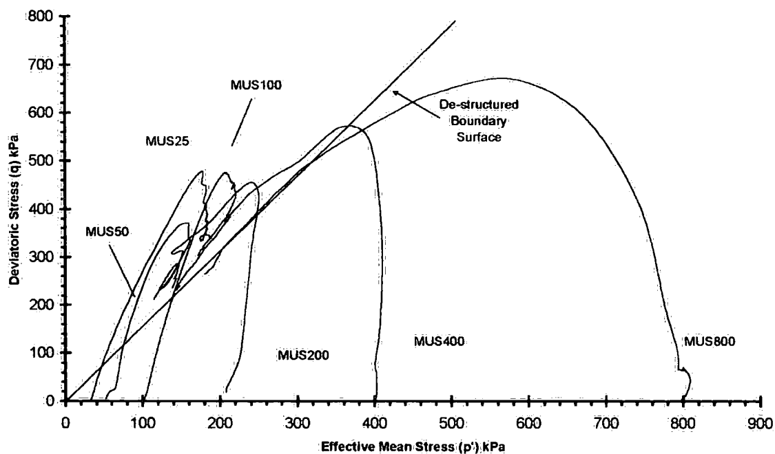
Figure 6-36 Effective stress paths for MUS tests
