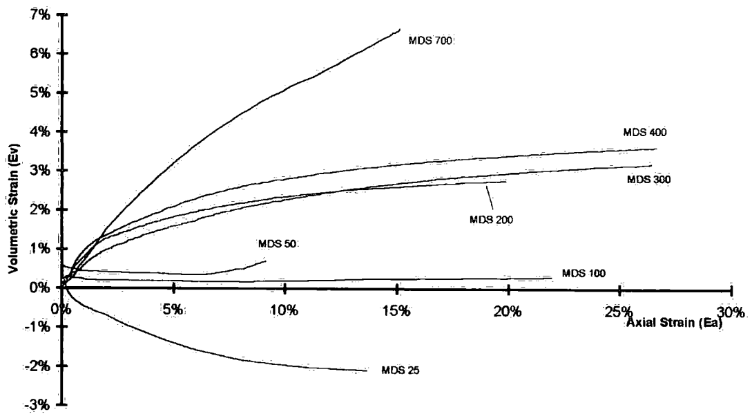
Figure 6-10 Volumetric strain versus axial strain plot for MDS tests
