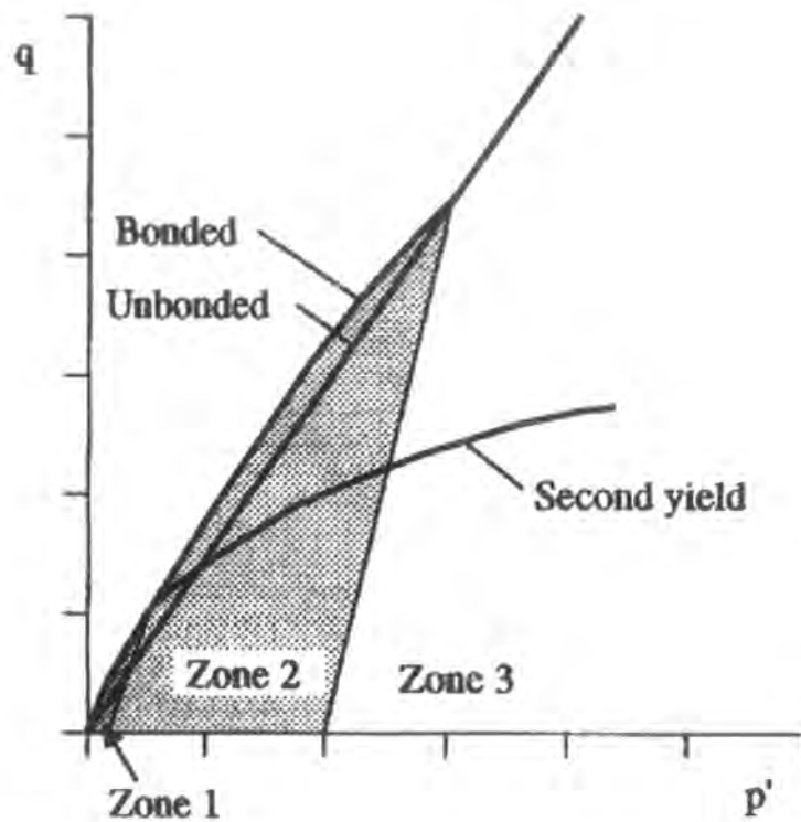
Figure 5.23 Idealised zones of behaviour for bonded soil (after Toll & Malandraki 1993)
