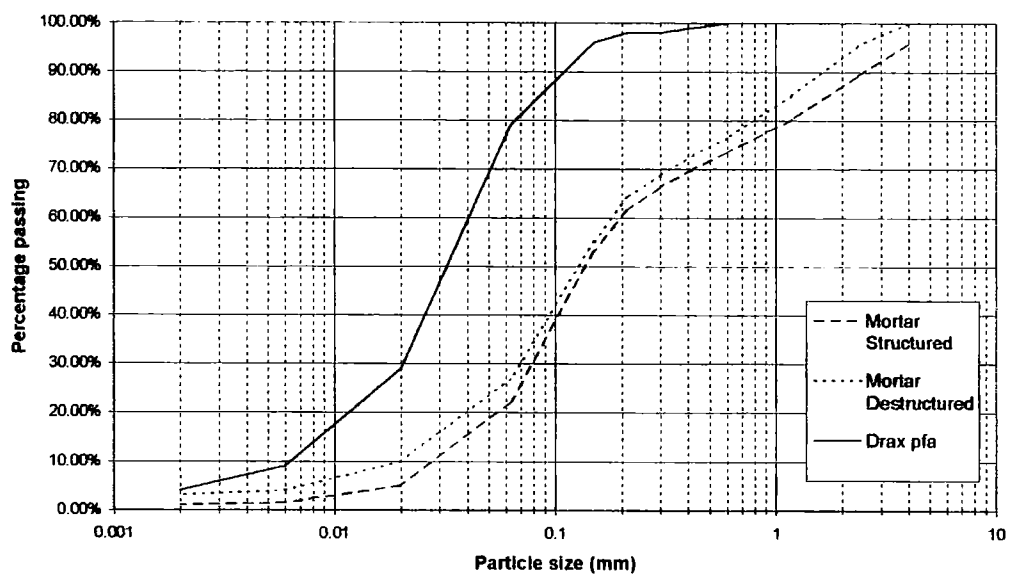
Figure 3.11 Particle Distributions for Drax fly ash on its own, and when mixed with lime
