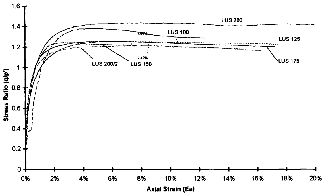
Figure 5-41 Stress ratio against strain for LUS'100-200' tests with LUS100 and LUS200 for comparison
