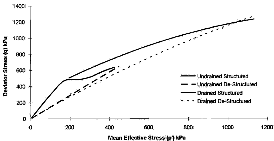
Figure 6-42 Comparison between the boundary surfaces for the two triaxial testing conditions
