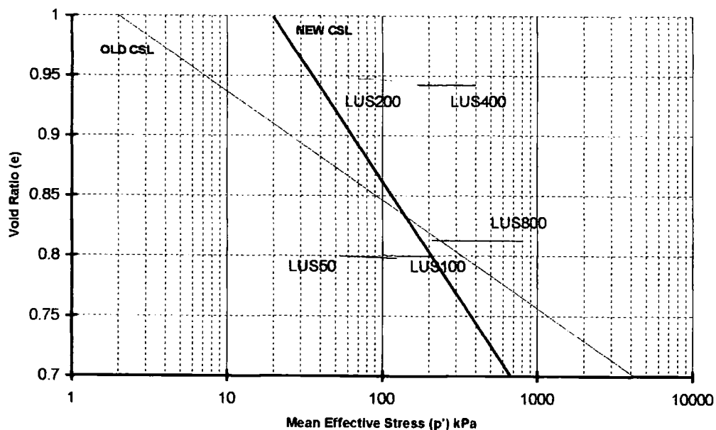
Figure 5-75a Comparison of new CSL to LUS tests '25-800'
