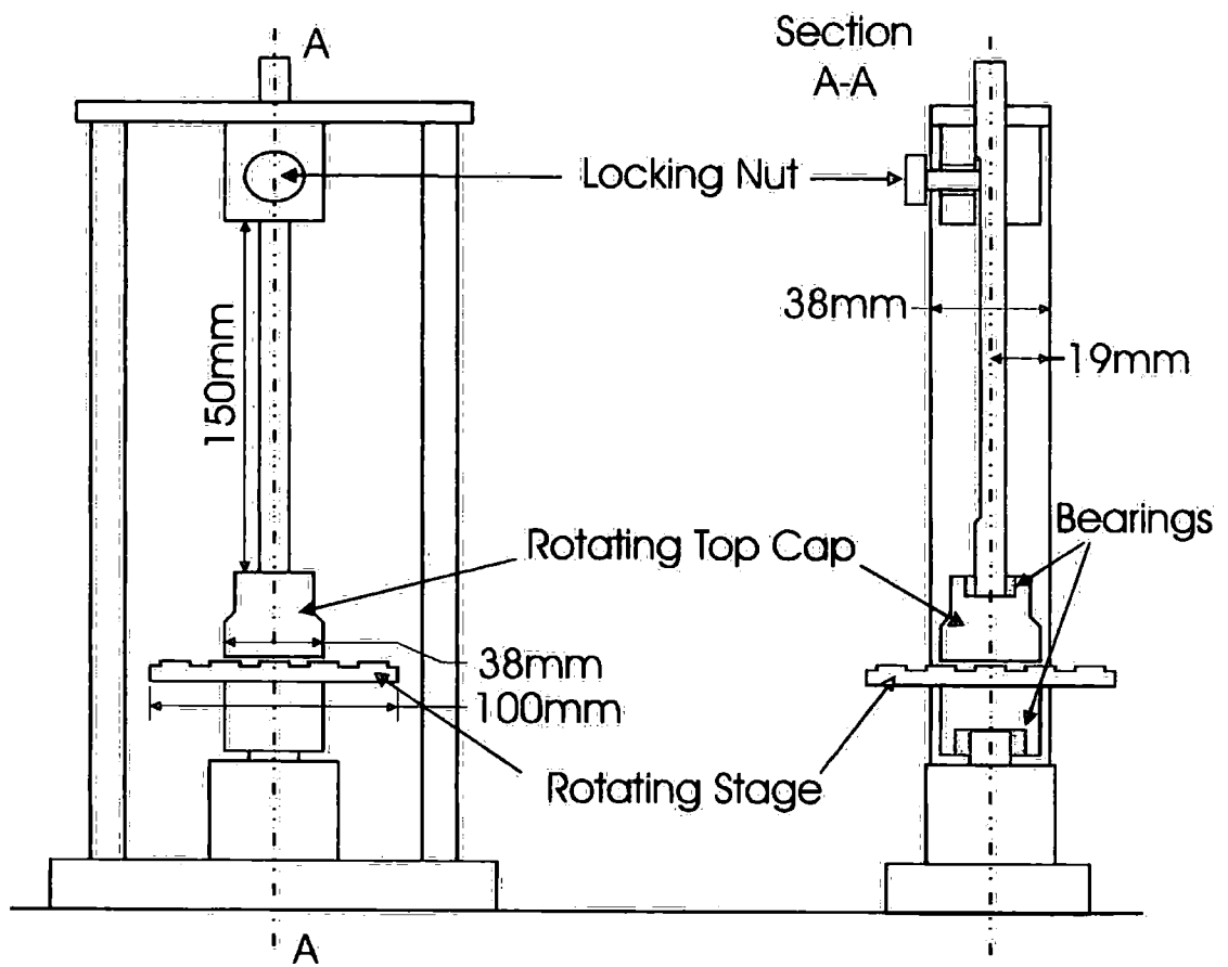
Figure 4-3 Soil Lathe for trimming undisturbed material into 38mm cylindrical specimens
