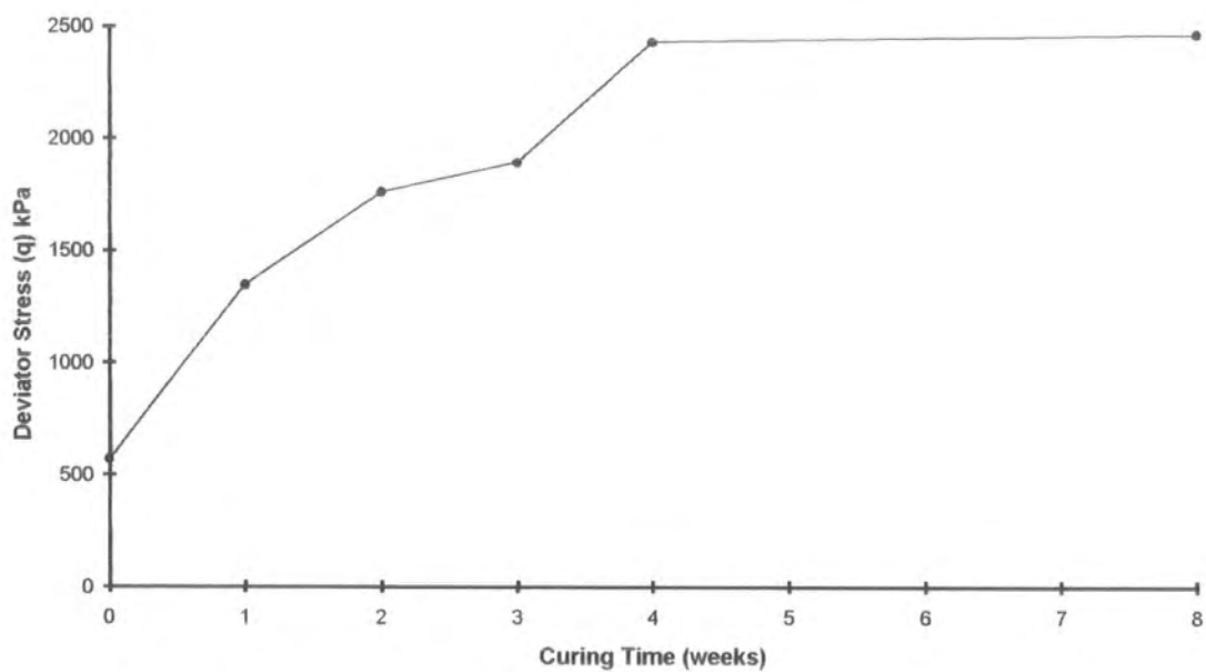
Figure 6.1 Maximum strength against curing time for lime/fly ash mortar specimen
