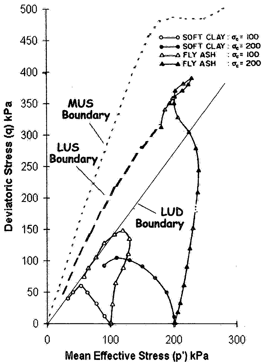
Figure 6-46 Comparison of the boundaries derived for LUD, LUS and MUS tests against test result by Inraratne et al (1991)
