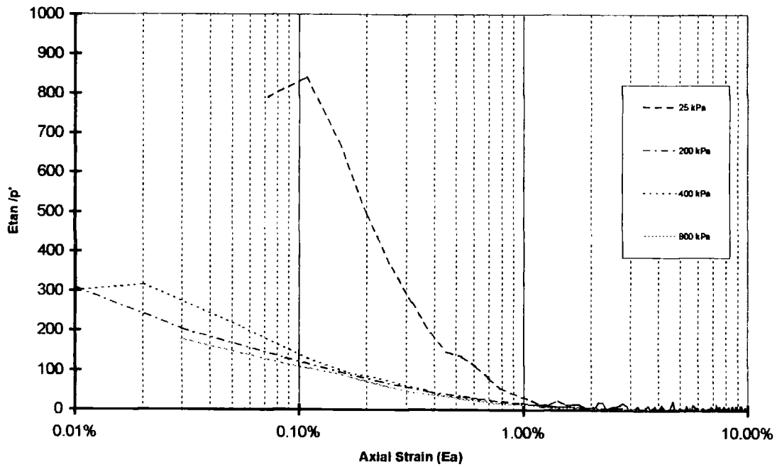
Figure 5-36 Plot of stiffness normalised with respect to the mean effective stress against strain for LUS '25-800' tests using internal strain measuring devices only
