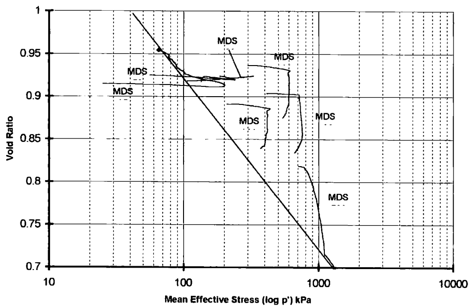
Figure 6-24 Void ratio against mean effective stress plots for MDS tests
