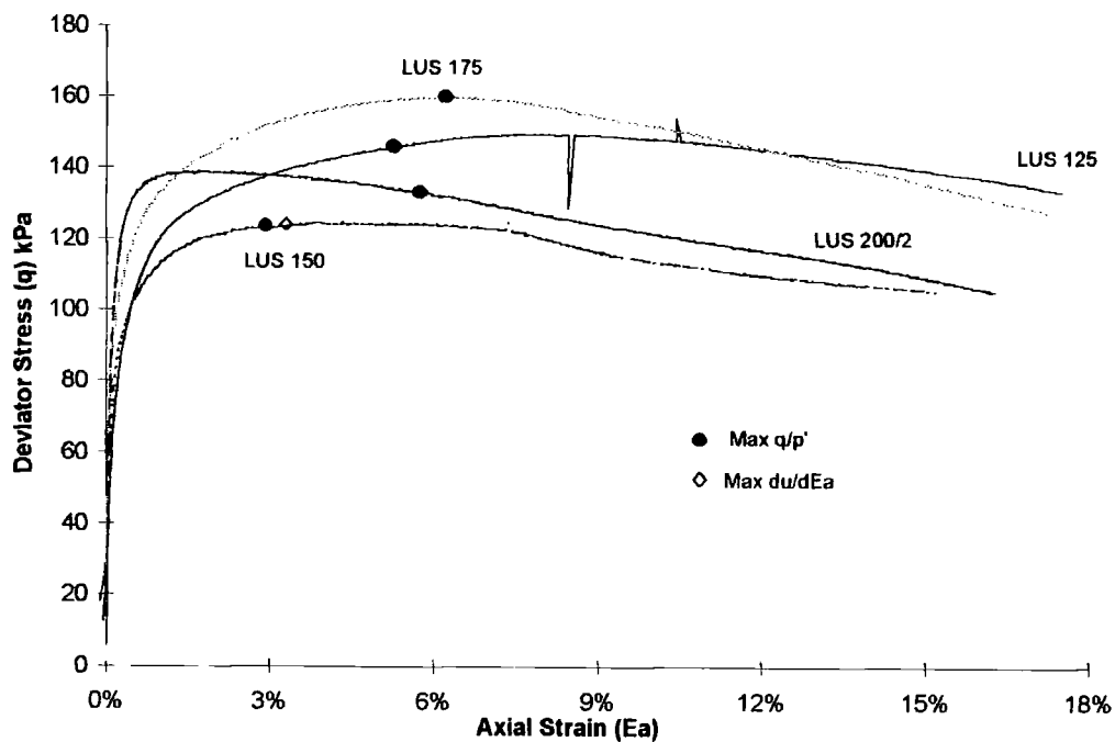
Figure 5-42 Relative position of maximum points for LUS '100-200' test plotted on stress-strain curves
