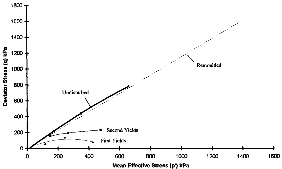
Figure 5.22 Framework for drained triaxial tests on lagoon fly ash
