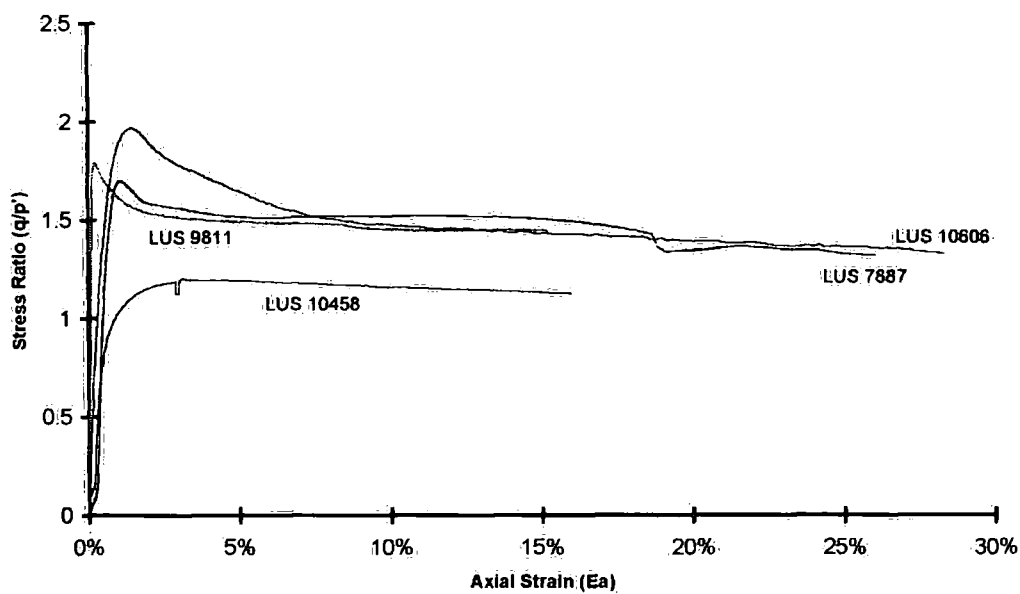
Figure 5-51 Stress ratio versus strain for BS406 tests at 75kPa confining pressure
