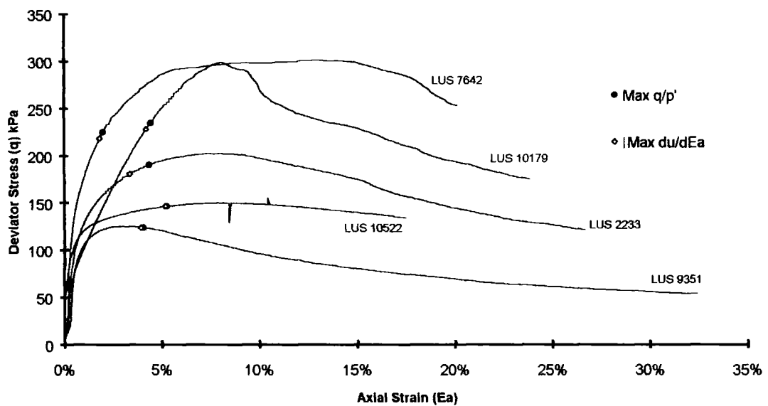
Figure 5-59 Relative position of maximum point for BS406 tests at 125kPa confining pressure plotted on stress-strain curves
