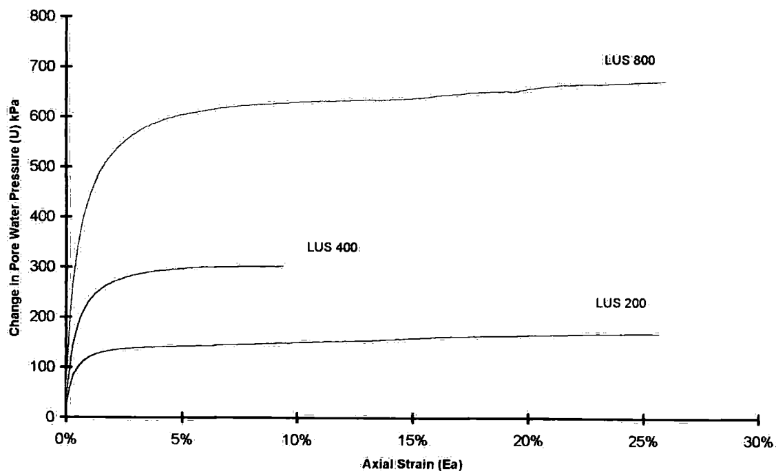
Figure 5-31b Changes in pore water pressure versus axial strain for LUS '25-800' tests at 200kPa confining pressure and above.
