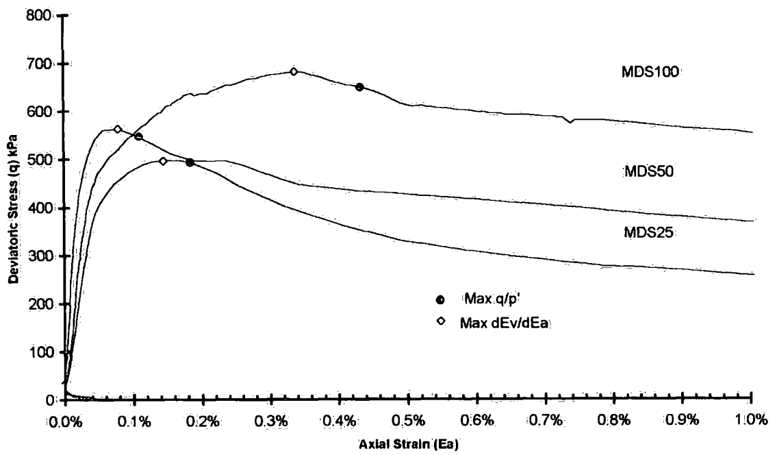
Figure 6-22 Maximum points for MDS25, MDS50 & MDS100 plotted relative to stress-strain curves
