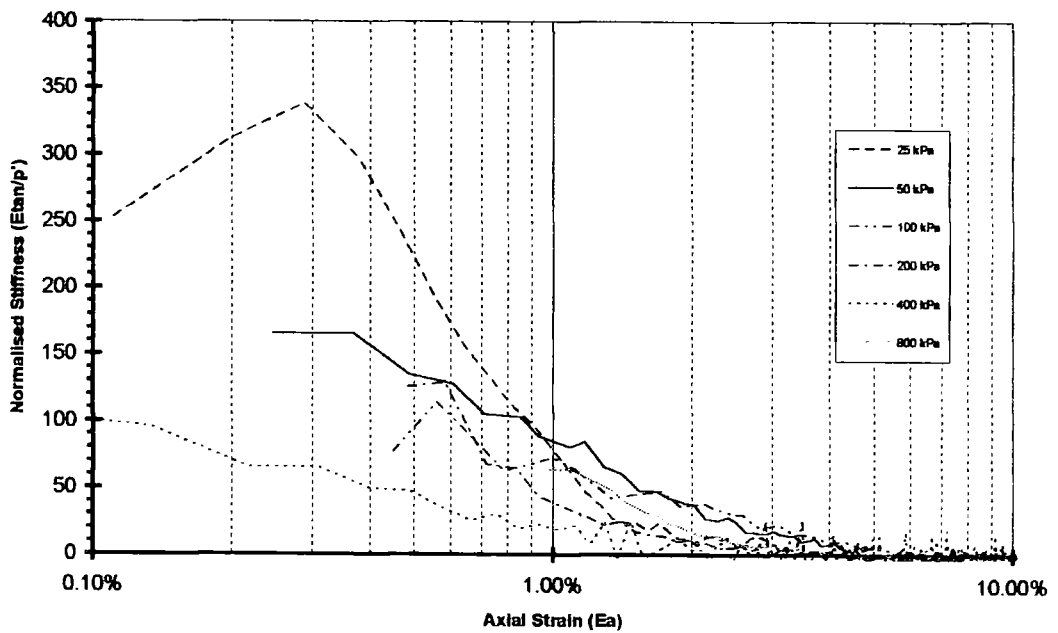
Figure 5-37 Plot of stiffness normalised with respect to the mean effective stress against strain for LUS '25-800' tests
