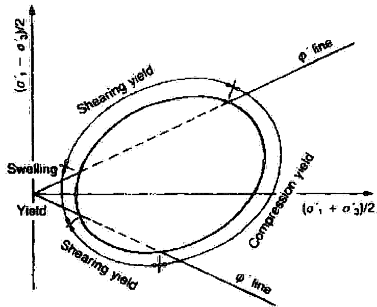
Figure 2-1 A typical yield loci within stress space showing different types of yield (Vaughan & Leroueil 1990)
