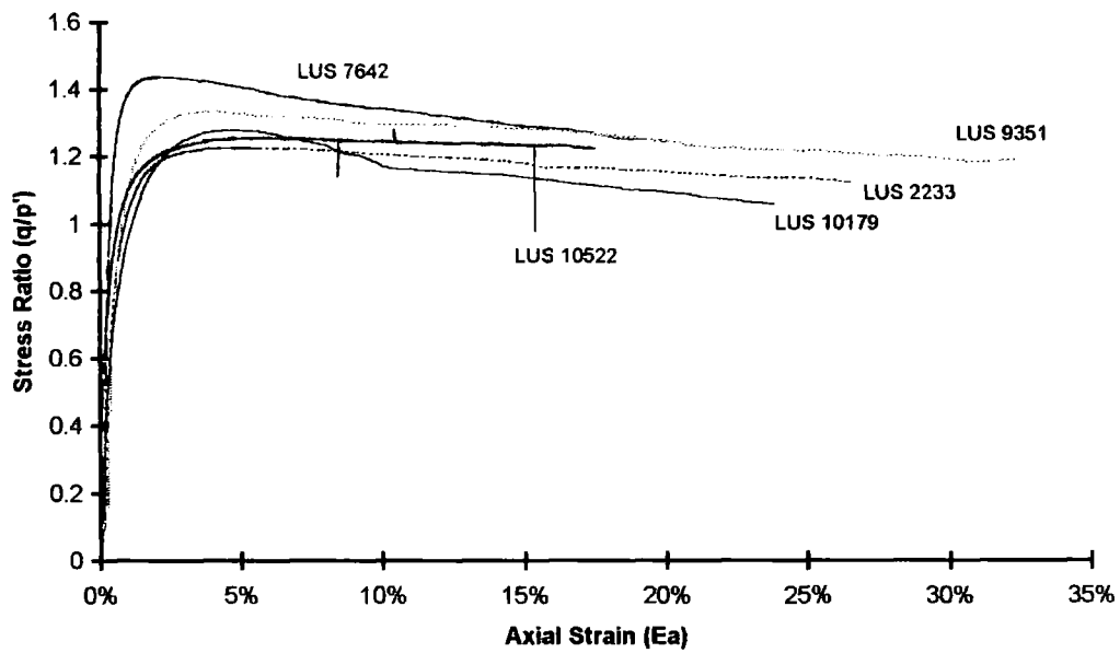
Figure 5-58 Stress ratio against strain for BS406 tests at 125kPa confining pressure
