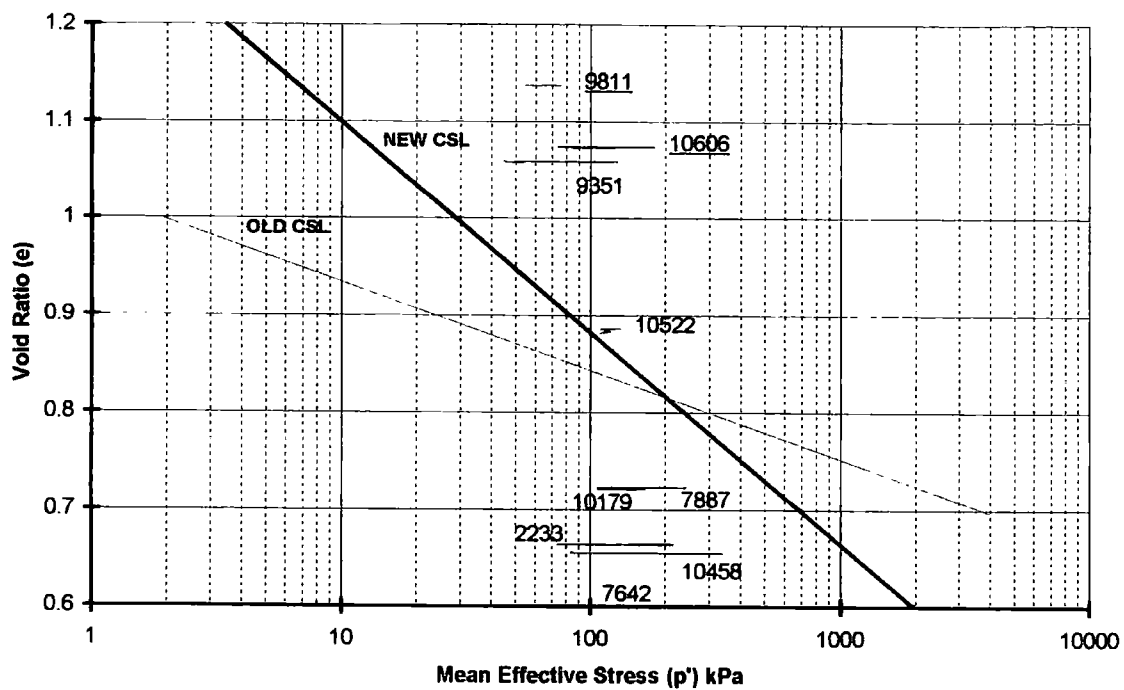
Figure 5-75c Comparison of new CSL to LUS tests 'Depth Profile
