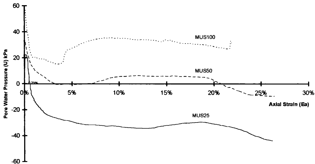
Figure 6-34 Changes in pore water pressure against strain plot for tests at 100kPa confining pressure and below
