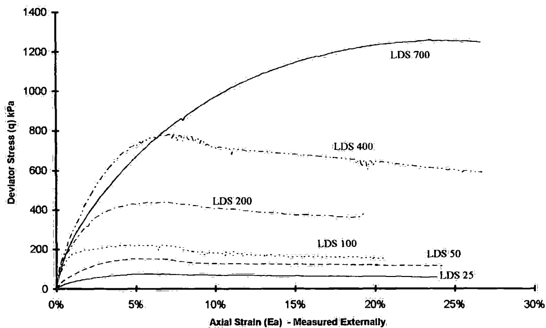
Figure 5.6b Stress against Strain plot for LDS tests using external strain measuring devices
