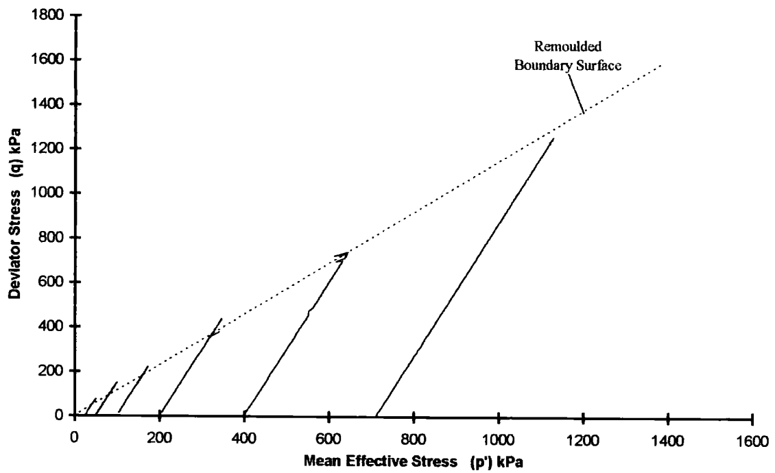
Figure 5.8 Effective stress paths for LDS tests
