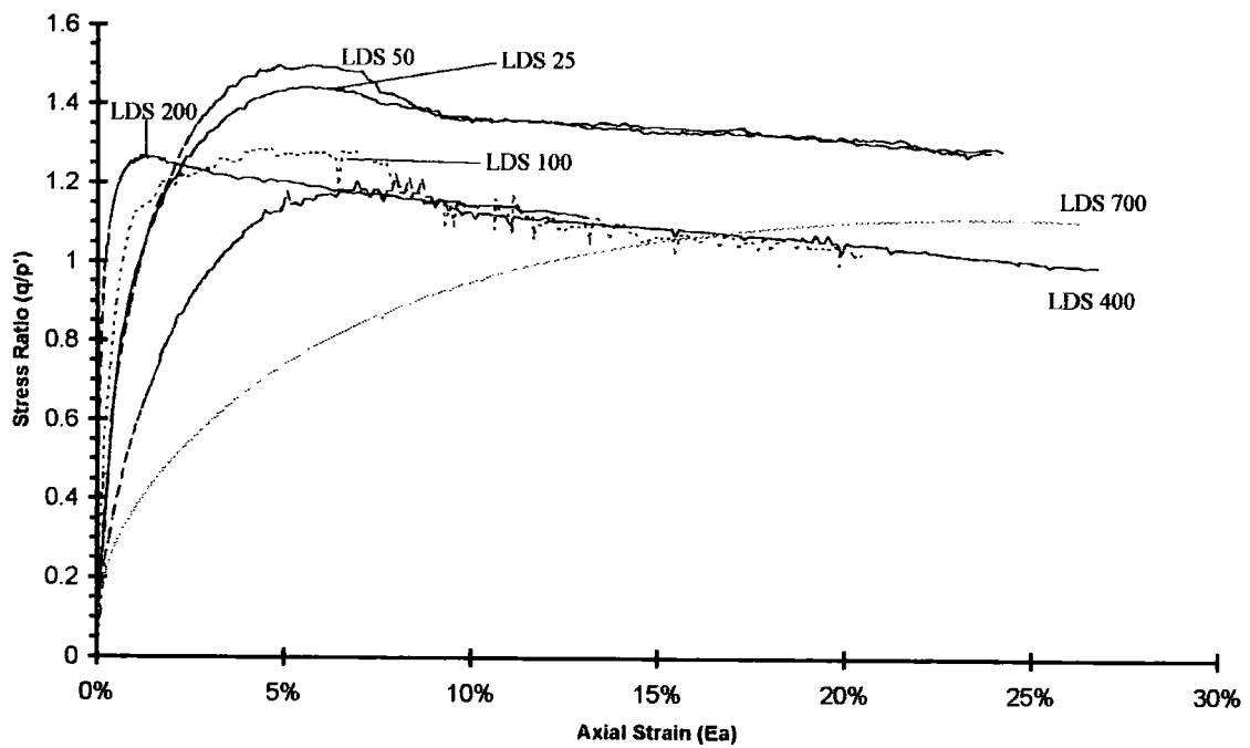
Figure 5.9 Stress ratio against strain plot for LDS tests
