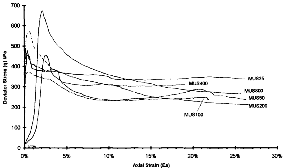
Figure 6-31 Stress against strain plots for MUS tests
