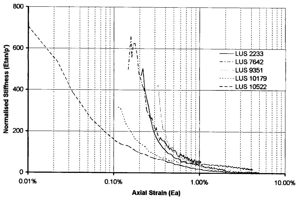
Figure 5-61 Normalised stiffness against strain for BS406 tests at 125kPa confining pressure
