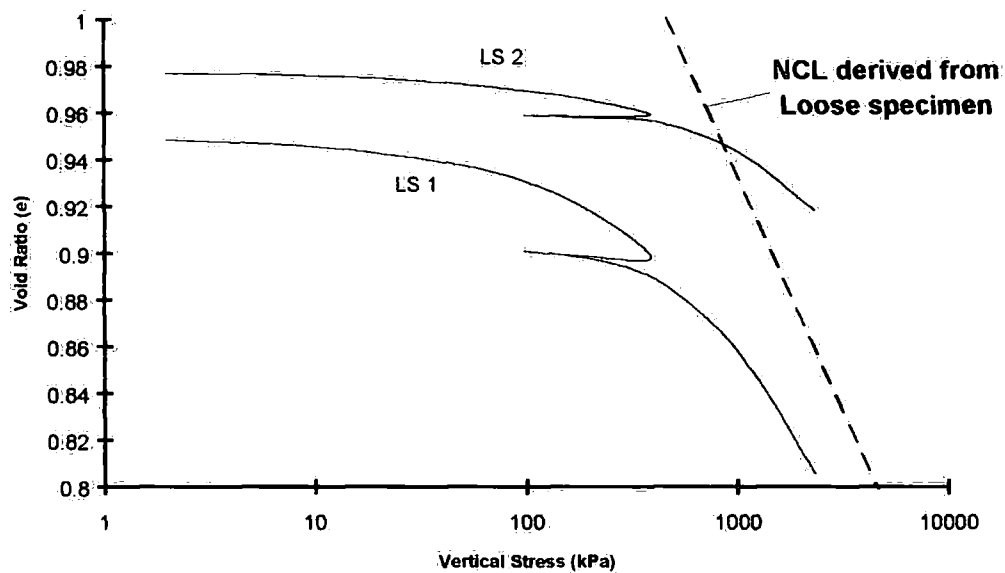
Figure 5-66 Consolidation curves for undisturbed lagoon fly ash specimens
