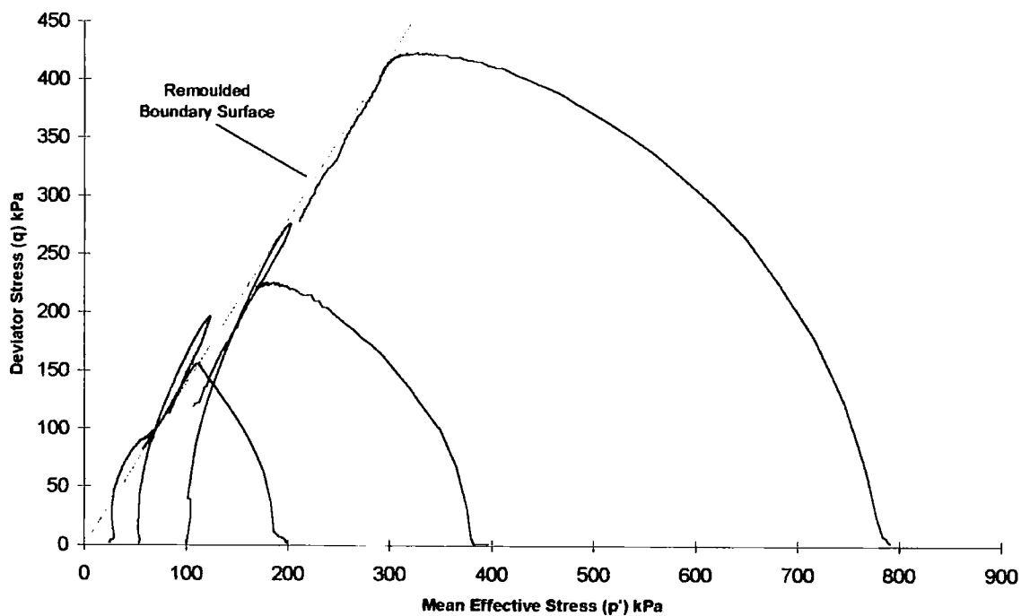
Figure 5-32 Effective stress paths for LUS '25-800' tests
