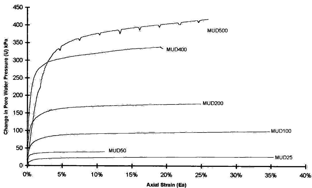
Figure 6-27 Changes in pore water pressure versus strain plots for MUD tests
