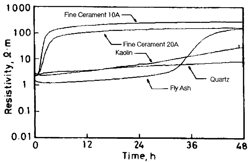
Figure 2-5 Variation of resistivity with time. The fly ash shows a retardation to its activity (Tashiro 1994)
