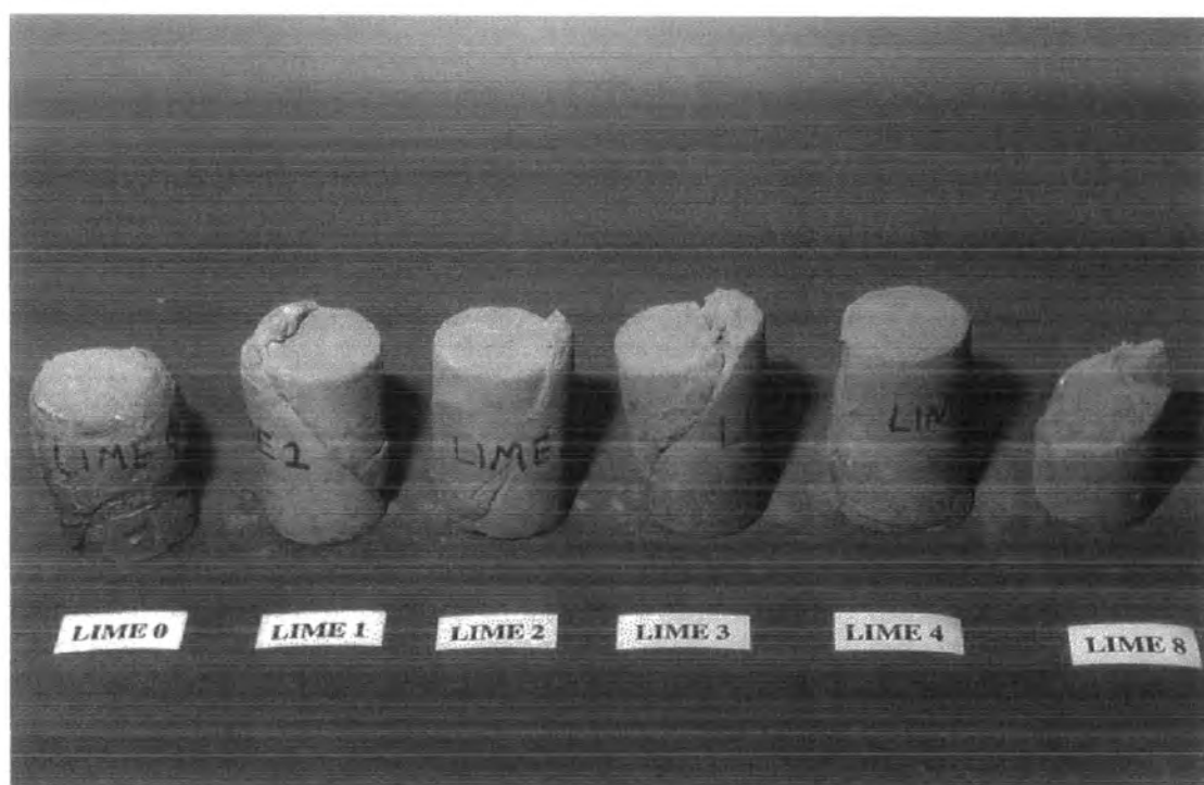
Plate 6-1 Lime/fly ash mortar specimens after undergoing triaxial compression
