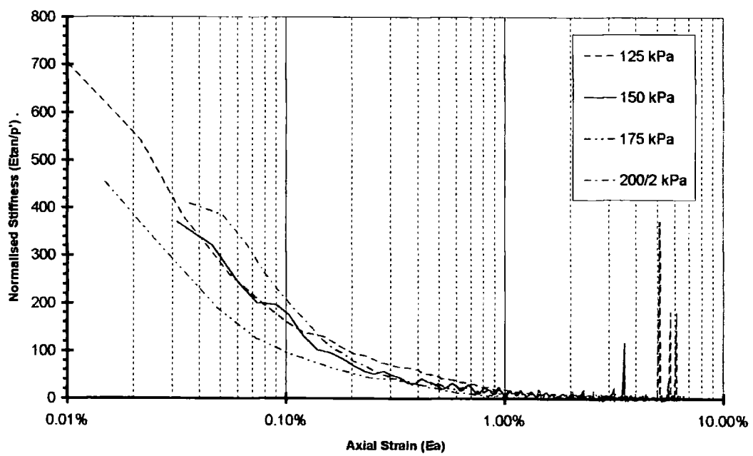
Figure 5-44 Plots of normalised stiffness against strain for LUS'100-200' tests
