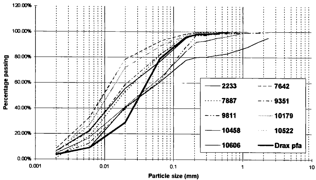
Figure 3-10 Particle distributions from BS406 and Drax fly ash. The numbers refer to tubes extracted from BS406 as shown in Table 3-2.
