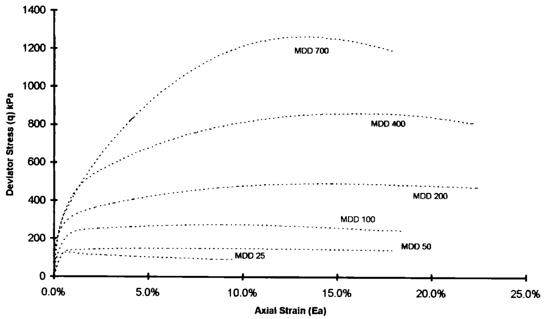
Figure 6.3 Stress against axial strain plot for MDD tests
