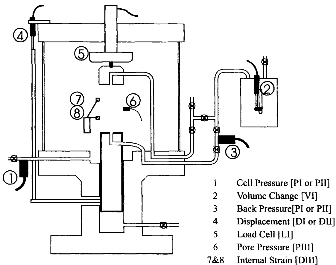
Figure 4-2 The location of transducers used in the Stress Path Cell
