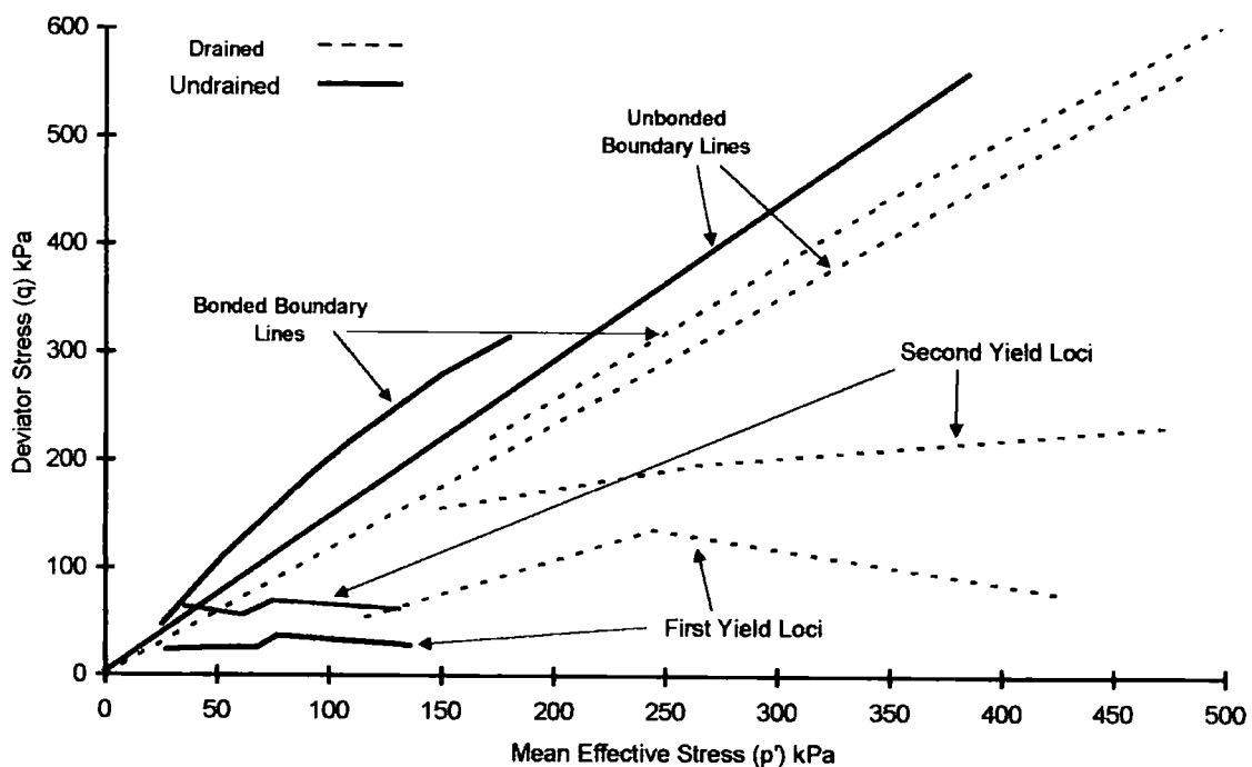
Figure 5-76 Comparison of drained and undrained test yield loci
