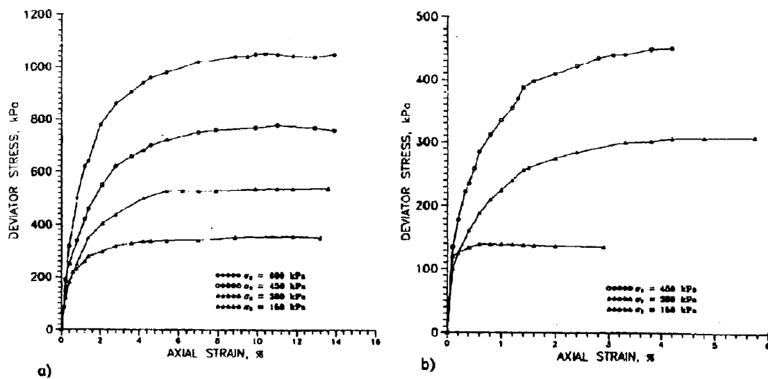
Figure 5-78 Group of triaxial tests (a) Drained & b) Undrained on fly ash after Indraratna et al (1990)
