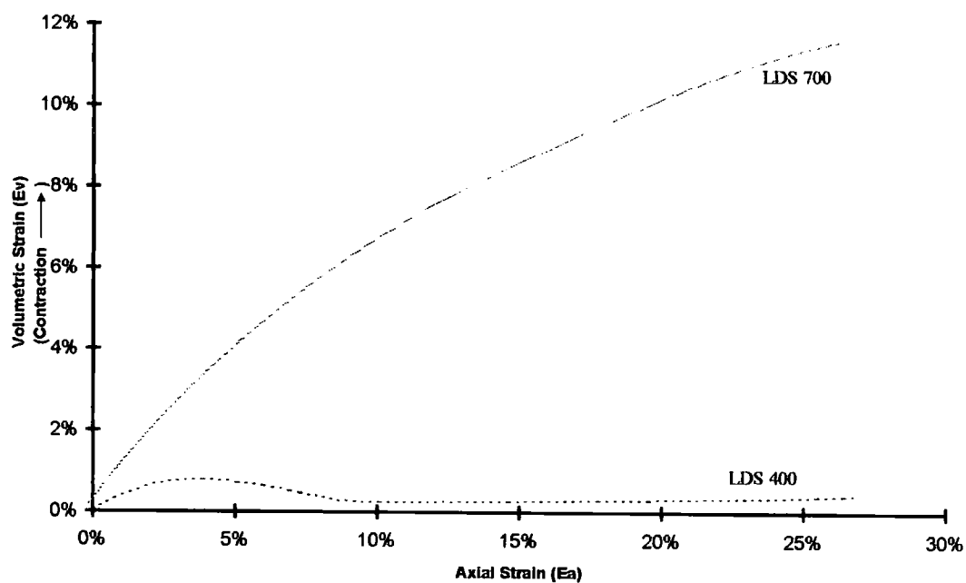
Figure 5-7b Volumetric strain versus axial strain for LDS tests at 400 & 700kPa confining pressure
