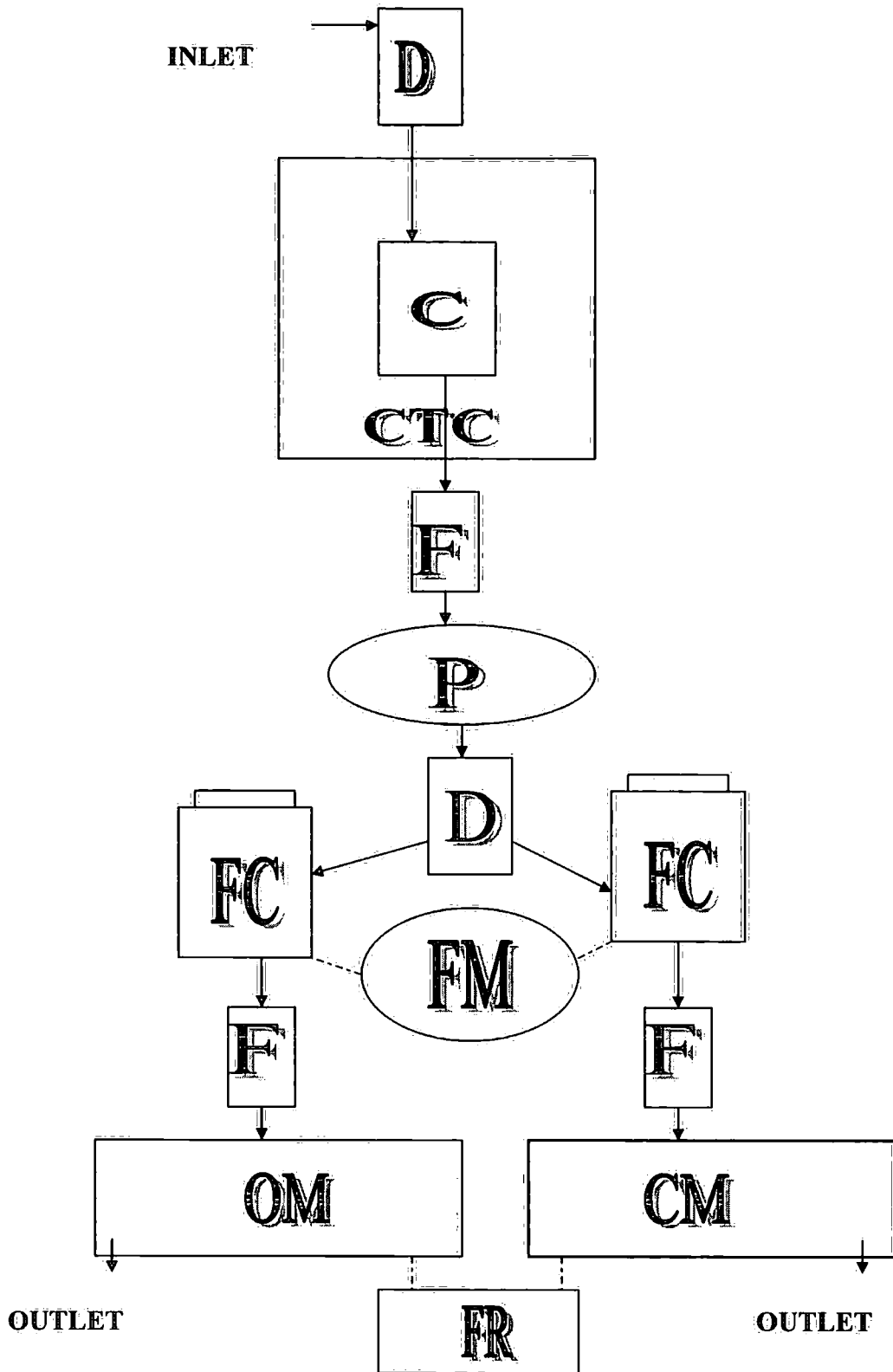
Figure 2.2: Schematic diagram of the apparatus used to measure the metabolic rate of birds during the course of this study. D= air drier, C= measurement chamber, P= pump, CTC = controlled temperature cabinet, CM = carbon dioxide meter, OM = oxygen meter, F = gas flow meter, FC= mass flow controller, FM = flow meter machine, FR = flatbed recorder, → direction of air.
