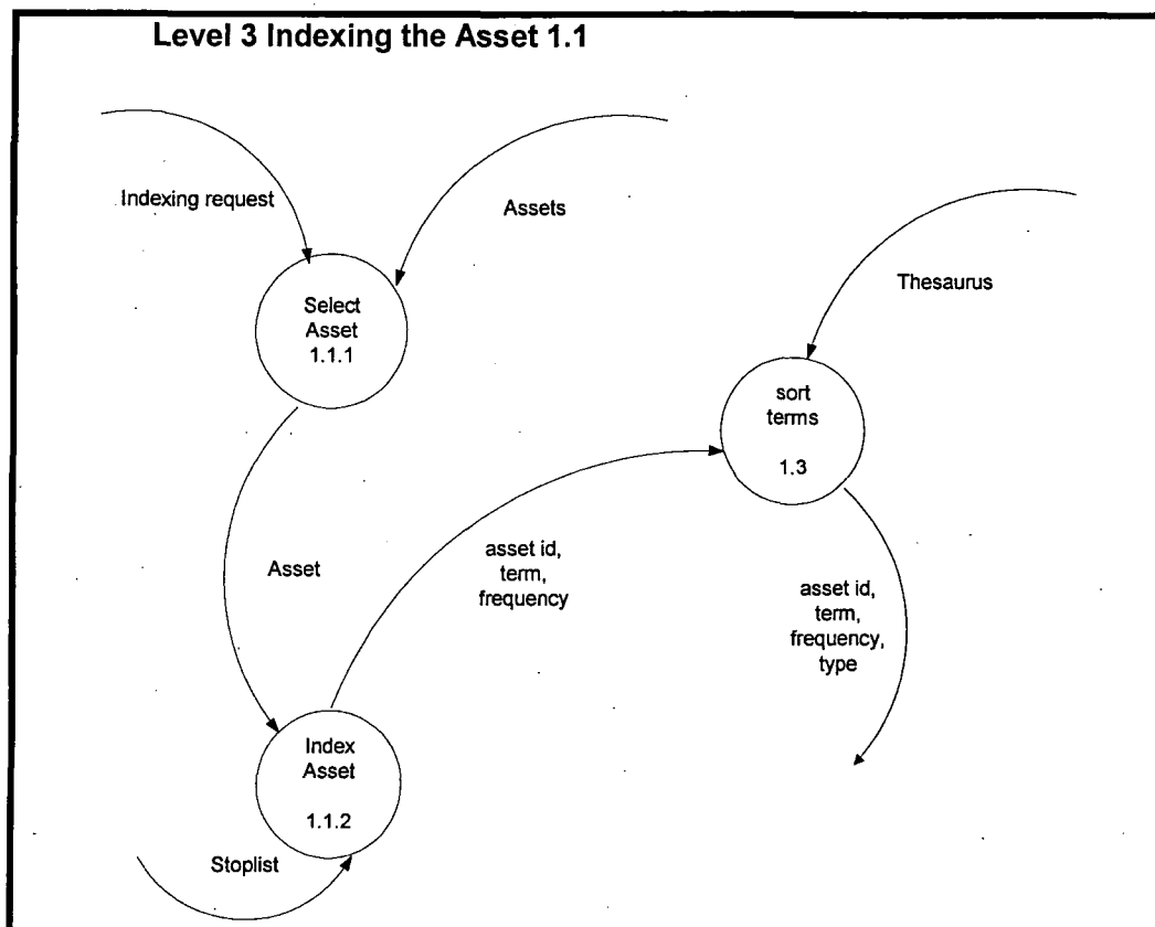
Figure 6.4 Level 3 Dataflow Diagram of Indexing the Asset
