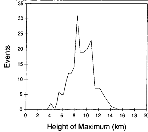
Figure 7.7: The height of maximum distribution for a spectrum of gamma rays at 0^\circ zenith angle.
