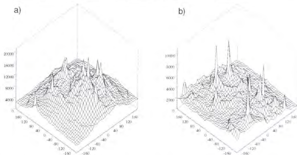
Figure 3.12: The distribution on the ground of Cherenkov photons from a) Helium and b) Magnesium nuclei with primary energies of 2 TeV. The graphs are measured over a 400 \times 400 m area with 10 \times 10 m grid resolution.
