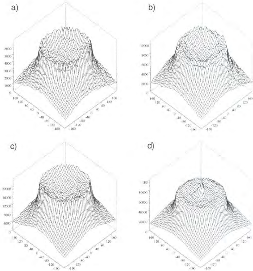
Figure 3.10: The distribution on the ground of Cherenkov photons from gamma ray EAS with primary energies of a) 300GeV, b) 500GeV, c) 1TeV and d) 3TeV. The distributions are measured over a 400 \times 400 m area with 10 \times 10 m grid resolution.
