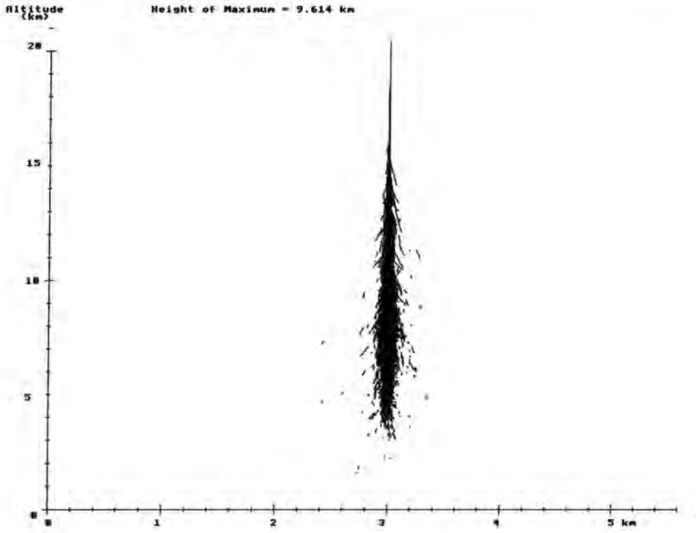
Figure 3.2: The simulated development of a 300GeV gamma ray EAS. Shown are the tracks of electrons and positrons with energies above 21MeV.
