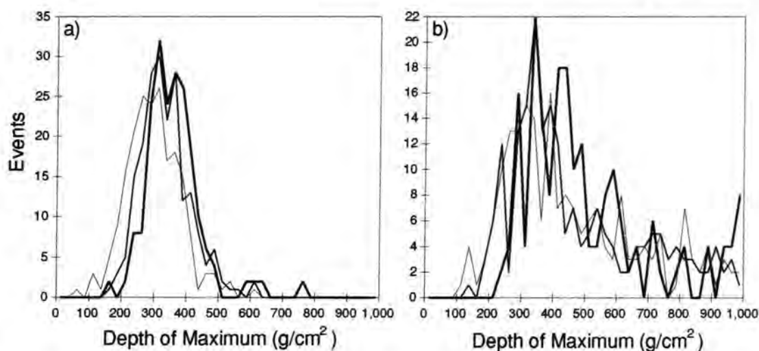
Figure 3.6: Normalised (to total events= 200) distributions of the depth of maxima for a) gamma ray and b) hadron showers. The thicker lines indicate higher primary energies (see table 3.1 for more details).
