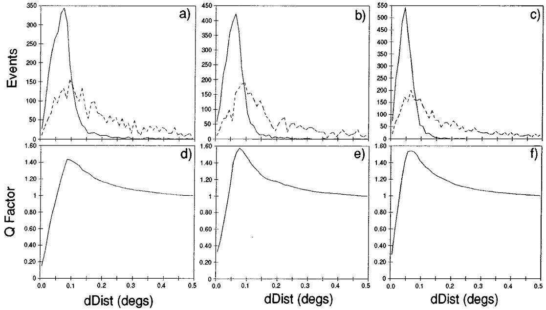
Figure 7.8: The distributions of dDist for simulated gamma rays (solid line) and hadrons (dashed line) imaged by an ideal optical system at zenith angles of a) 0° , b) 30° , and c) 60° . Shown in d), e) and f) are the Q factors obtained from the data in a), b) and c) when events with dDist greater than a particular value are rejected.
