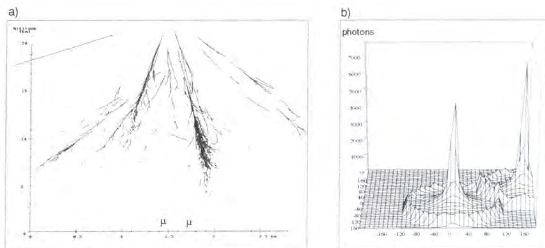
Figure 3.13: a) A low energy (300 GeV) proton EAS with two penetrating high energy muons. b) The Cherenkov emission, plotted on the ground in 10 \times 10 m bins, is dominated by the muons.
