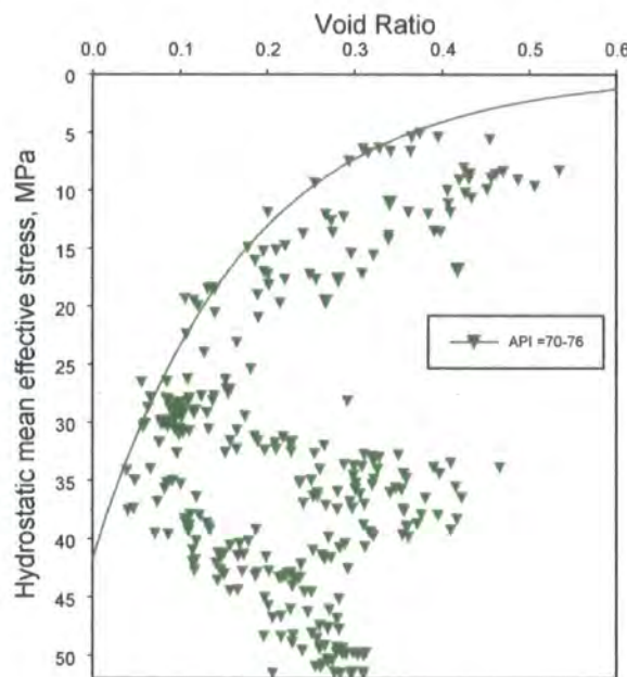
Figure 5.6 Void ratio vs mean hydrostatic effective stress for all shales from Wells E, F and G. Shales are subdivided into lithology on the basis of gamma ray response.
