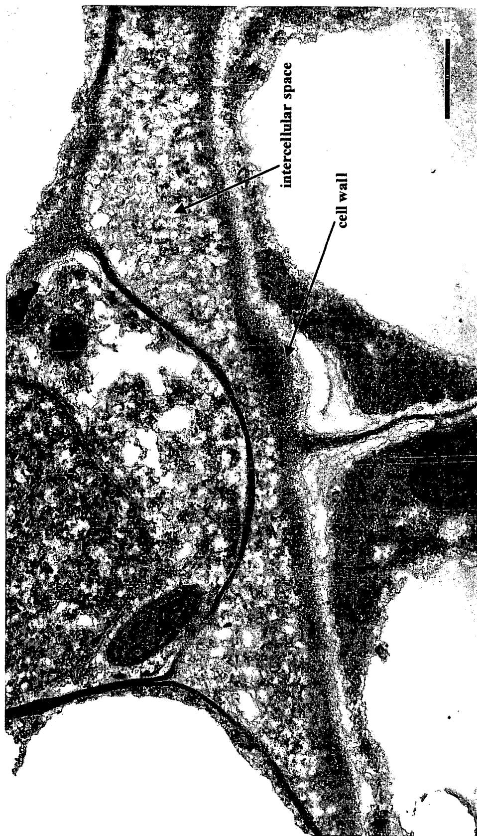
Figure 4.8 Electron micrograph of part of a transverse section of an inflorescence from Arabidopsis (23,500X magnification) incubated with preimmune serum (1/100). The section was subsequently incubated with anti-rabbit IgG conjugated to gold particles (20nm in diameter). Gold particles were found only very rarely in intercellular spaces, the cell wall, cytoplasm and in cellular organelles, such as chloroplasts and mitochondria. Scale bar = 850nm.
