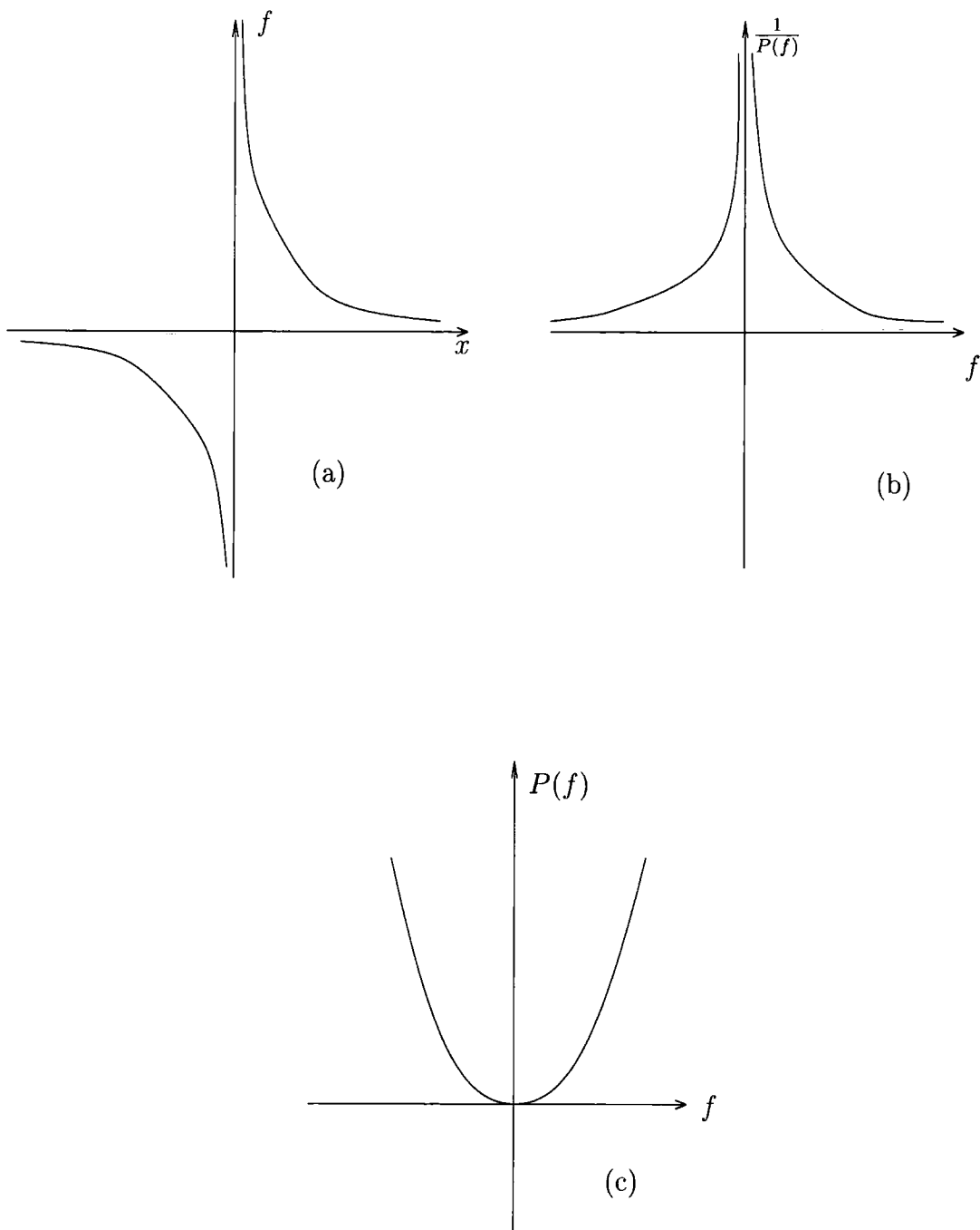
Figure 2.8: For X = \mathbb{R} from f in (a) the required shape of P(f) for winding solutions can be deduced through (b).
