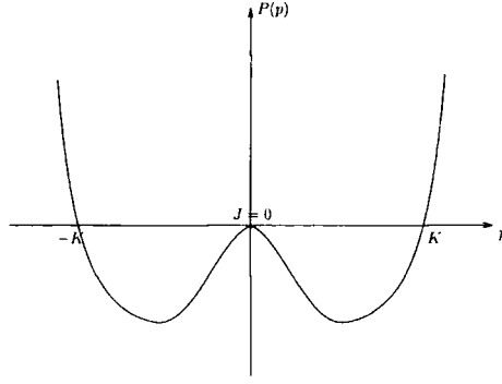
Figure 3.3: P(p) with double zero J = 0 .
