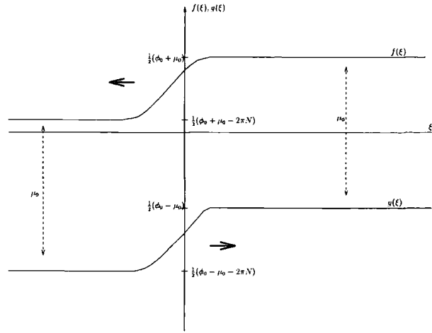
Figure 3.5: The two kinks f(\xi), g(\xi) at t = 0 .
