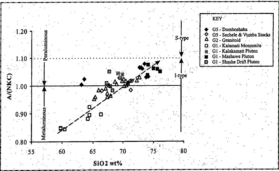
Figure 3.6: Alumina saturation (Shand, 1951) and I-&S type (Chappell and White, 1974) diagram of the granitoids from the Vumba granite-greenstone terrain. Abbreviations: A/(NKC) = Mol% Al_2O_3/(Na_2O + K_2O + CaO) .
