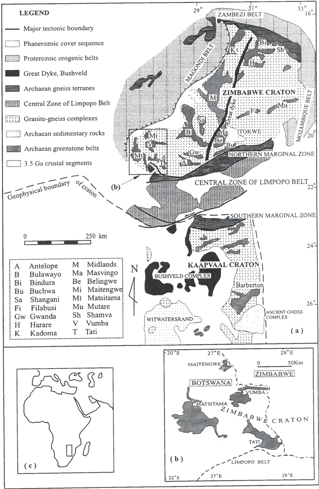
Figure. 1.1: (a) Map showing the main geological units of Southern African cratons and adjacent Proterozoic belts (Modified from Treloar and Blenkinsop, 1995, and Jelsma and Dirks, 2000). The rectangle locates the map of Fig. 1.1b. (b) Distribution of the four granite-greenstone terrains of the Zimbabwe craton in NE Botswana. (c) Location of the Southern Africa cratons.
