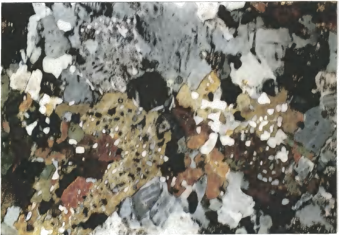
Photo 3.4. Skeletal clinoamphibole crystals poikilitically enclosing fine quartz grains. This is a characteristic feature of Kalakamati Monzonite (G1). Magnification: 1.3 x 0.77 mm. Sample ZB-98-85.
