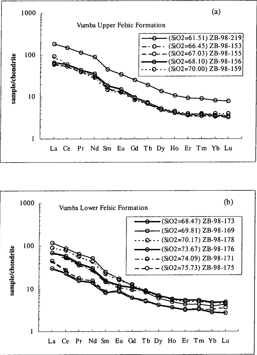
Figure 6.3: Chondrite-normalised REE plots for the felsic metavolcanics from the Vumba granite-greenstone terrain. Chondrite normalising values are taken from Boynton (1984).
