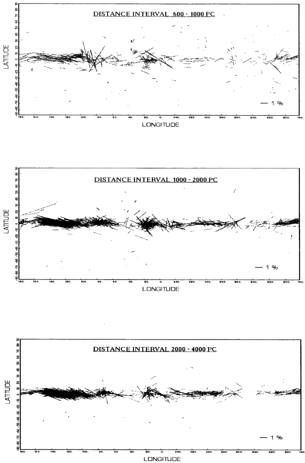
Figure 2.8: Interstellar polarization as a function of distance. Axon & Ellis (1976)
