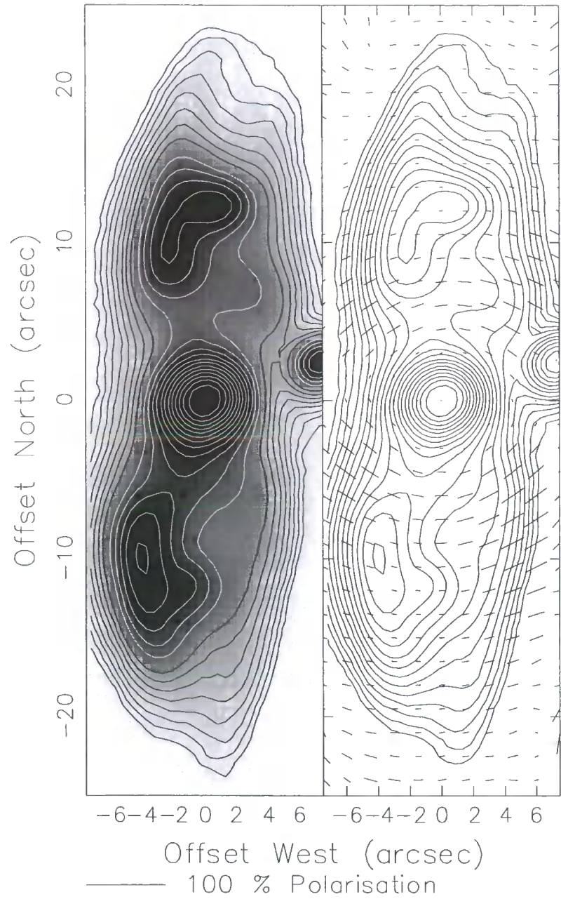
Figure 3.11: R-band total intensity image with superposed contour data, and polarization image with superposed contour data. Polarization data are corrected for ISP.
