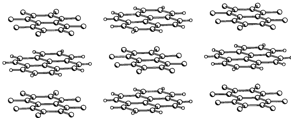
Figure 6.7(h) Packing diagram of OFN·pyrene (8)
