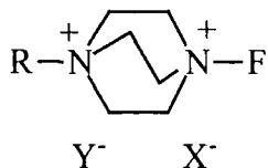
Generic structure of Selectfluor™
