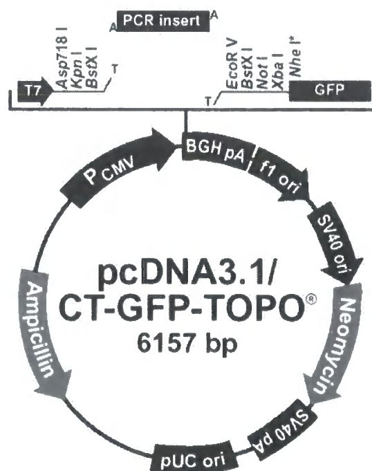
Figure 13 - The CT-TOPO-GFP- \alpha 9 vector
