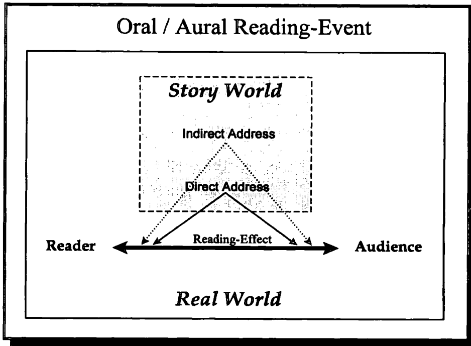
Figure 3: Oral/Aural Reading-Event
