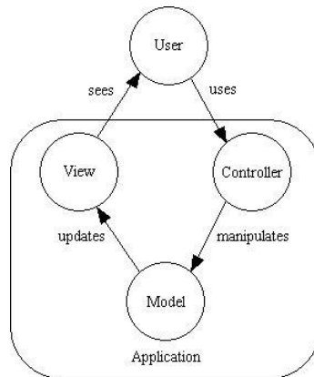
Figure 3.3: MVC explanatory diagram.
