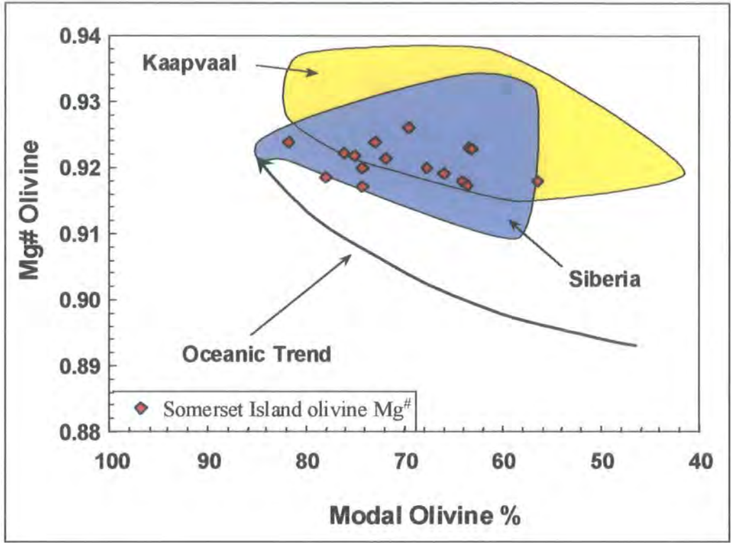
Figure 5.14 Olivine Mg^\# vs. modal olivine content (%) for Somerset Island peridotites. Fields for Low-T peridotites from the Kaapvaal and Siberian cratons (Boyd, 1989; Boyd et al. , 1997). Trend defined by oceanic peridotites after Boyd (1989).
