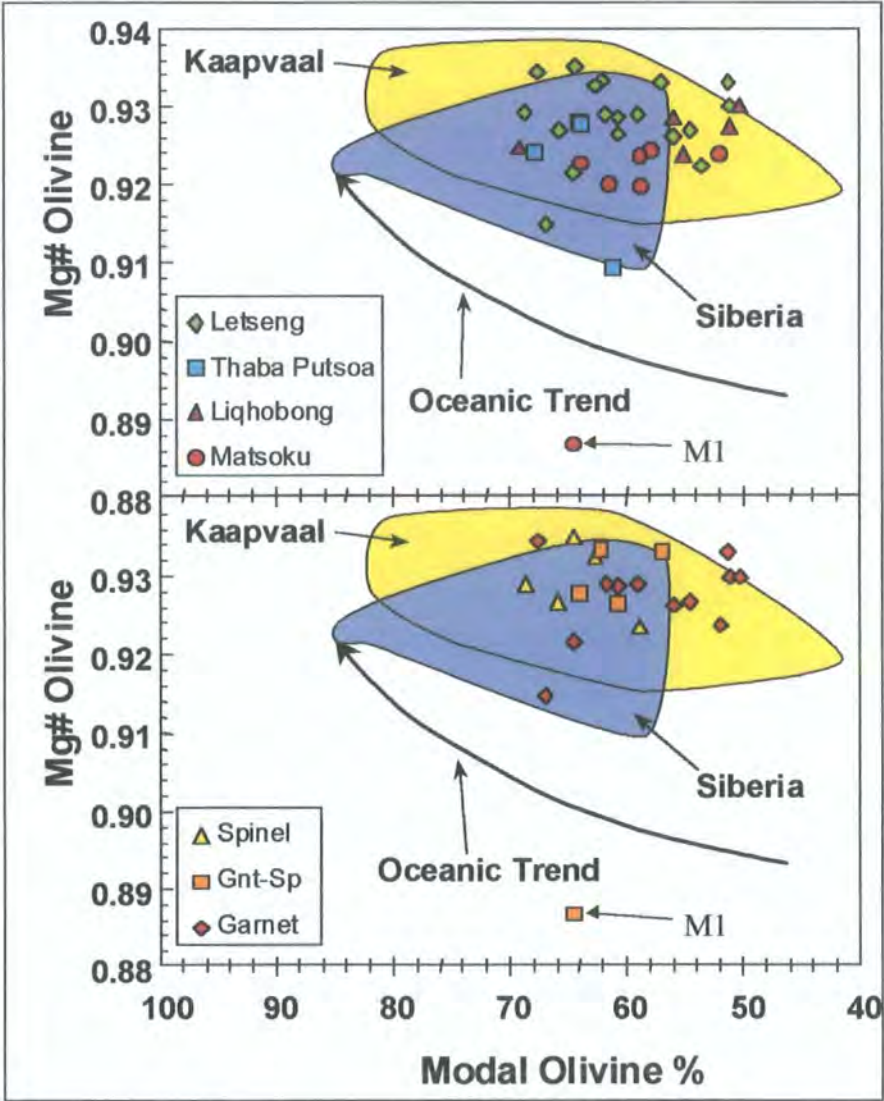
Figure 3.17 Olivine Mg^\# vs. modal olivine content (%) for low-T Lesotho peridotites. Fields for Low-T peridotites from the Kaapvaal and Siberian cratons (Boyd, 1989; Boyd et al. , 1997). Trend defined by oceanic peridotites after Boyd (1989).
