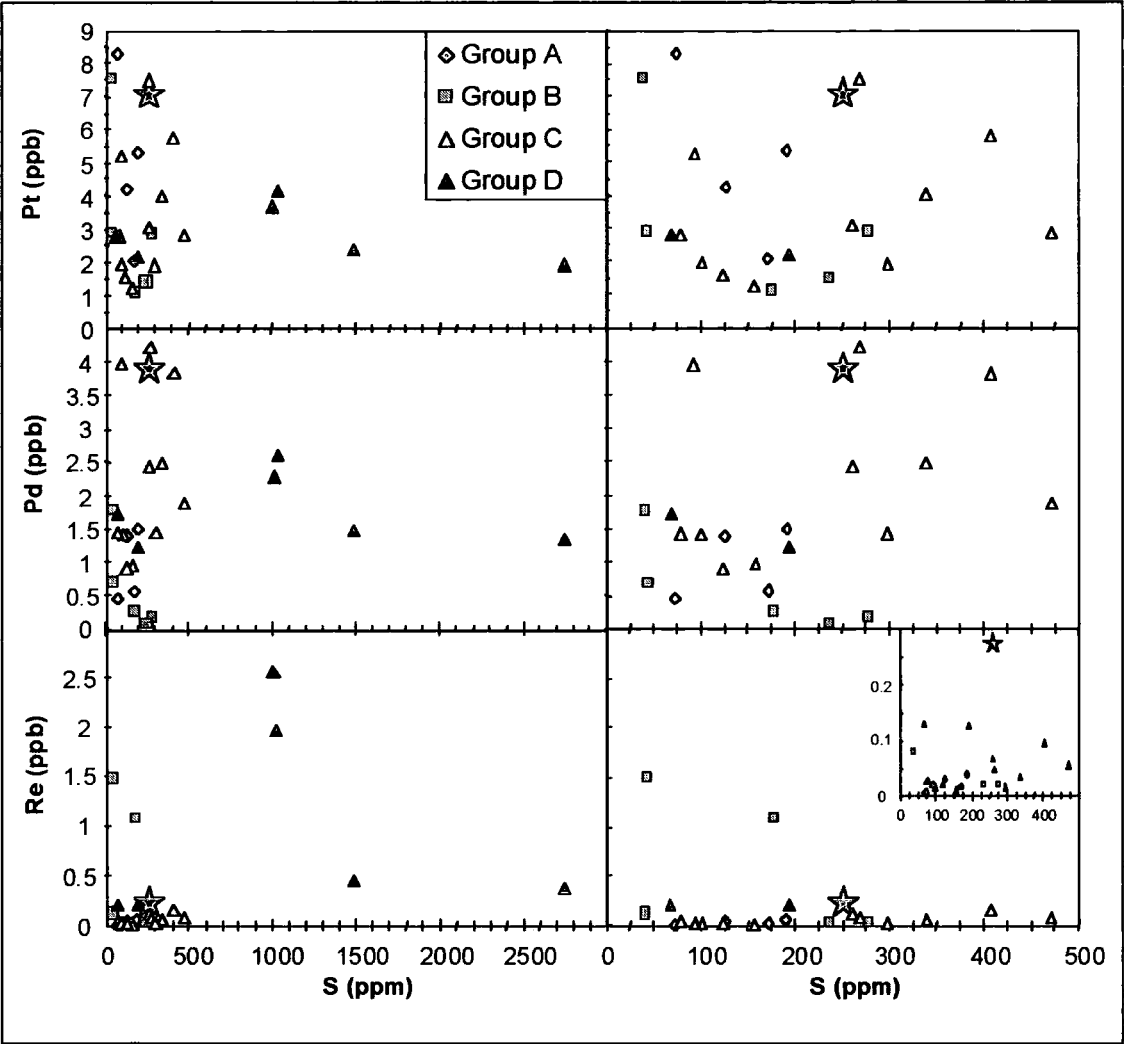
Figure 5.24 (continued) PGE and Re abundances versus S content for the Somerset Island peridotite suite. Primitive mantle, represented by star, after McDonough and Sun (1995).
