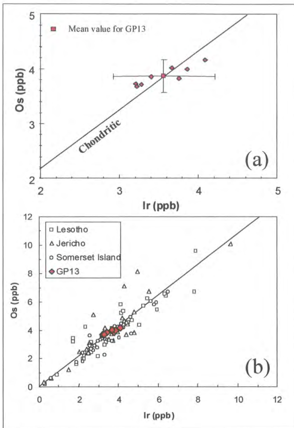
Figure 2.3 Plot of Os vs. Ir for GP13 and peridotites from the Lesotho, Jericho and Somerset Island peridotite suites. (a) Os and Ir data for GP13, from Table 2.2, with 2σ RSD% error bars. (b) Os and Ir data for GP13 and 98 peridotite samples from the Lesotho, Jericho and Somerset Island suites. Line represents the chondritic ratio (McDonough and Sun, 1995).
