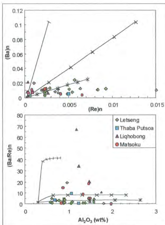
Figure 3.36 A) Chondrite normalised plot of Ba vs. Re content for Lesotho peridotites. B) Chondrite normalised Ba/Re ratio vs. \text{Al}_2\text{O}_3 . The lines represent model mixing lines between an end-member depleted peridotite ( \text{Re} = 0.01\text{ppb} , \text{Ba} = 1\text{ppm} ) and possible metasomatising magmas, marks indicate 5% increments in the addition of magma. Carbonatite (hatching; \text{Re} = 2\text{ppb} , \text{Ba} = 5000\text{ppm} ; Tuttle and Gittins (1966), kimberlite (x; \text{Re} = 2\text{ppb} , \text{Ba} = 1000\text{ppm} ; Bergman (1987) and Smith et al (1985), average OIB (star; \text{Re} = 0.35\text{ppb} , \text{Ba} = 200\text{ppm} ; Basaltic Volcanism Studies Project (1981).
