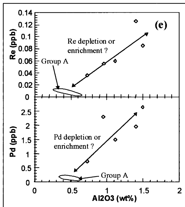
Figure 4.21 (continued) Pd and Re abundances versus \text{Al}_2\text{O}_3 content for the Jericho peridotites. (e) moderately depleted peridotites?
