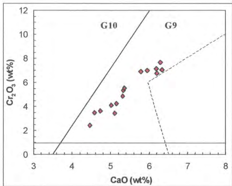
Figure 5.8 A \text{Cr}_2\text{O}_3 vs. \text{CaO} plot for garnet in Somerset Island peridotites. Fields shown for garnets (G9, G10 and all non-peridotitic garnets) are from Dawson and Stephens (Dawson and Stephens, 1975).
