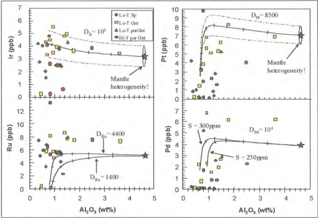
Figure 4.20 PGE abundances versus \text{Al}_2\text{O}_3 (symbols as for Figure 4.16). Predicted residue compositions are based on non-modal fractional melting models using a primitive mantle source with sulfur compositions of 300 ppm (represented by star symbol), and the extracted melts have a sulfur capacity of 1000 ppm S. The range of partition coefficients for PGEs, D_{\text{PGE}(\text{sulf/melt})} is large (Stone et al. , 1990; Bezmen et al. , 1994; Peach et al. , 1994; Fleet et al. , 1996). A value of 10^4 for D_{\text{Pd}} has been used to model Pd based upon the good correlation found by Lorand et al. (1999) in Pyrenean orogenic lherzolites. The value D_{\text{Ir}} was assumed to be an order of magnitude higher based upon contrasting behaviour of these two elements in the same study. D_{\text{Ru}} was modelled using values of 1400 and 4400, D_{\text{Pt}} a value of 8500. For comparison of models with xenolith data, F values were re-calculated as \text{Al}_2\text{O}_3 wt%. Varying S content of the source or S capacity of the melt does not significantly alter the melt extraction trends. Marks indicate 5% increments of melting.
