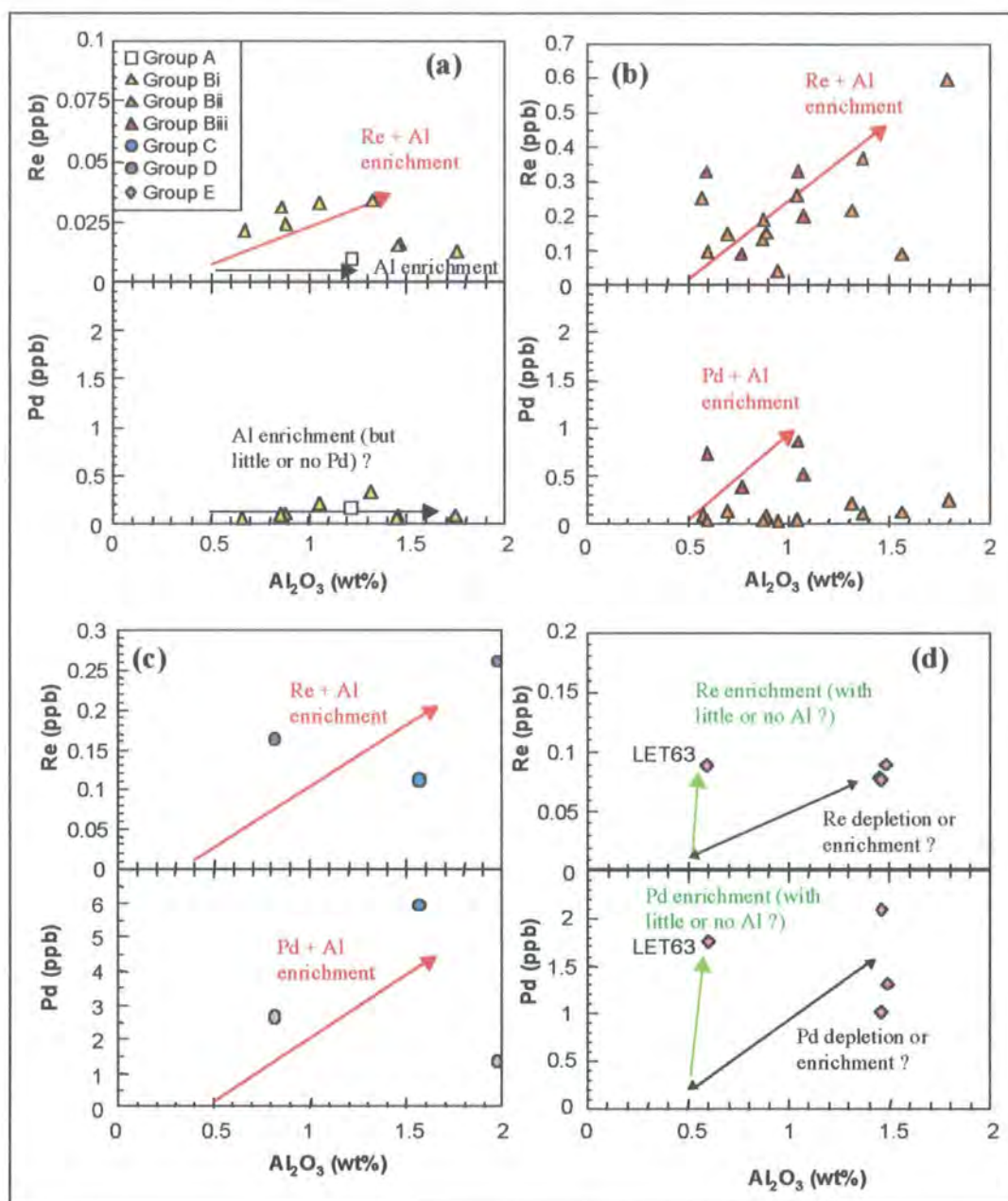
Figure 3.30 Pd and Re abundances versus \text{Al}_2\text{O}_3 content for the Lesotho peridotite, based on CI-chondrite normalised PGE patterns. (a) Group A and B peridotites, (b) Group B peridotites, (c) Group C and D peridotites, and (d) Group E peridotites.
