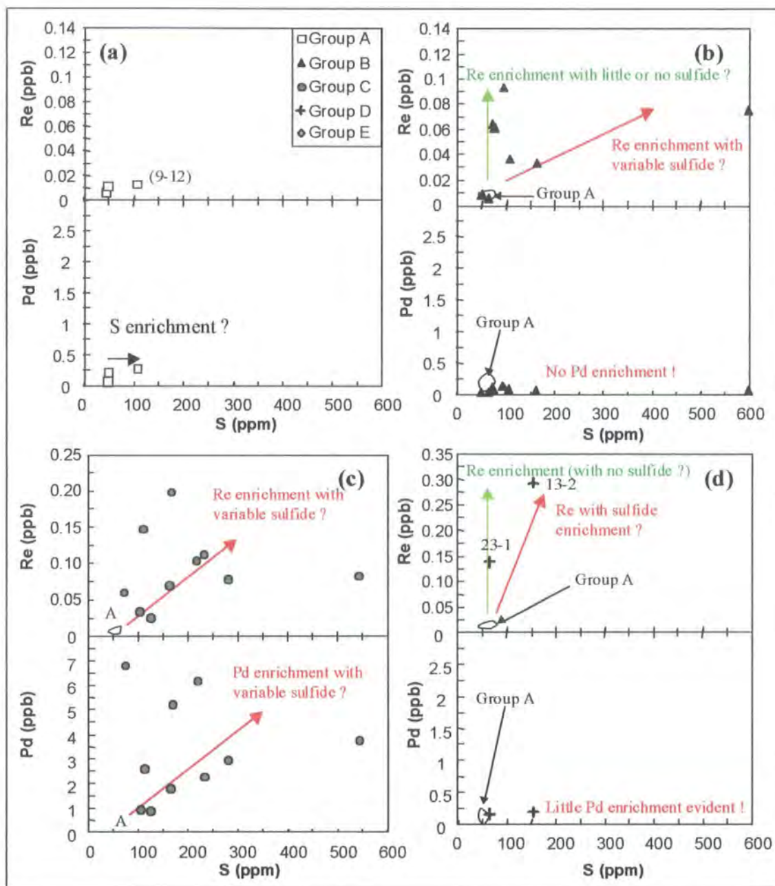
Figure 4.19 Pd and Re abundances versus S content for individual Jericho peridotite groups. (a) peridotites with highly depleted PGE patterns, (b) peridotites with Re enriched PGE patterns, (c) peridotites with Pd enriched PGE patterns, and (d) peridotites with Re and Pd enriched PGE patterns.
