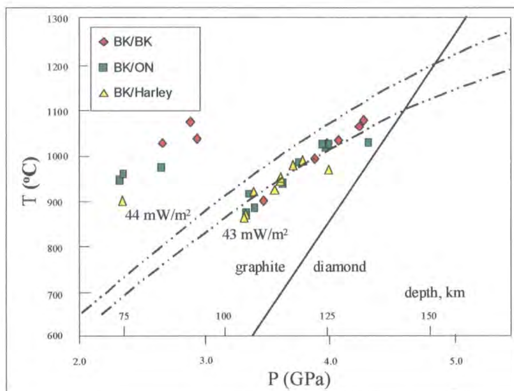
Figure 3.12 Equilibrium pressure-temperature estimates for Lesotho peridotites calculated iteratively according to (i) Brey & Köhler (1990), (ii) O'Neill (1980) and Brey & Köhler (1990), and (iii) Brey & Köhler (1990) and Harley (1984).
