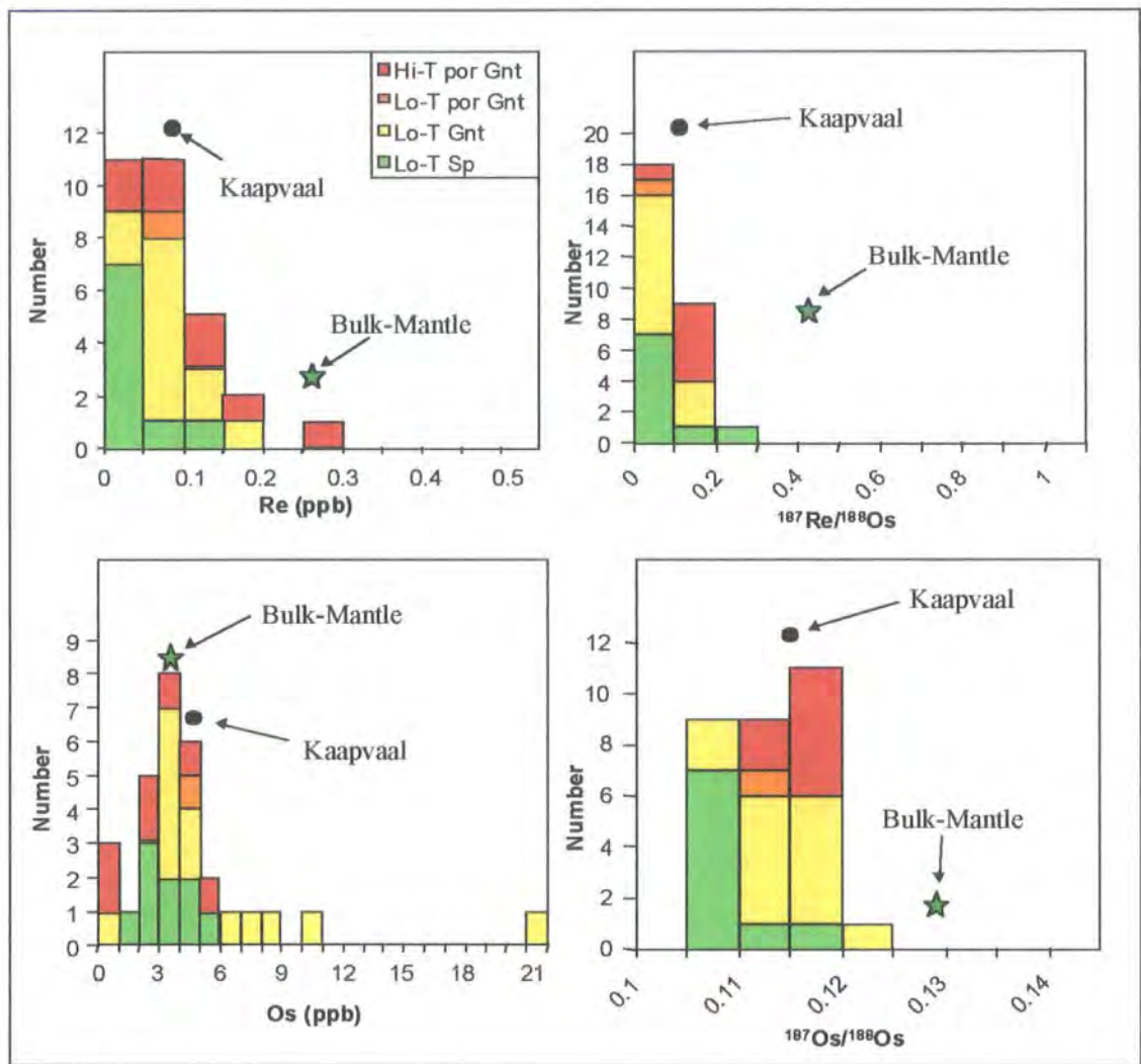
Figure 4.15 Histograms of Re and Os concentration (ng/g or ppb), ^{187}\text{Re}/^{188}\text{Os} and ^{187}\text{Os}/^{188}\text{Os} for Jericho peridotite xenoliths. Mean Kaapvaal values after Carlson et al. (1999) and Bulk-Mantle after Morgan (1986).
