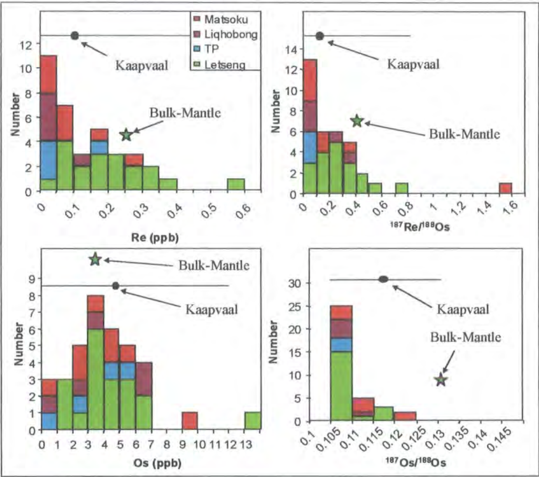
Figure 3.24 Histograms of Re and Os concentration (ng/g or ppb), ^{187}\text{Re}/^{188}\text{Os} and ^{187}\text{Os}/^{188}\text{Os} for low-T Lesotho peridotite xenoliths. Mean Kaapvaal values and range after Carlson et al (1999) and Bulk-Mantle after Morgan (1986).
