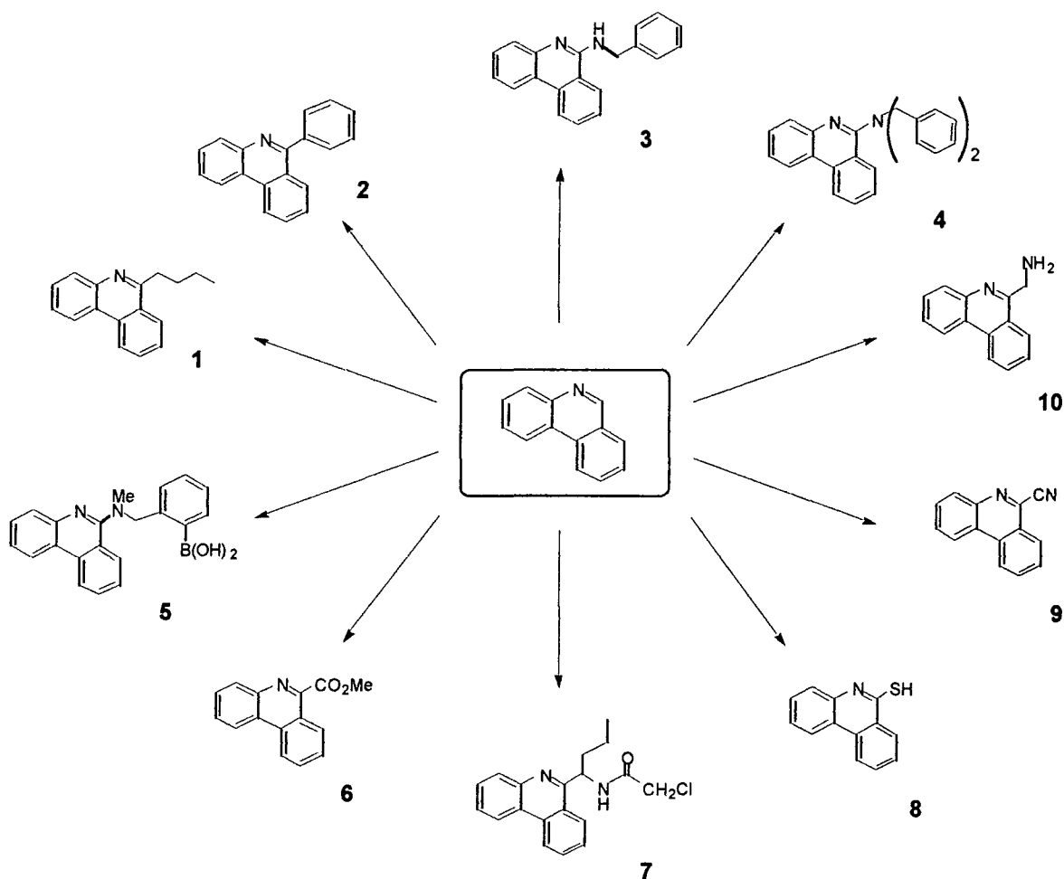
Scheme 2.6: 6-Substituted phenanthridines
