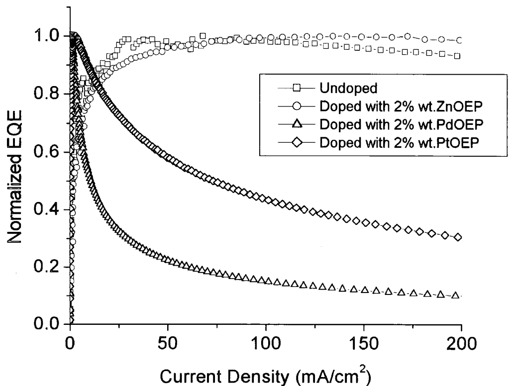
Figure 7-14 Normalized EQE-Current Plots for representative Devices: Undoped PF2/6am4 with 2% wt. ZnOEP, PdOEP and PtOEP doped PF2/6am4 doped PF2/6am4. For absolute EQE values refer to Table 7-2. The purpose of normalizing the curves is to compare the curve shapes and the positions of the peaks for different dopant species
