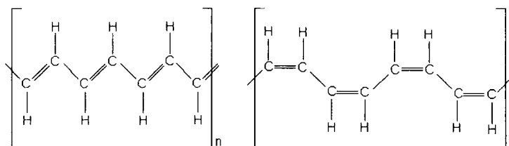
Figure 2-4 Chemical Structure of poly(acetylene). cis - (CH)_n (left) and trans - (CH)_n (right)
