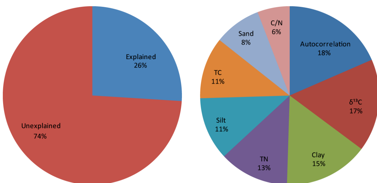
Figure 6.6: Pie charts showing the total variation in the fossil dataset divided into (a) explained and unexplained sectors and (b) sectors representing the individual environmental variables and interactions between variables contributing to the total explained variance.
