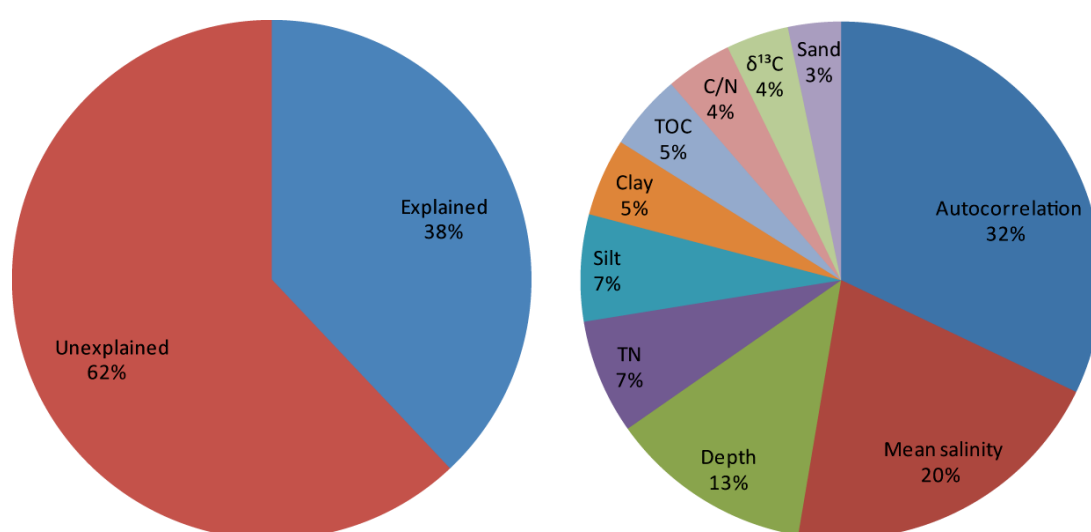
Figure 5.9: Pie charts showing the total variation in the contemporary fauna divided into (a) explained and unexplained sectors and (b) the total explained variance divided into sectors representing the individual environmental variables and interactions between variables.
