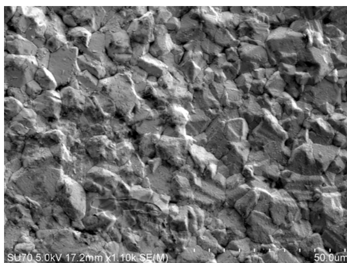
Figure 5.11: SEM image for a CdTe film grown at 200 Torr of N 2 as used in the “Bevel 1” sequence. The grain size (up to ~ 10 \mu\text{m} ) is relatively large and is associated with high roughness.
