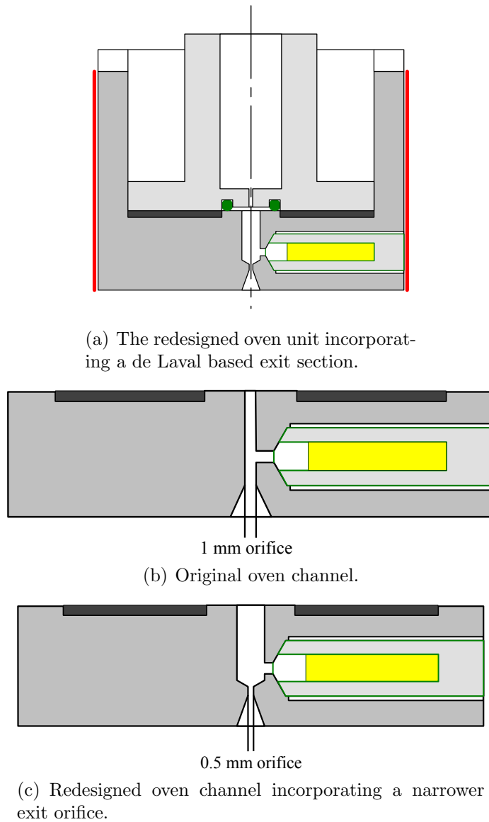
Figure 2.9: Comparison between exit channels of the two different oven designs.
