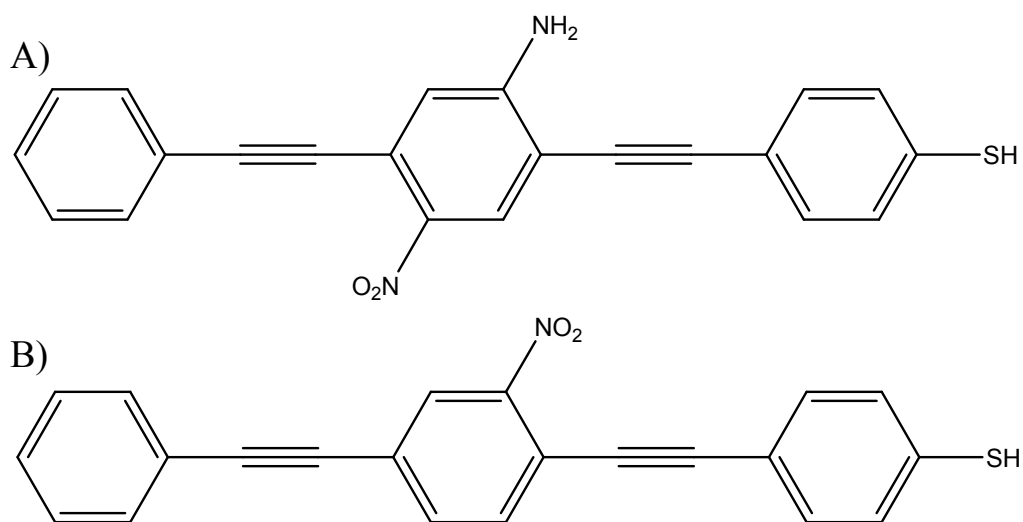
Figure 1.6: A) 2-amino-4,4-di(ethynylphenyl)-5-nitro-1-benzenethiol and B) 4,4-di(ethynylphenyl)-2-nitro-1-benzenethiol. Both derivatives of BPEB display negative differential resistance when placed between gold electrodes.
