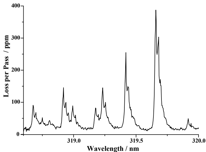
(a) Performance of original oven design.
