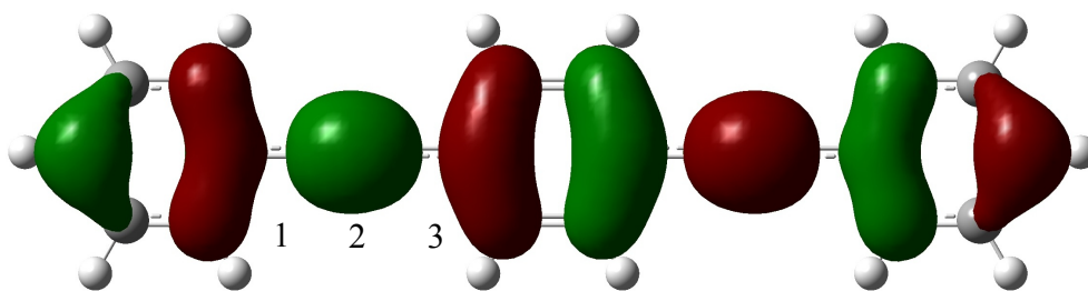
Figure 1.8: Planar geometry adopted by 1,4-bis(phenylethynyl)benzene displaying the HOMO orbital. Points 1 and 3 show orbital nodes between the alkyne triple bond and the benzene rings.
