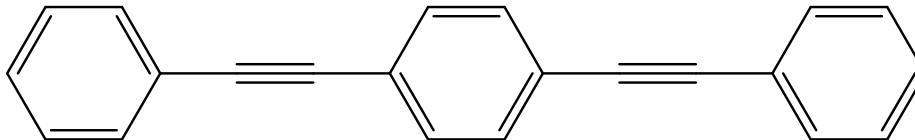
Figure 1.5: 1,4-bis(phenylethynyl)benzene.
