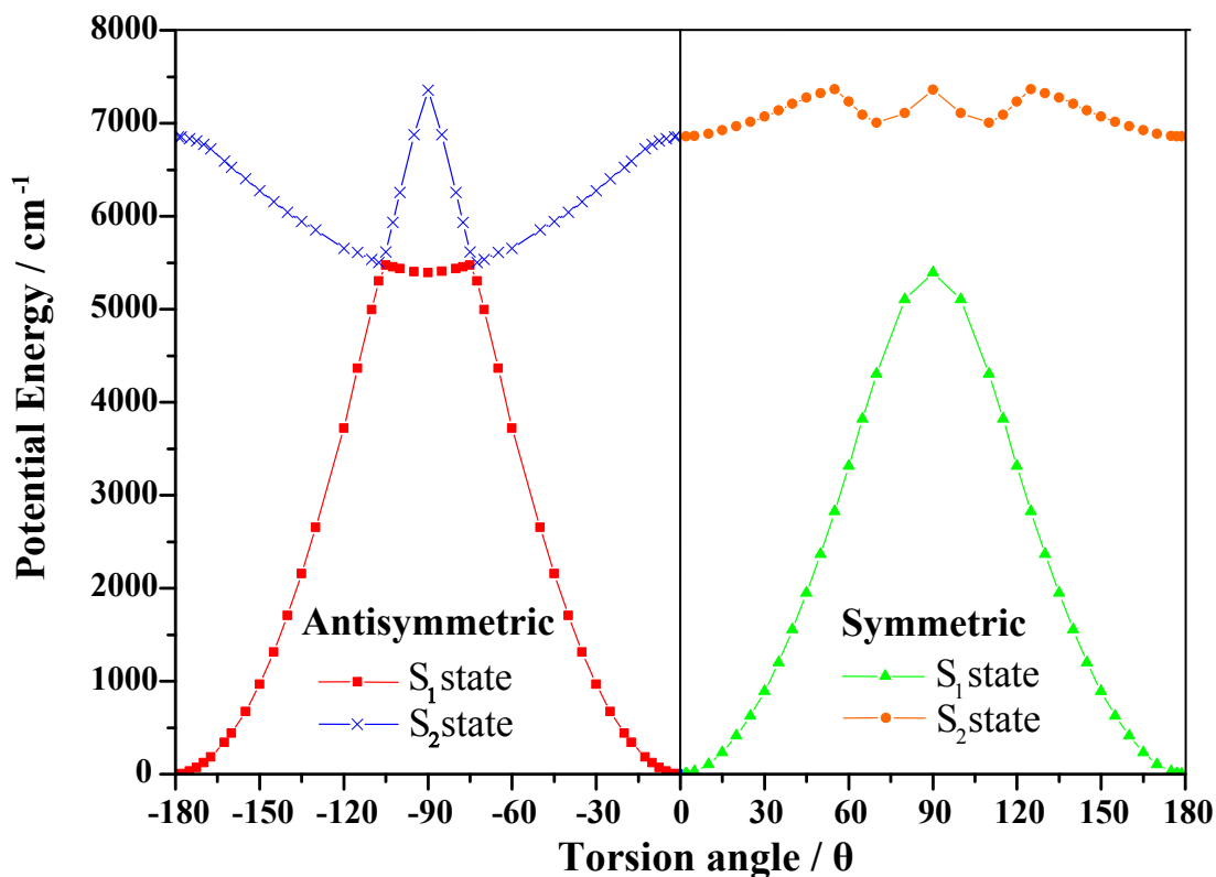
Figure 4.9: The first two singlet excited states of the BPET molecule as calculated using the optimised ground state geometries. Both the symmetric and antisymmetric torsion motions are shown.
