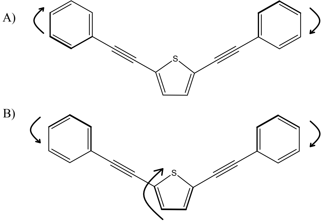
Figure 4.6: The A) Antisymmetric and B) Symmetric torsional motions of the BPET molecule.
