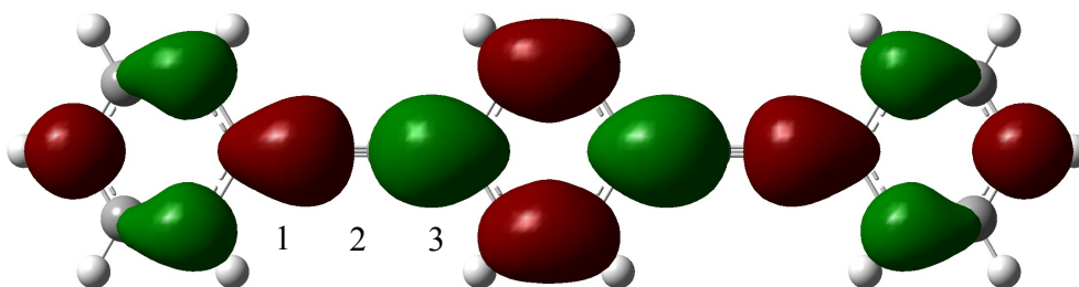
Figure 1.9: Planar geometry of 1,4-bis(phenylethynyl)benzene LUMO. Shown is the change in orbital distribution, whereby point 2 displays a node and points 1 and 3 now exist as bonds between the benzene ring and alkyne carbons.
