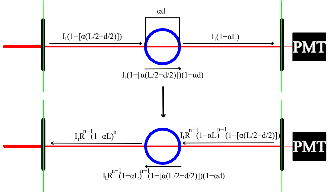
Figure 3.11: The intensity of the laser pulse entering the cavity is I_L , R and T = 1 - R are the mirror reflectivity and transmission, respectively, L is the length of the sample inside the cavity, d the length of the LIF probe volume and \alpha the molecular absorption coefficient.
