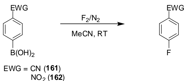
Scheme 84: Fluoro-deboronation of 4-cyanophenylboronic acid using elemental fluorine
