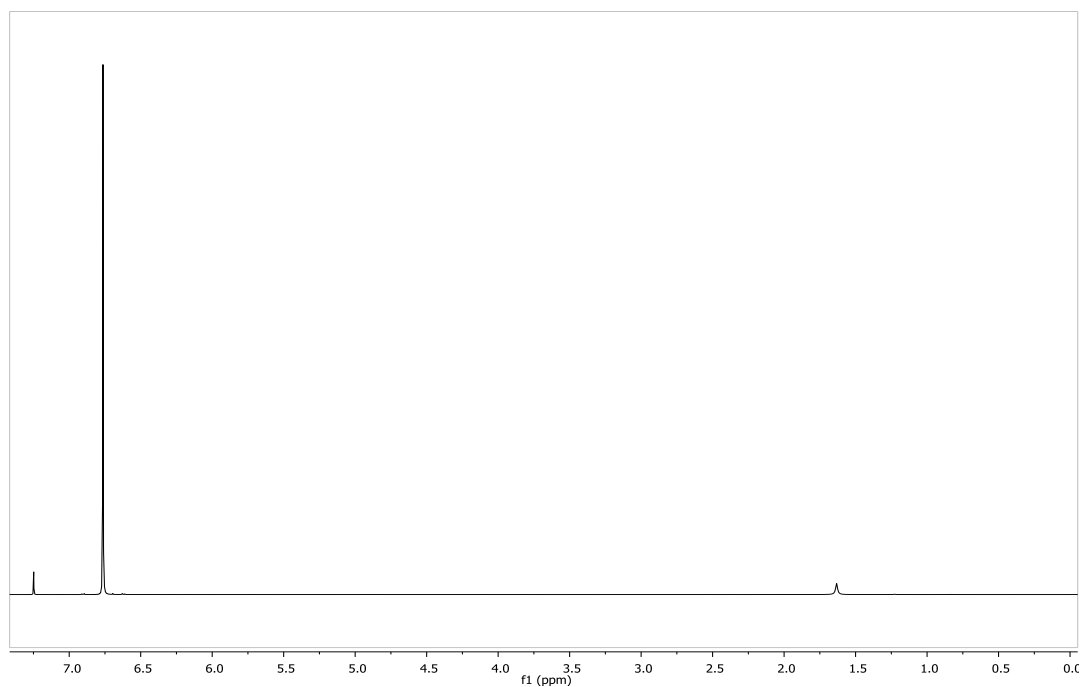
Figure 11: ^1\text{H} NMR Spectrum of 78 from fluorination of 1,4-diethoxybenzene
