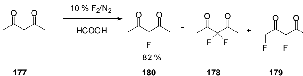
Scheme 104: Fluorination of pentane-2,4-dione using fluorine
