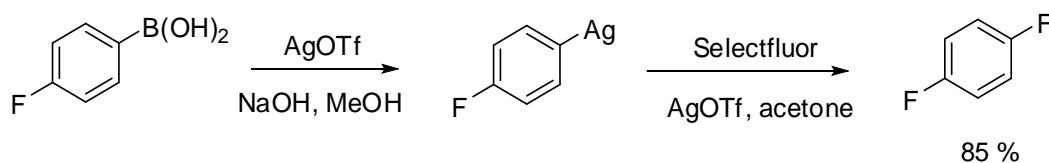
Scheme 25: Fluorination of boronic acids using silver salts and Selectfluor TM
