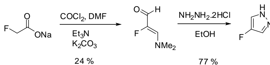
Scheme 95: Synthesis of 4-fluoropyrazole
