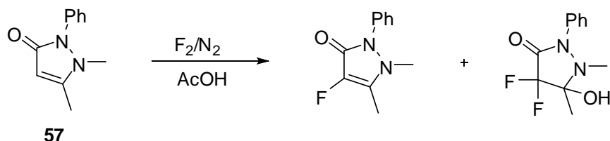
Scheme 15: Direct fluorination of antipyrine
