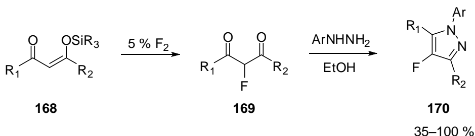
Scheme 92: Synthesis of 4-fluoropyrazoles
