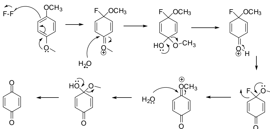
Scheme 42: Proposed mechanism of oxidation to the p -benzoquinone
