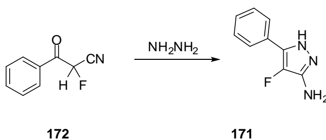
Scheme 93: Synthesis of 4-fluoroaminopyrazoles 96
