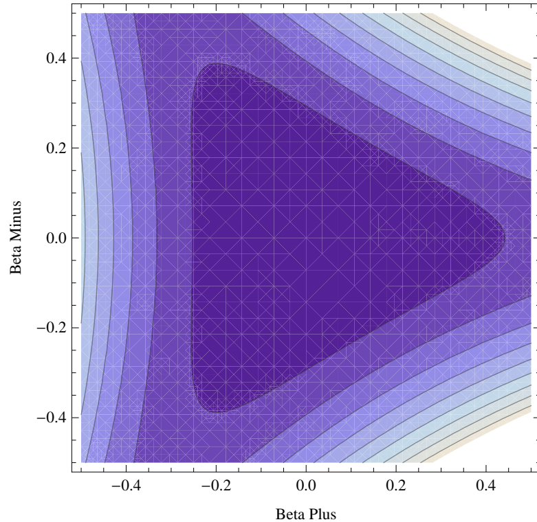
Figure 2.2: A contour plot showing the equipotential lines of the potential V(\beta_+, \beta_-) demonstrating the triangular symmetry of this potential.
