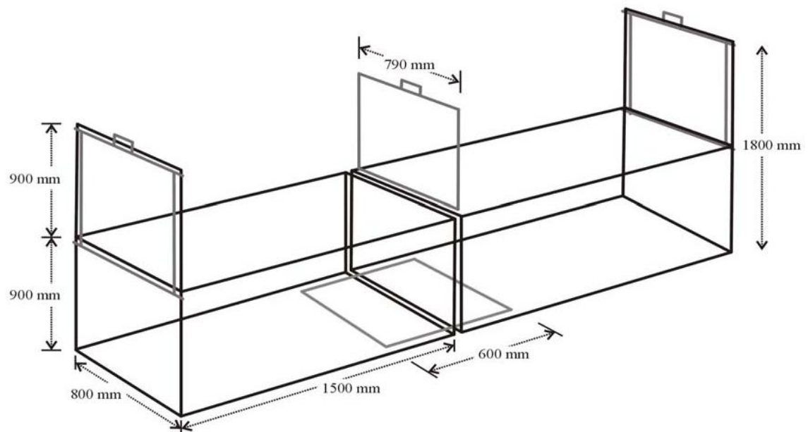
Figure 2.6 Design of double-door box traps constructed to capture cheetahs in Savé Valley Conservancy (Marker, 2002).
