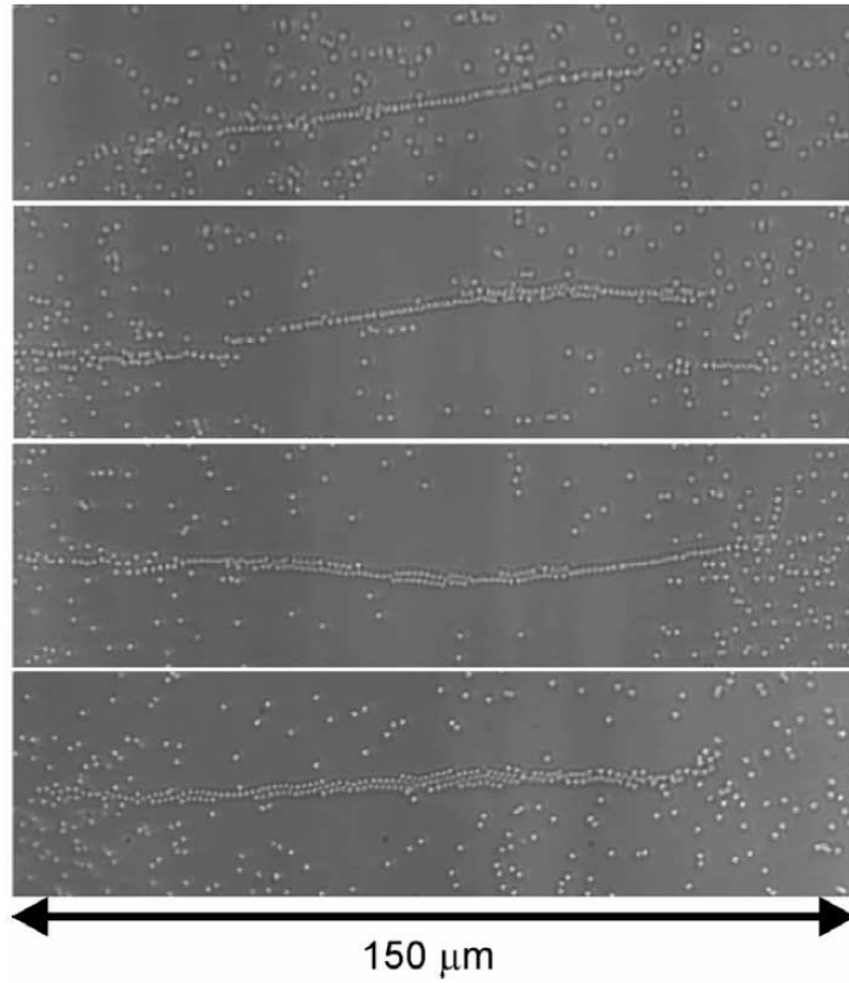
Figure 1.11: Chain-like structures of 1\ \mu\text{m} silica formed for different input powers (corresponding peak intensity on the surface is given in brackets): (i) 100\ \text{mW} ( 0.34\ \text{mW}\ \mu\text{m}^{-2} ); (ii) 175\ \text{mW} ( 0.68\ \text{mW}\ \mu\text{m}^{-2} ); (iii) 219\ \text{mW} ( 0.94\ \text{mW}\ \mu\text{m}^{-2} ); (iv) 266\ \text{mW} ( 1.02\ \text{mW}\ \mu\text{m}^{-2} ). 49
