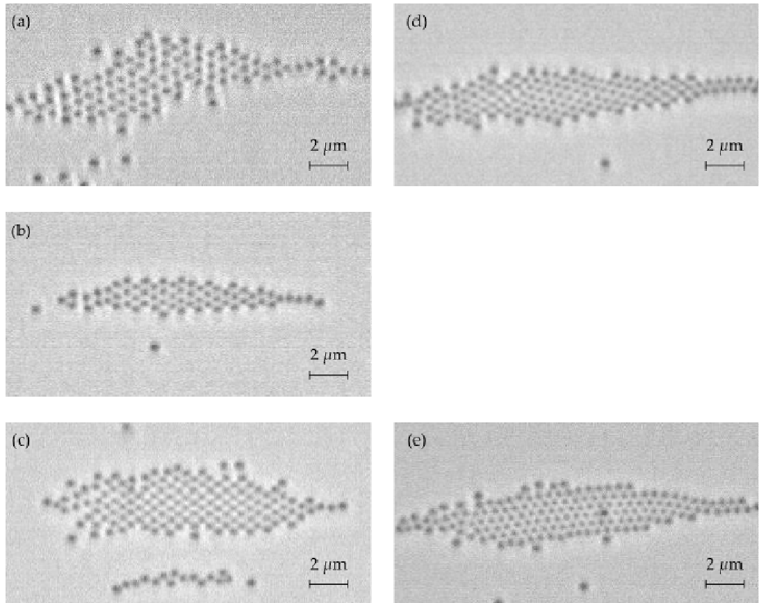
Figure 5.1: Incoherently trapped arrays of 420 nm PS at: (a) \lambda=840 nm in p -pol, showing hex2 with unstable columns; (b) \lambda=865 nm in p -pol, showing stable hex-2; (c) \lambda=890 nm in p -pol, showing stable hex-2; (d) \lambda=840 nm in s -pol, showing tilted hex-2; and (e) \lambda=890 nm in s -pol, showing tilted hex-1. ( n_{BK7} = 1.507 ; \theta_c = 62.2^\circ ; \theta_i = 64.5^\circ )
