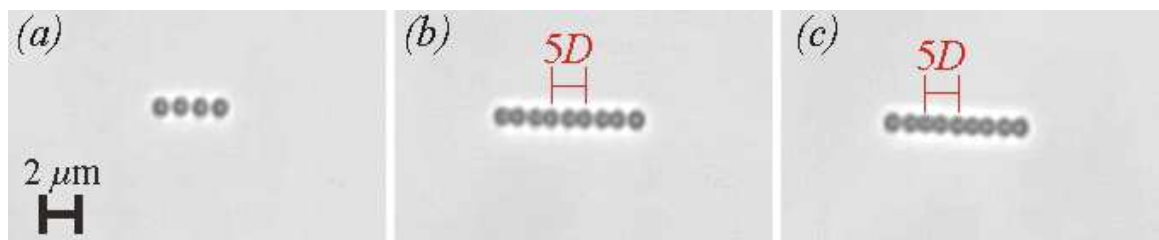
Figure 3.9: Lines of 800 nm PS particles showing (a) uniform spacings of 3D , which subsequently rearranges to (b) pairs, and (c) triplets ( n_{\text{SF10}}=1.702 ; \theta_i=56^\circ ; \lambda=1064 nm; s -pol; [\text{NaCl}] = 1 \mu\text{M} ).
